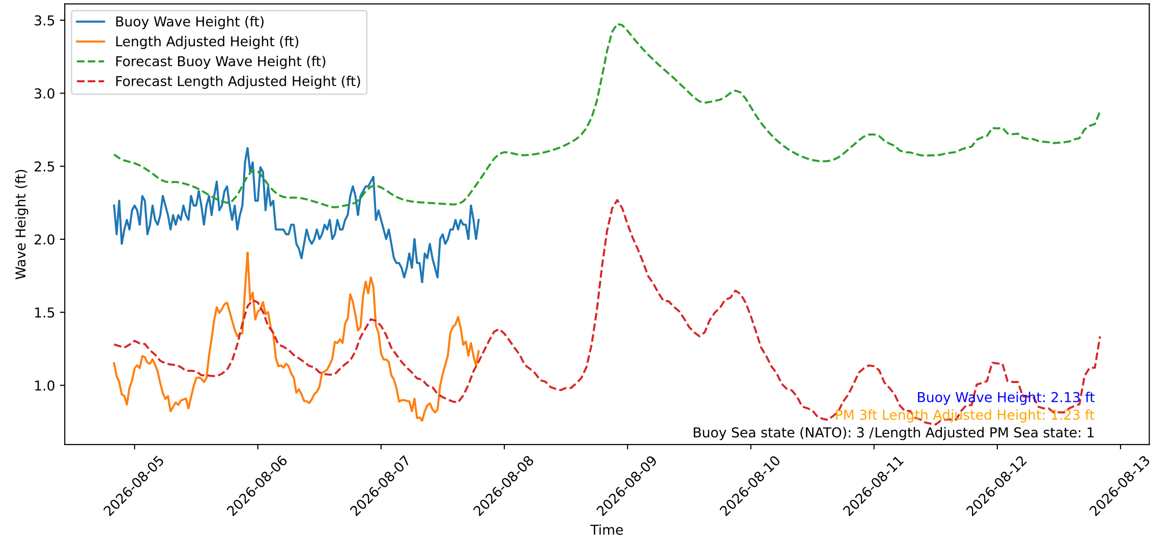
Wave Heights over Time for Green Beach at 2026-08-07 19:51:09
