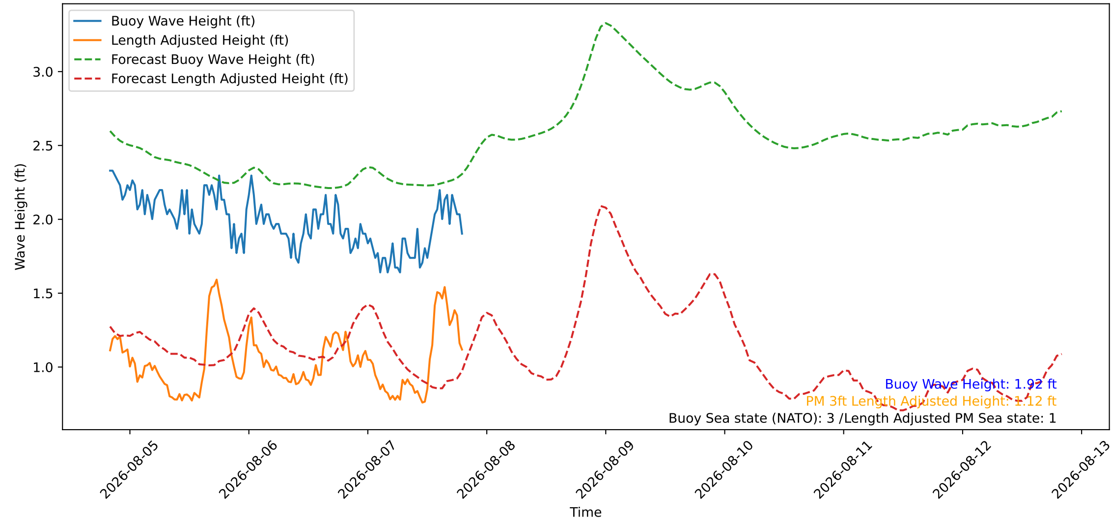
Wave Heights over Time for Oceanside Harbor at 2026-08-07 19:50:26
