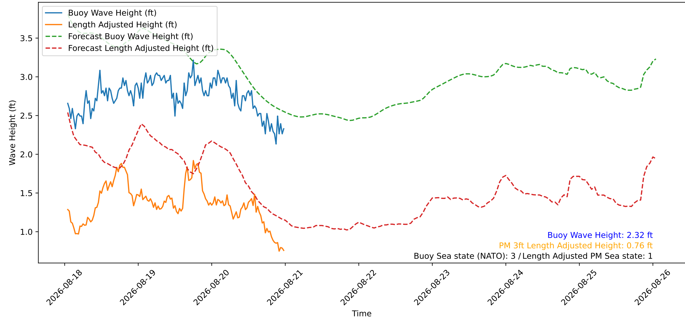
Wave Heights over Time for Red Beach at 2026-08-21 00:30:46
