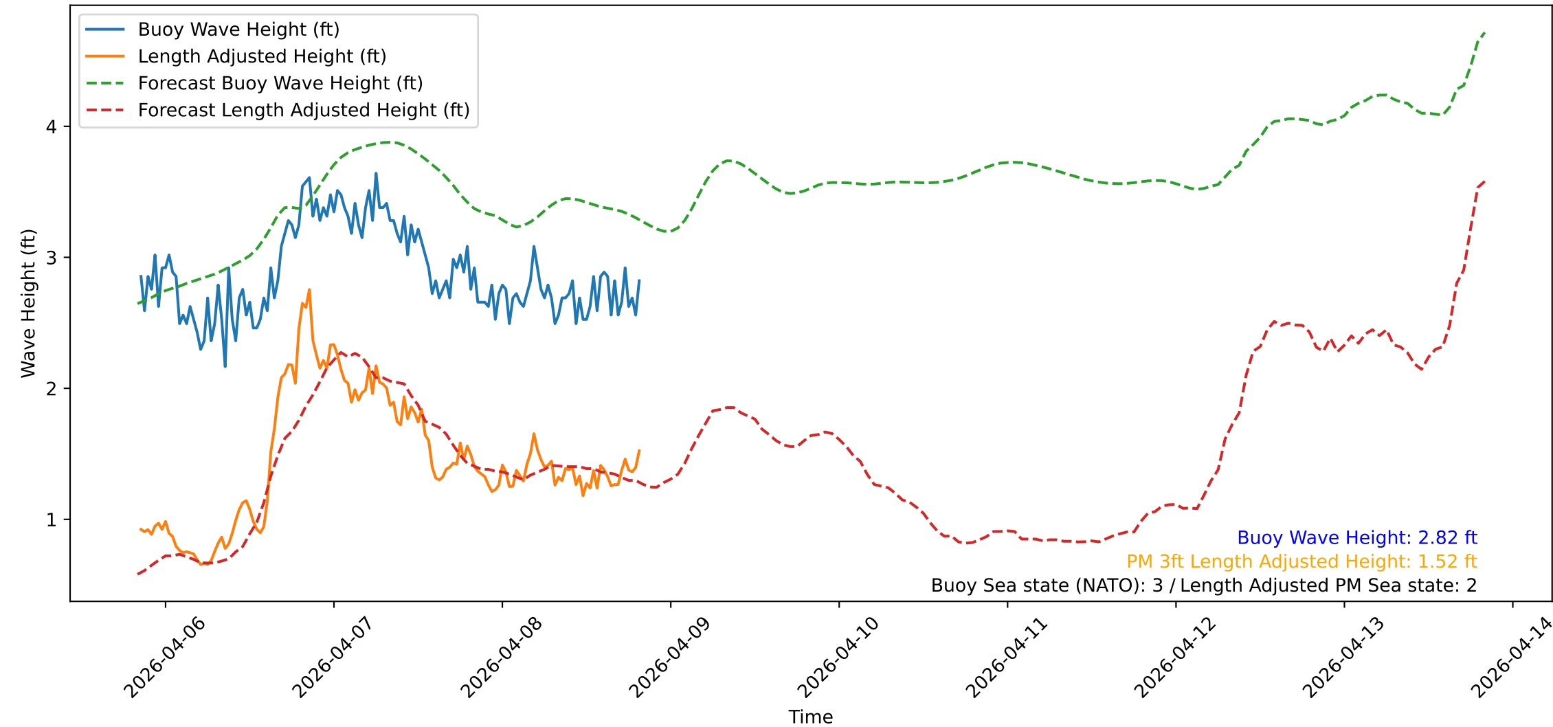
Wave Heights over Time for Oceanside Harbor at 2026-04-08 20:20:31
