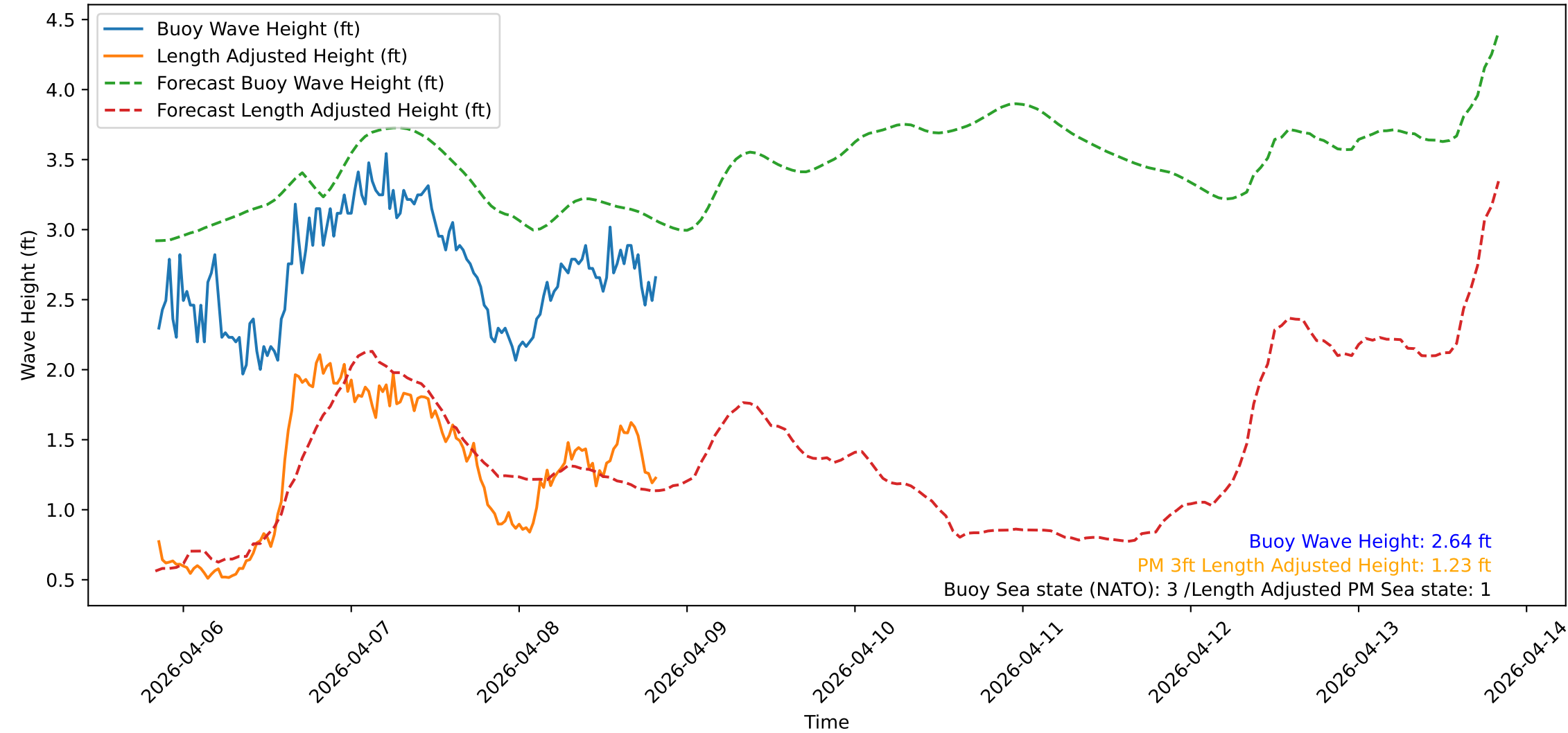
Wave Heights over Time for Red Beach at 2026-04-08 20:20:47
