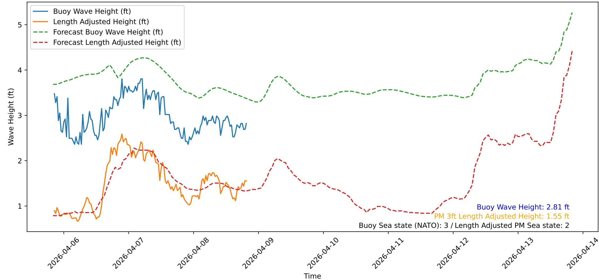
Wave Heights over Time for Green Beach at 2026-04-08 20:21:08
