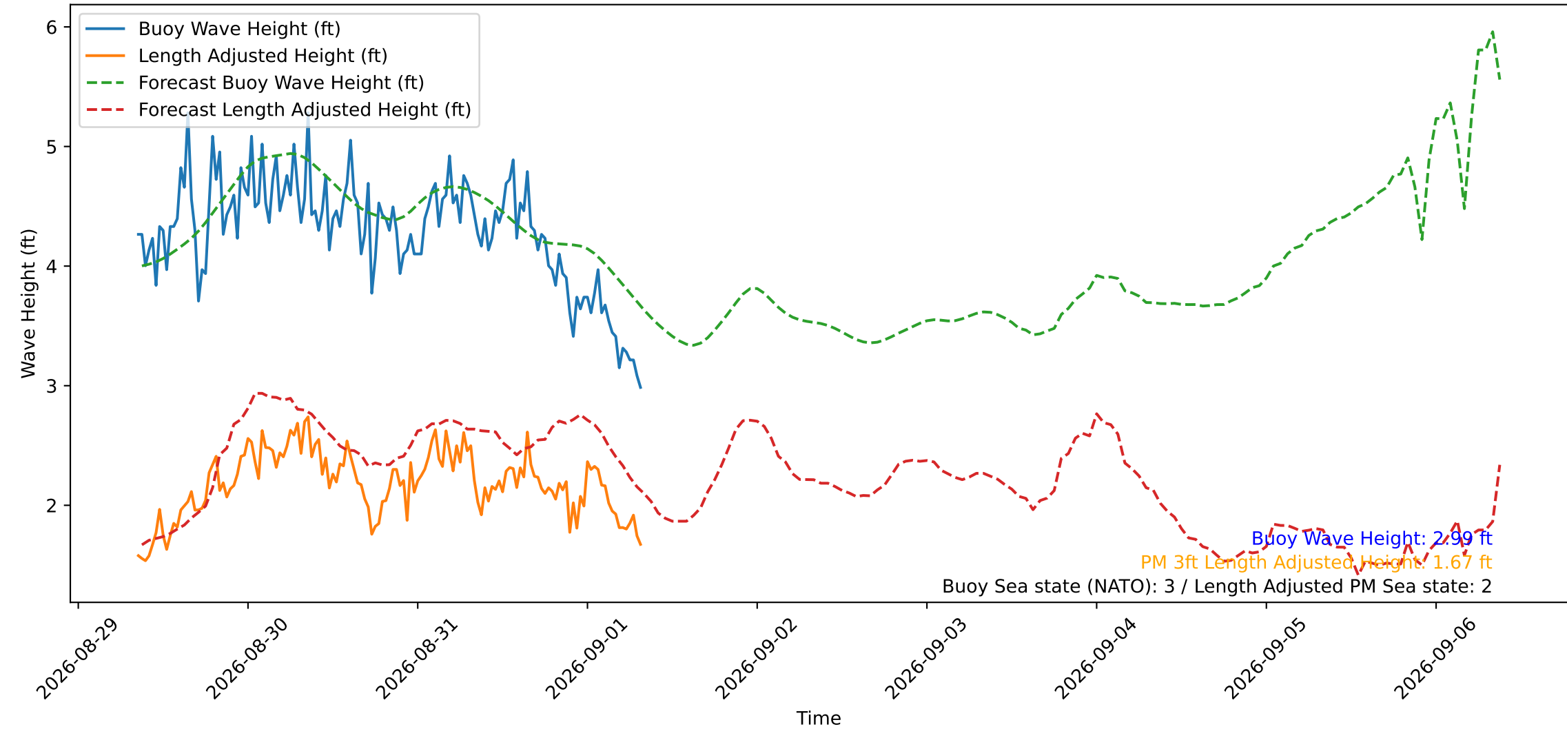
Wave Heights over Time for Oceanside Harbor at 2026-09-01 08:30:30
