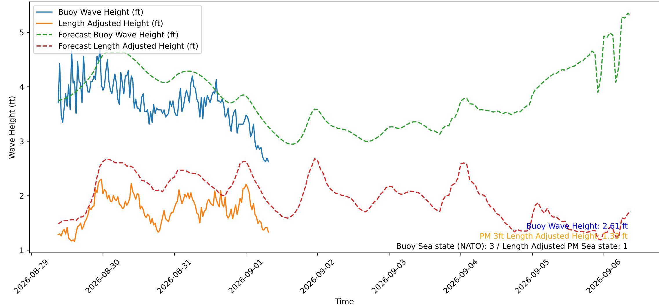
Wave Heights over Time for Red Beach at 2026-09-01 08:30:49
