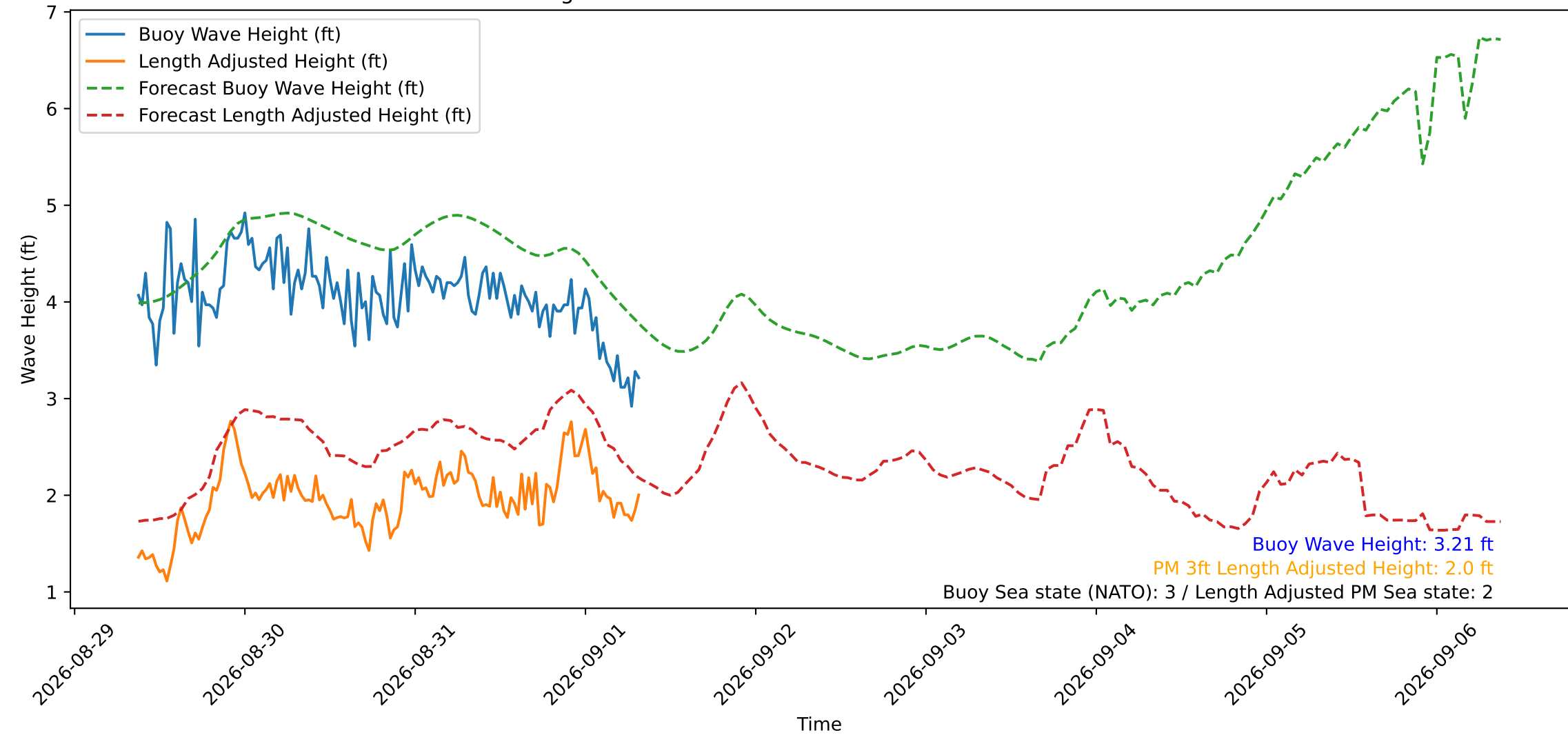
Wave Heights over Time for Green Beach at 2026-09-01 08:31:11
