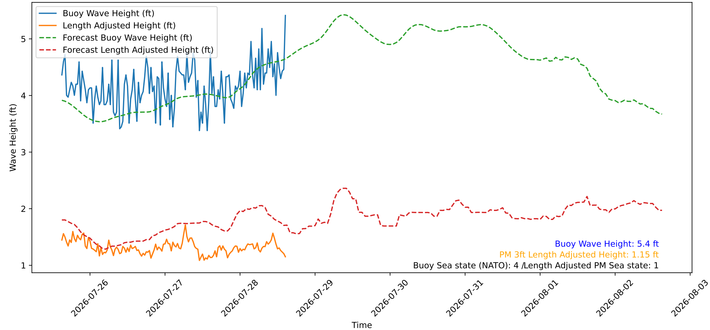
Wave Heights over Time for Green Beach at 2026-07-28 15:11:08
