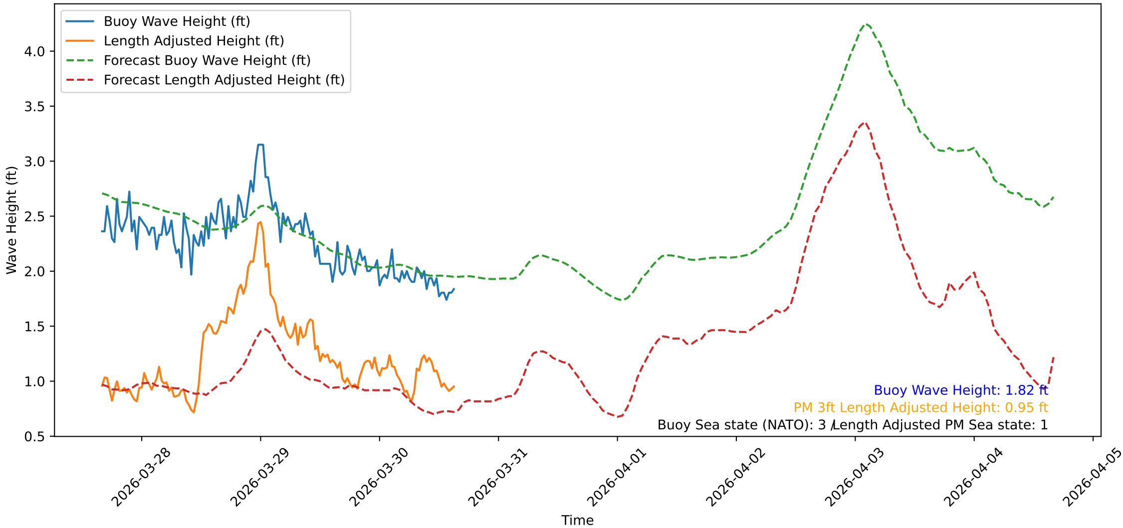
Wave Heights over Time for Oceanside Harbor at 2026-03-30 15:50:31
