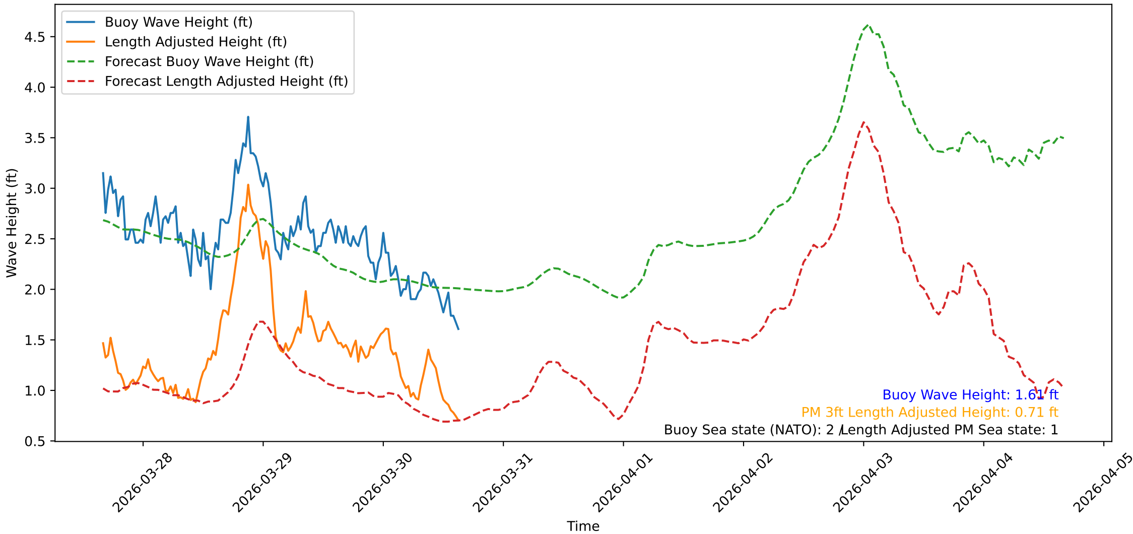
Wave Heights over Time for Green Beach at 2026-03-30 15:51:10
