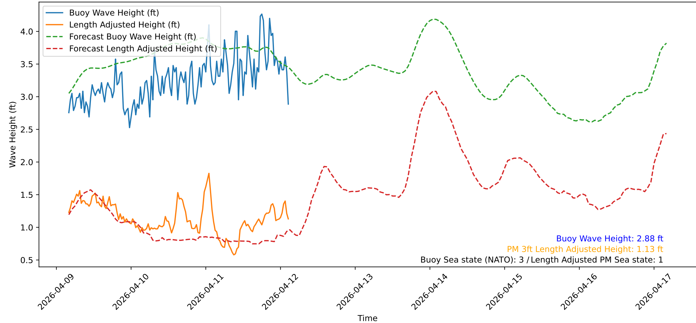
Wave Heights over Time for Red Beach at 2026-04-12 03:40:51
