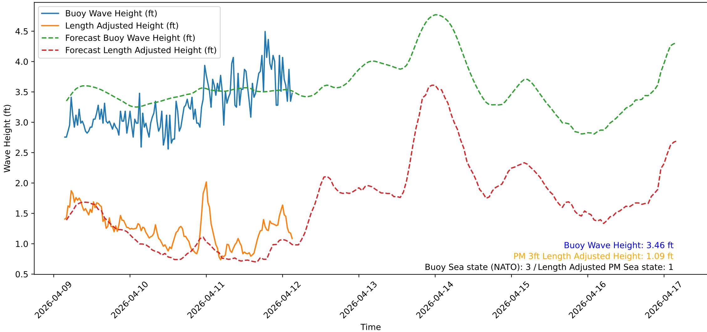
Wave Heights over Time for Green Beach at 2026-04-12 03:41:14
