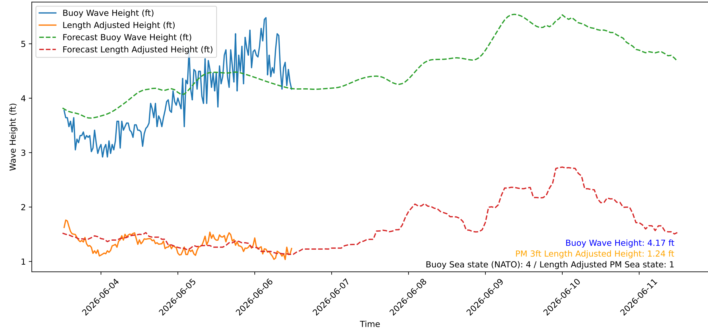
Wave Heights over Time for Oceanside Harbor at 2026-06-06 12:20:25
