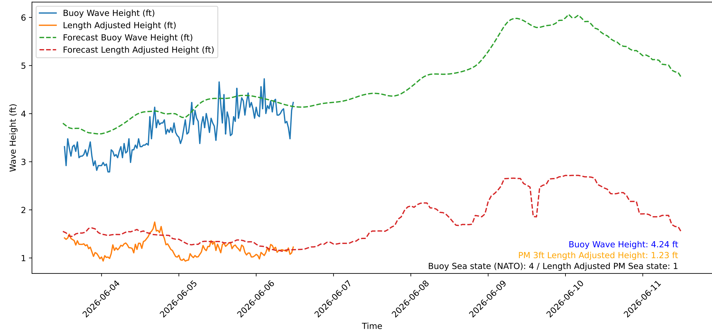
Wave Heights over Time for Green Beach at 2026-06-06 12:21:08
