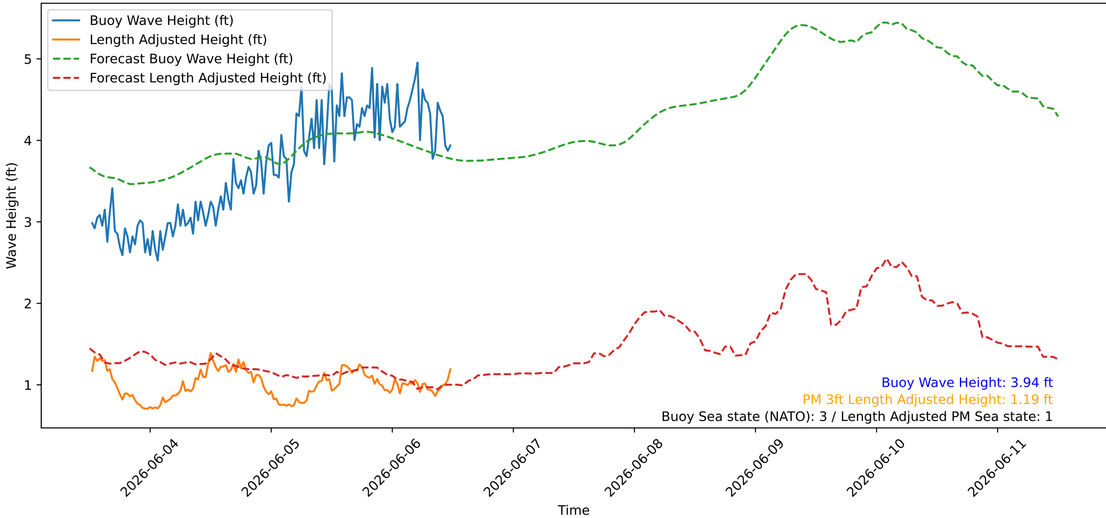
Wave Heights over Time for Red Beach at 2026-06-06 12:20:46
