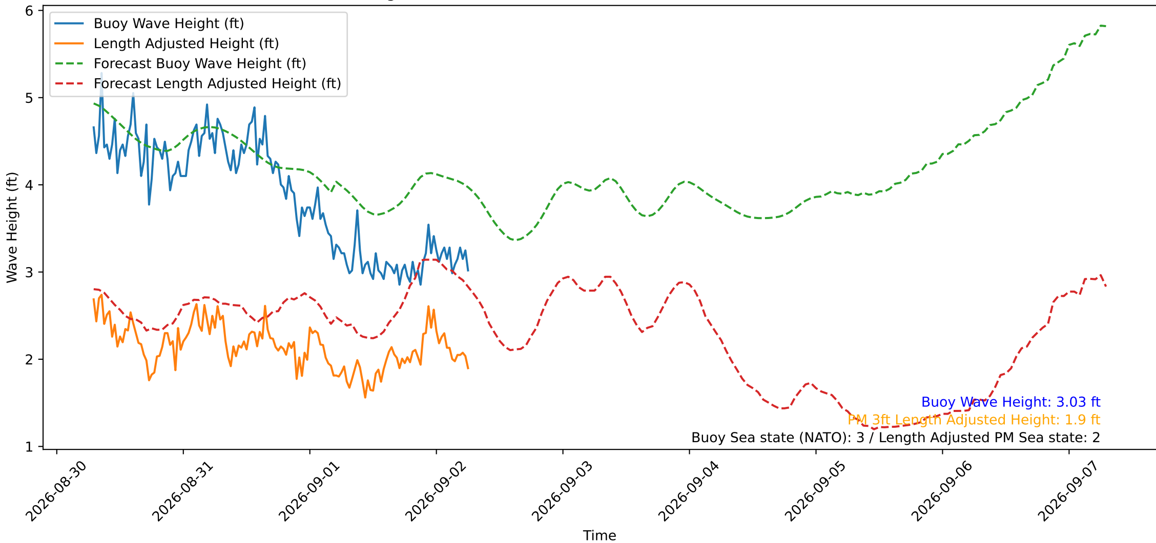
Wave Heights over Time for Oceanside Harbor at 2026-09-02 07:00:30
