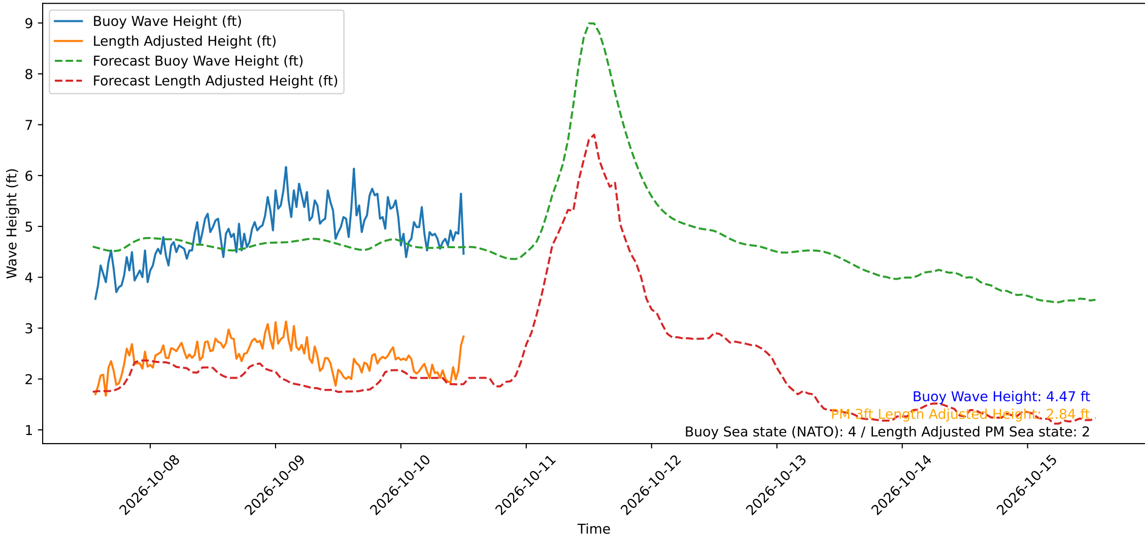
Wave Heights over Time for Green Beach at 2026-10-10 13:01:13
