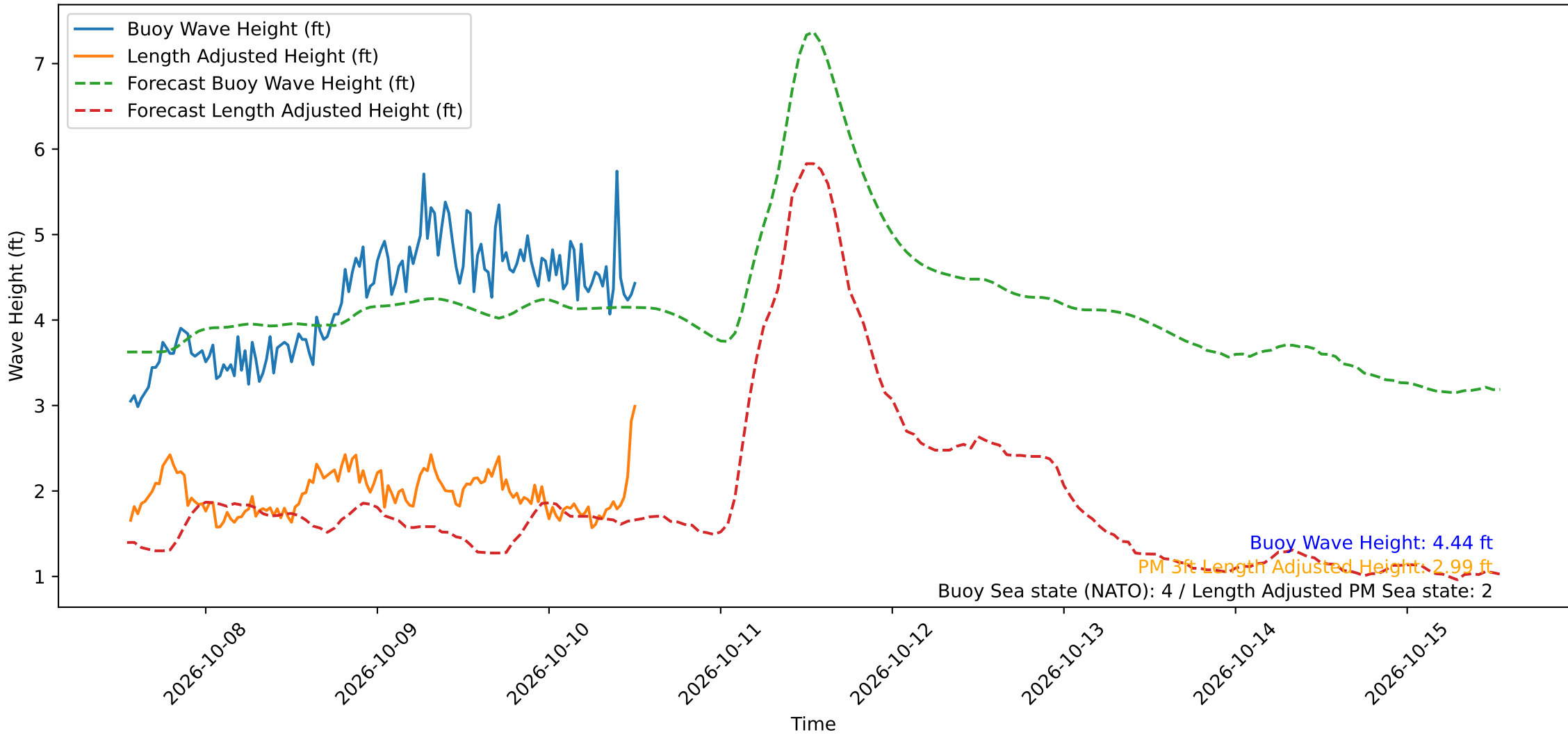
Wave Heights over Time for Red Beach at 2026-10-10 13:00:50
