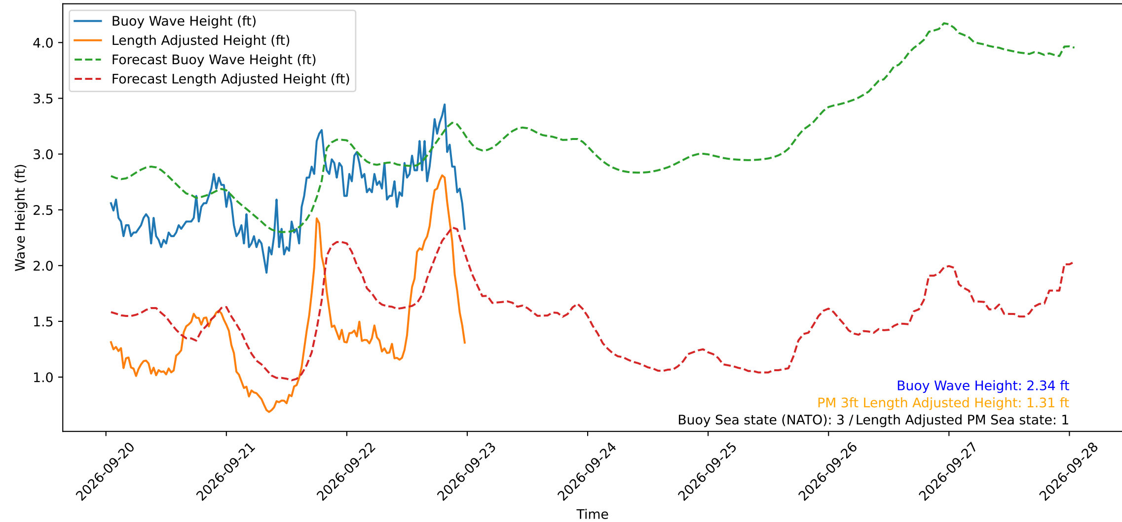
Wave Heights over Time for Green Beach at 2026-09-23 00:31:11
