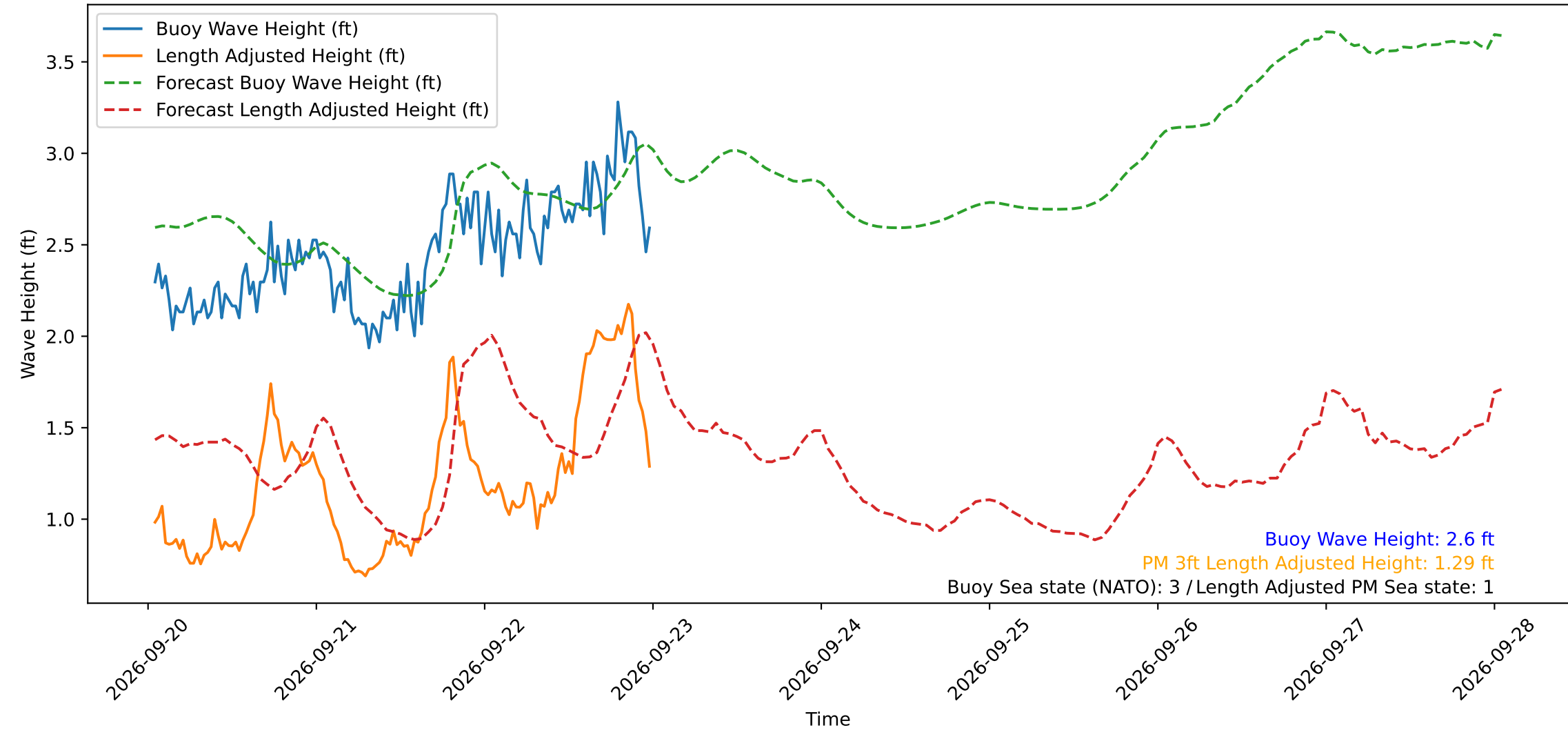
Wave Heights over Time for Red Beach at 2026-09-23 00:30:49
