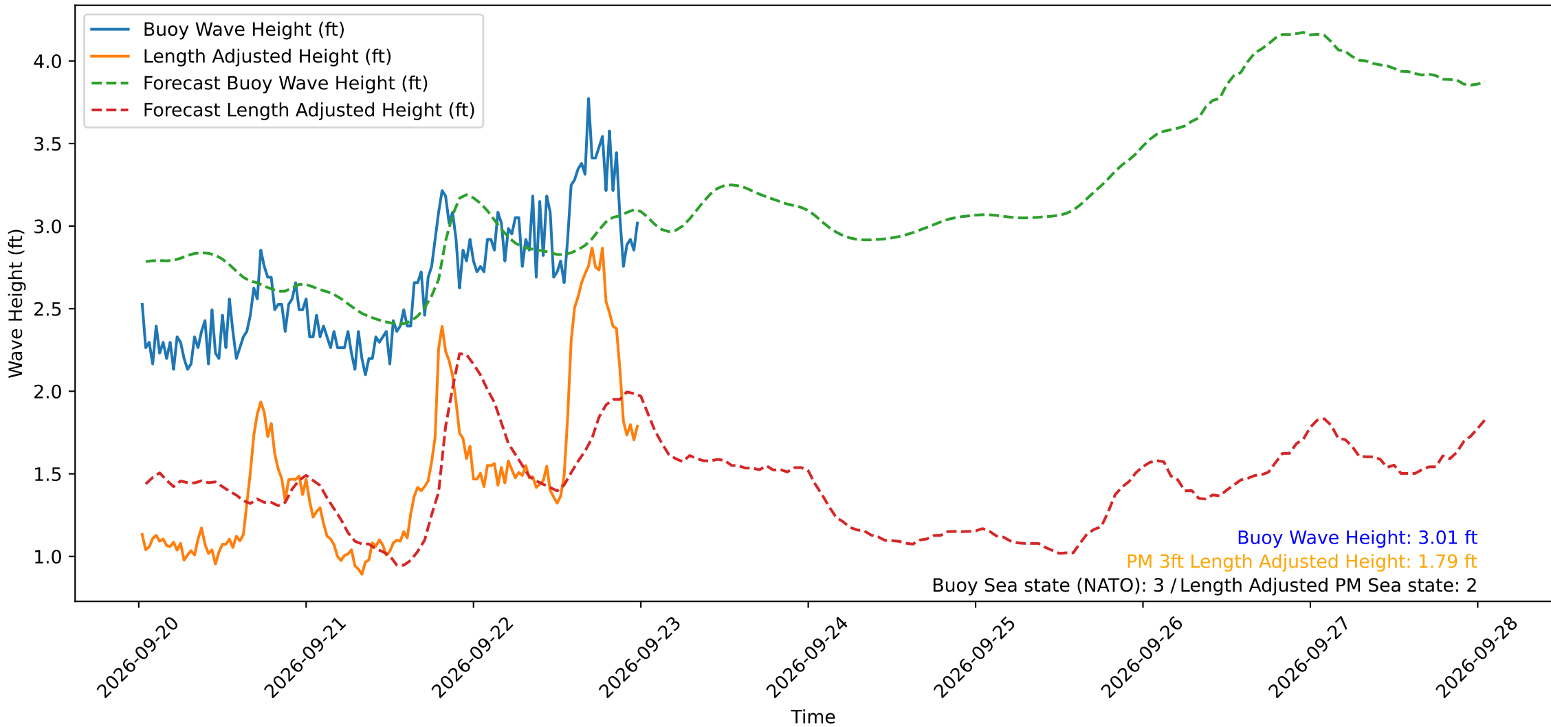
Wave Heights over Time for Oceanside Harbor at 2026-09-23 00:30:29
