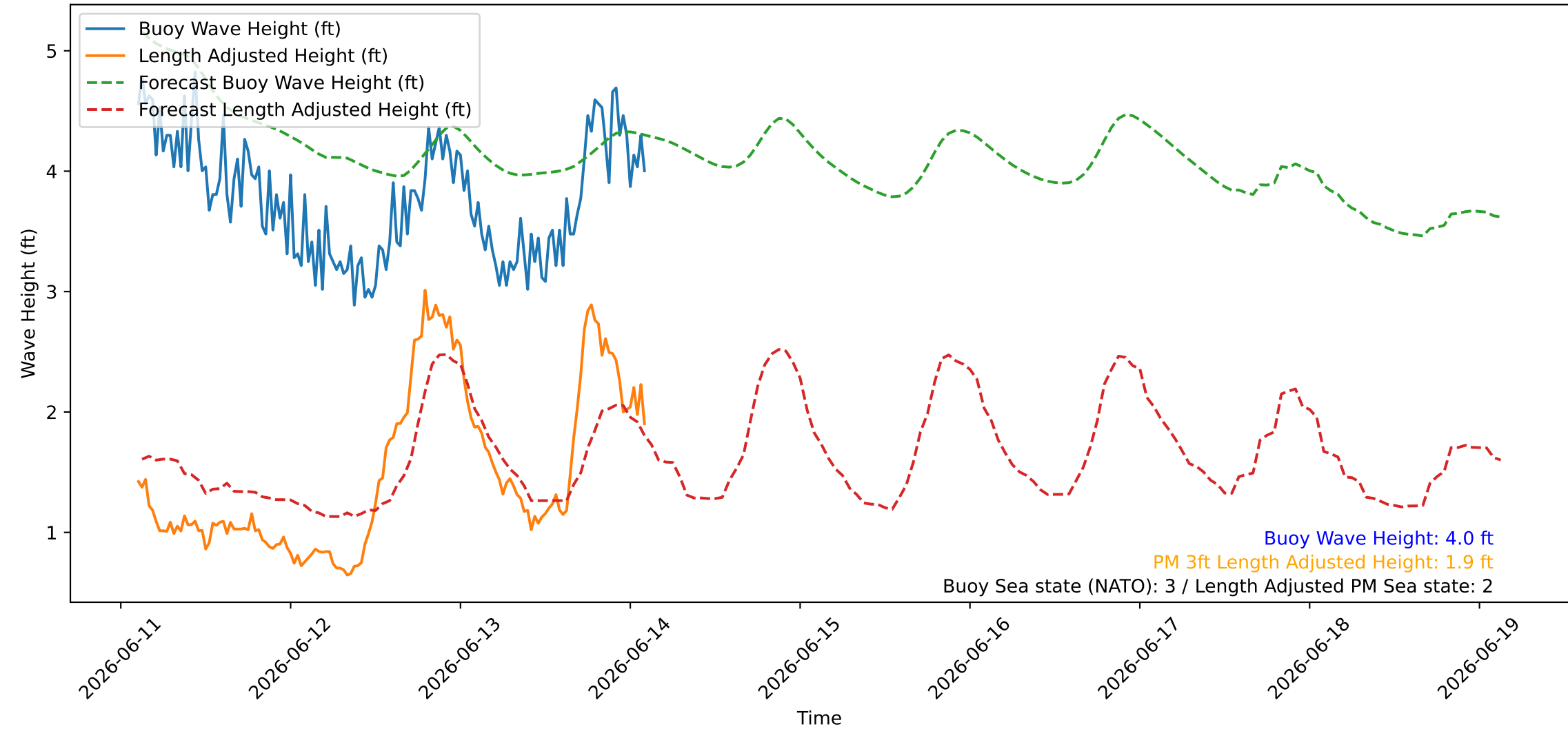
Wave Heights over Time for Green Beach at 2026-06-14 02:41:09
