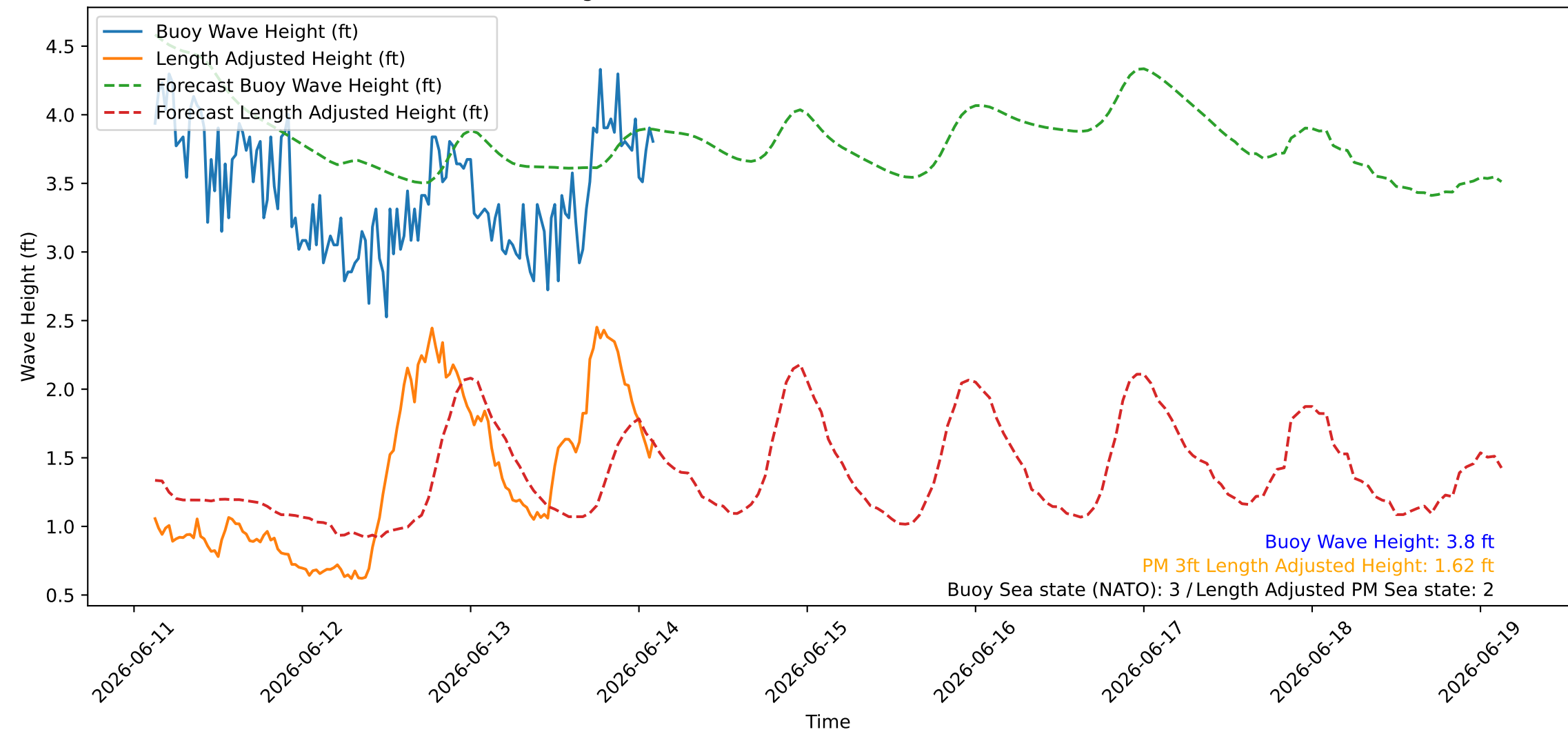
Wave Heights over Time for Red Beach at 2026-06-14 02:40:46
