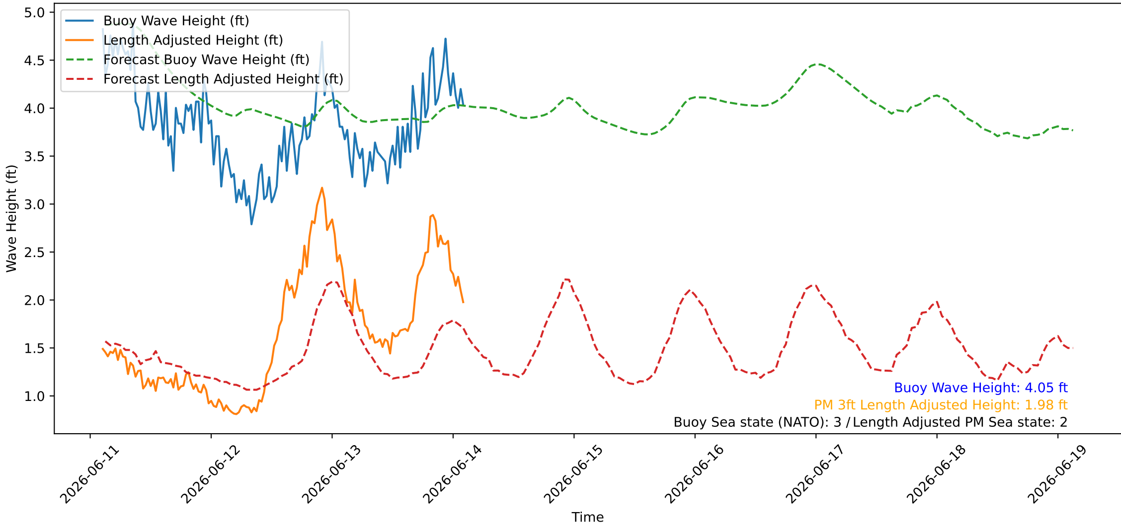
Wave Heights over Time for Oceanside Harbor at 2026-06-14 02:40:26
