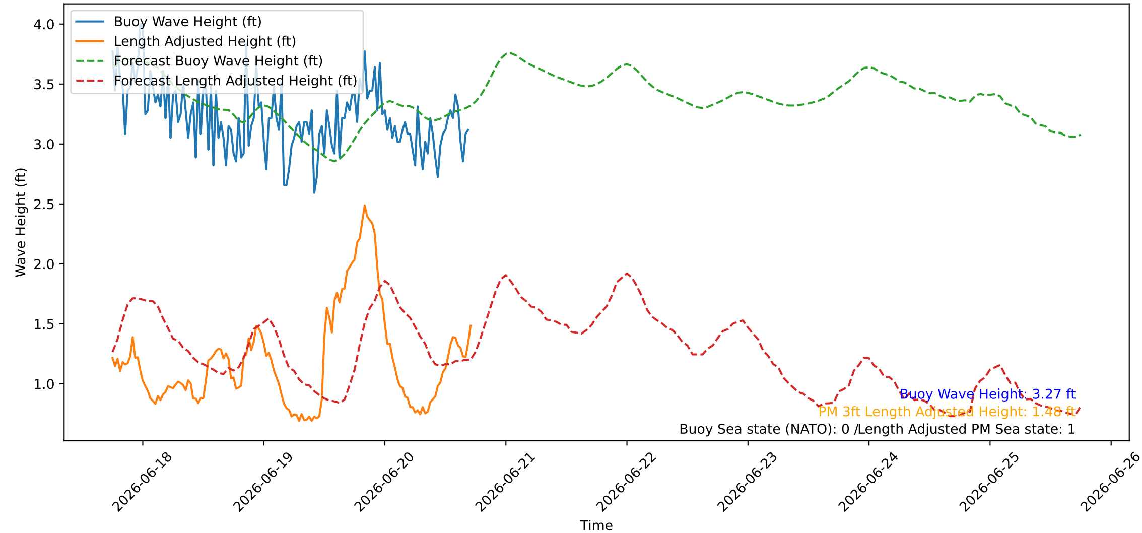
Wave Heights over Time for Red Beach at 2026-06-20 17:40:45
