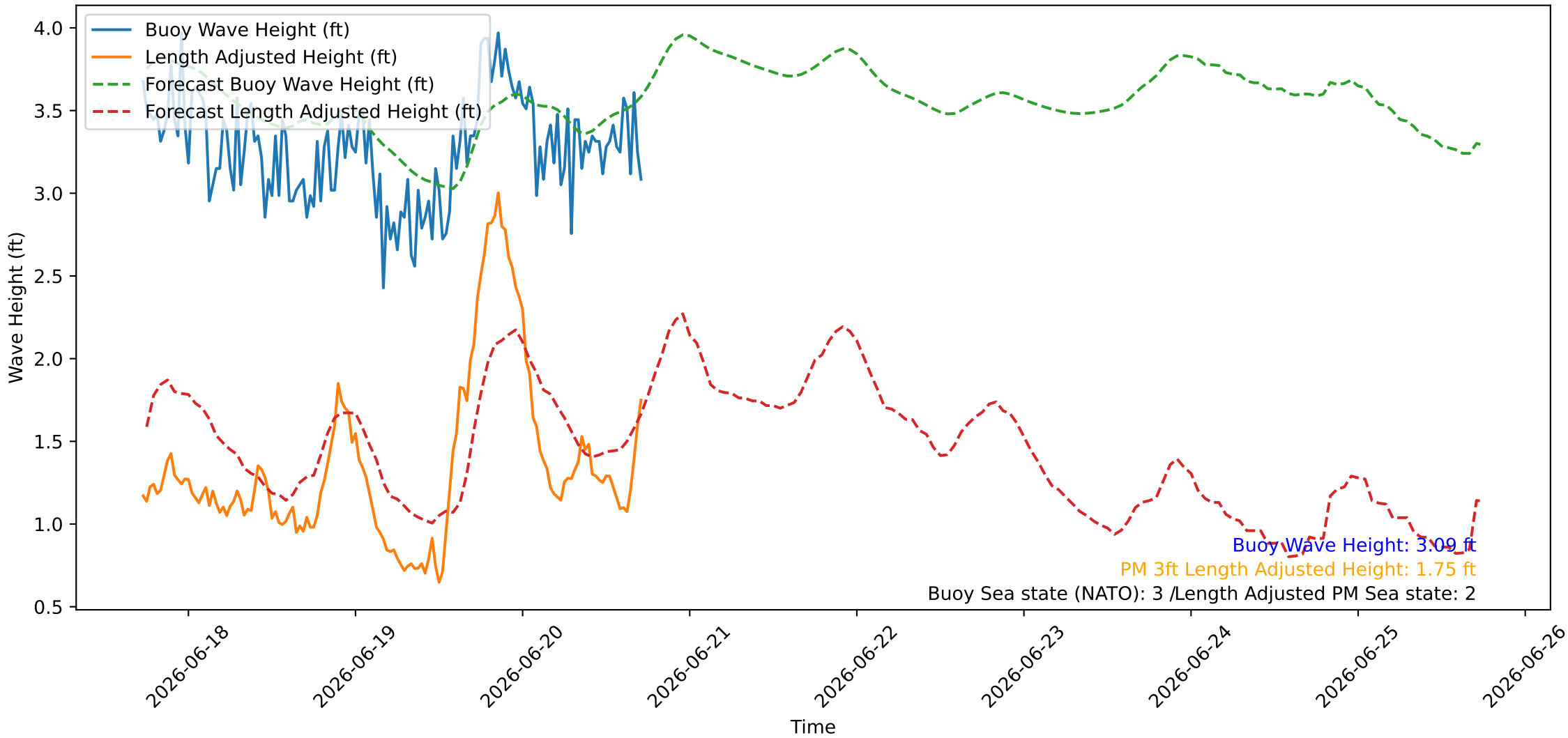
Wave Heights over Time for Green Beach at 2026-06-20 17:41:08
