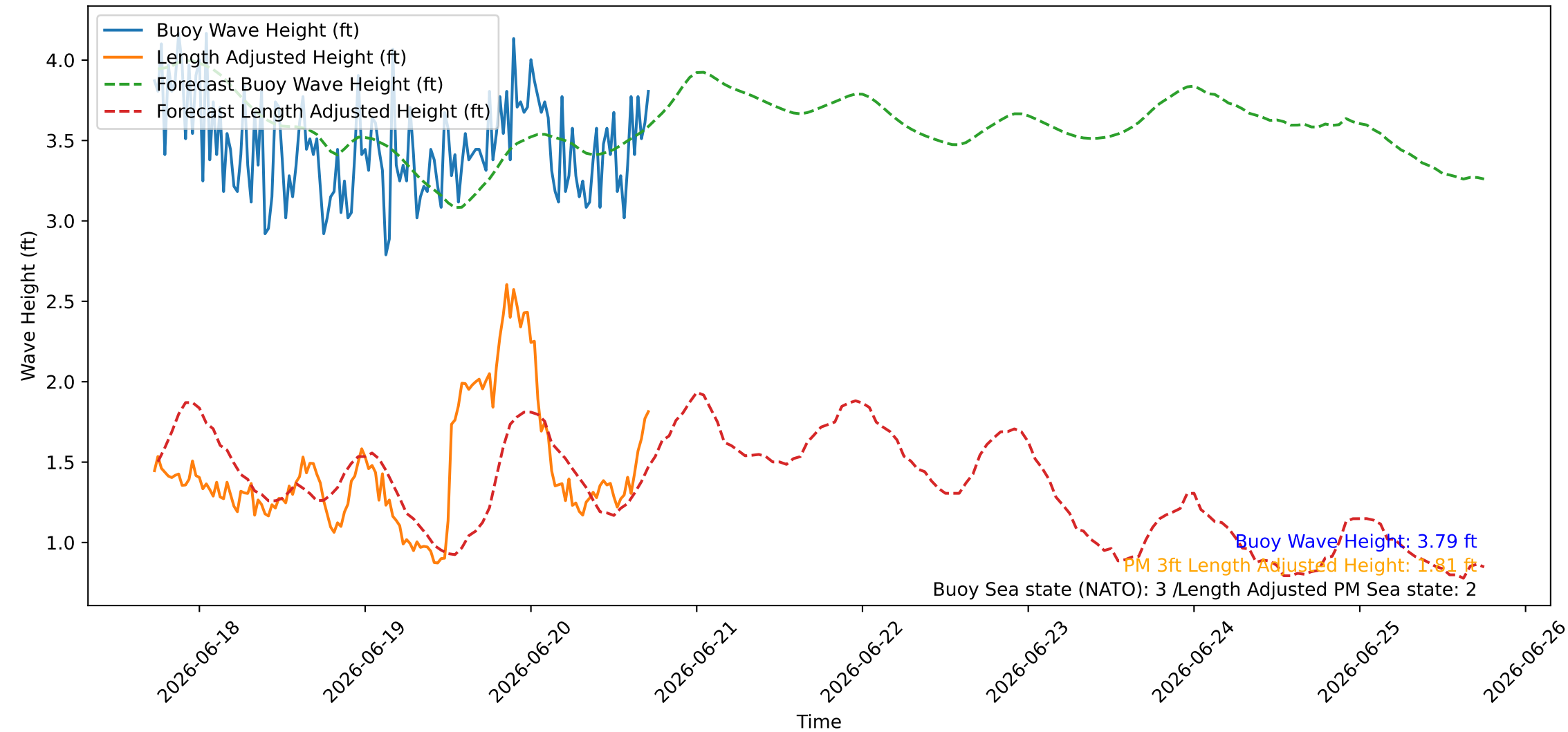
Wave Heights over Time for Oceanside Harbor at 2026-06-20 17:40:26
