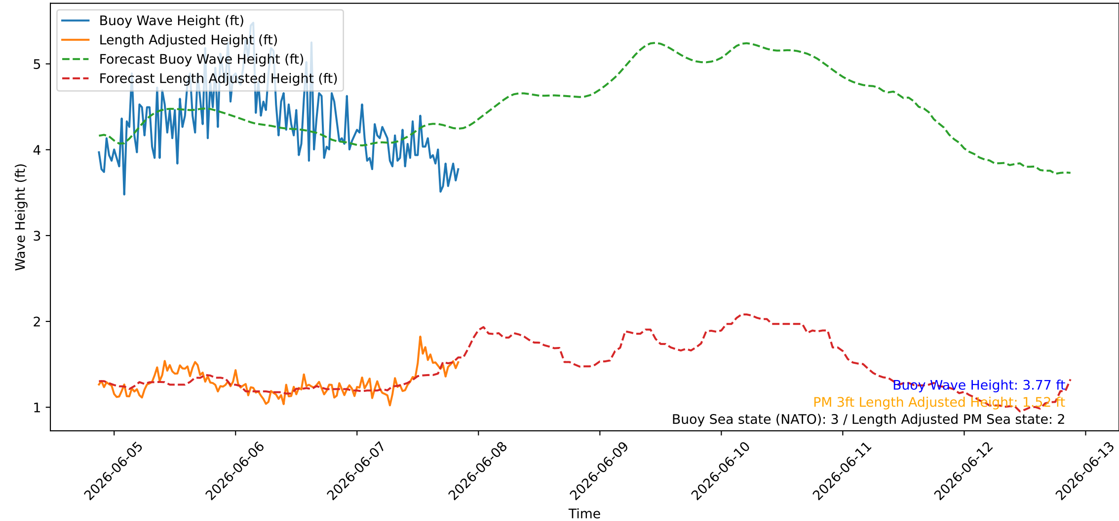
Wave Heights over Time for Oceanside Harbor at 2026-06-07 20:50:26
