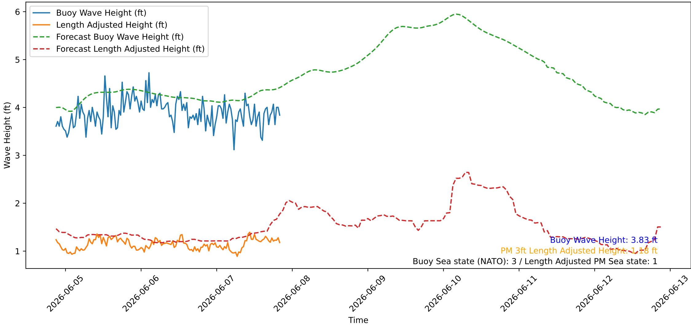
Wave Heights over Time for Green Beach at 2026-06-07 20:51:08
