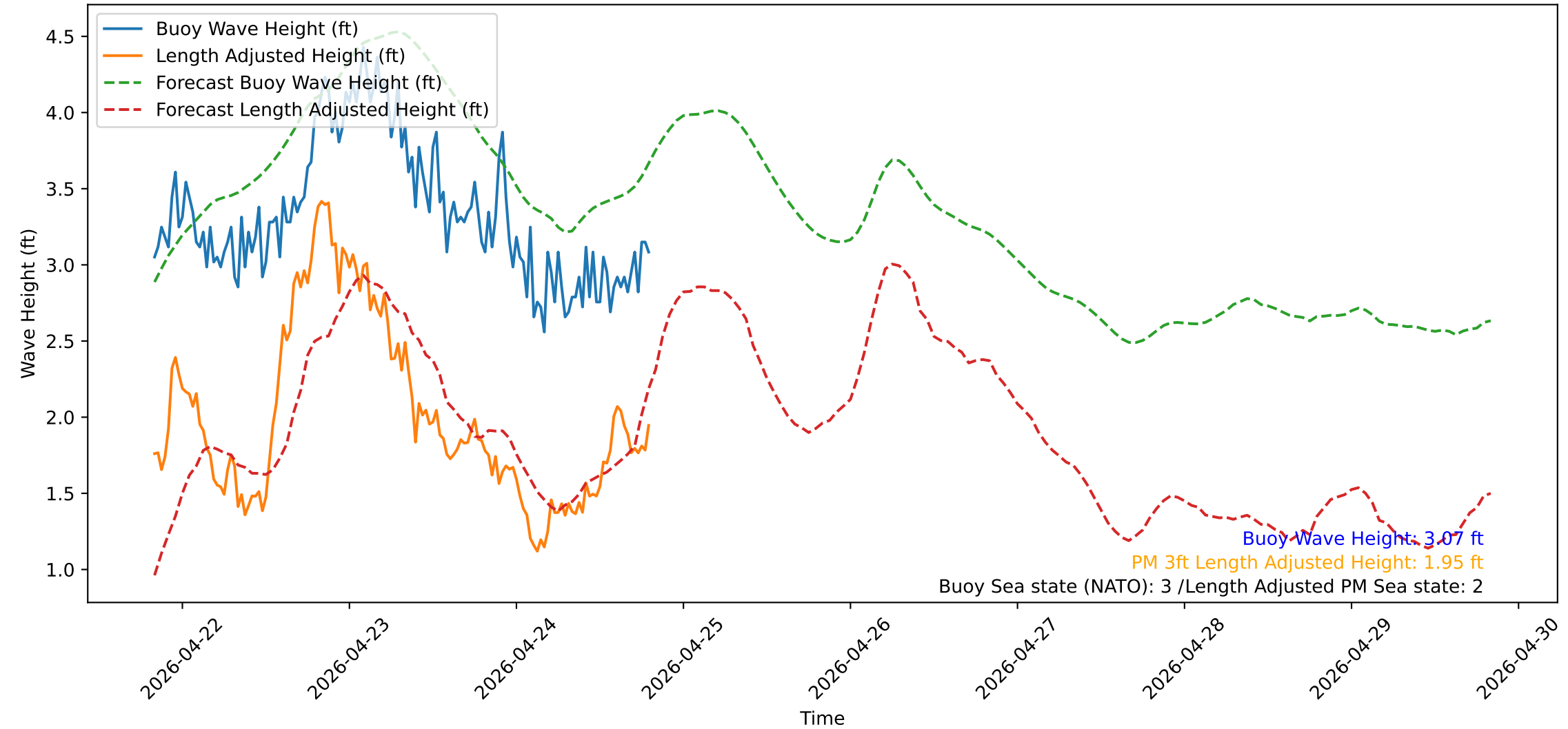
Wave Heights over Time for Oceanside Harbor at 2026-04-24 20:10:31
