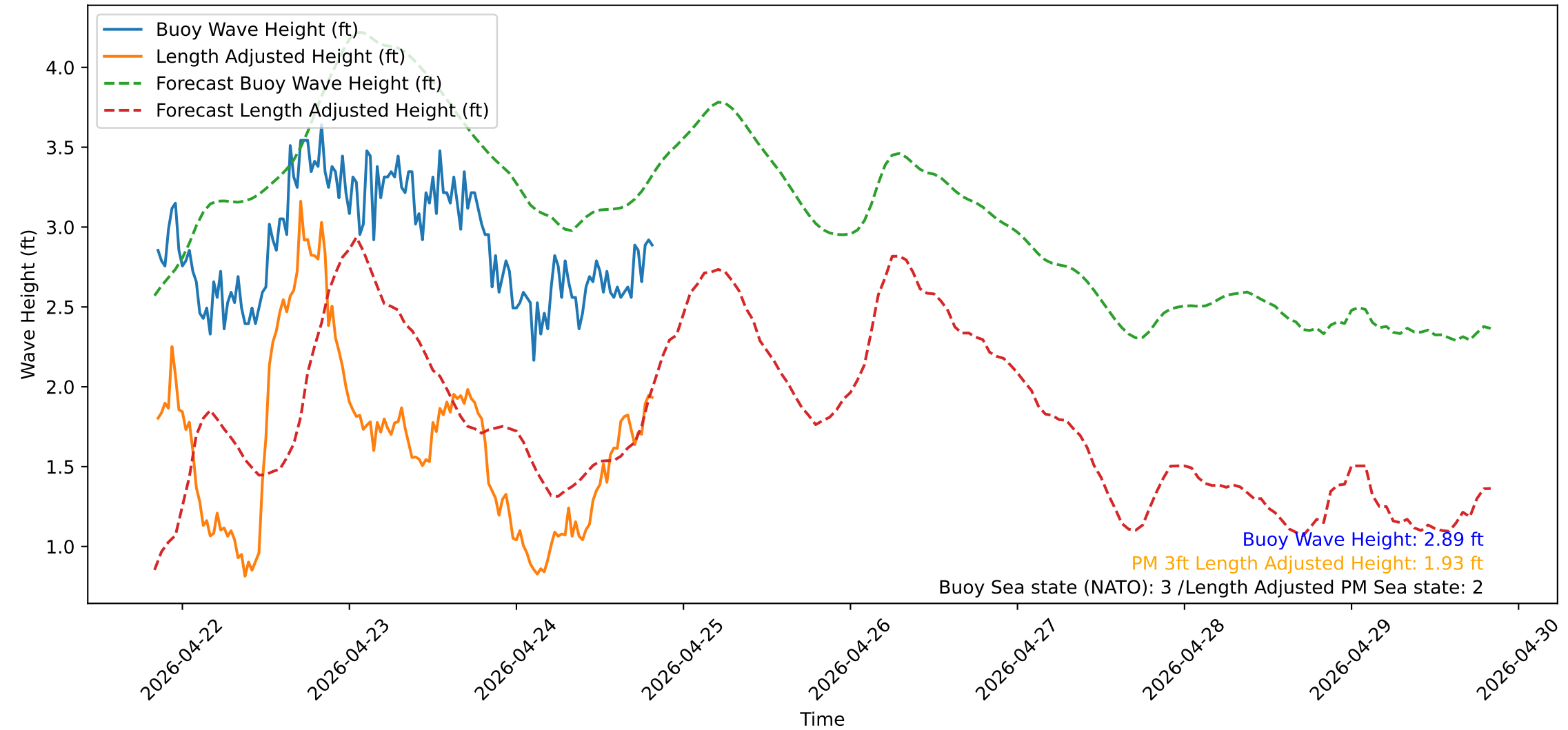
Wave Heights over Time for Red Beach at 2026-04-24 20:10:50
