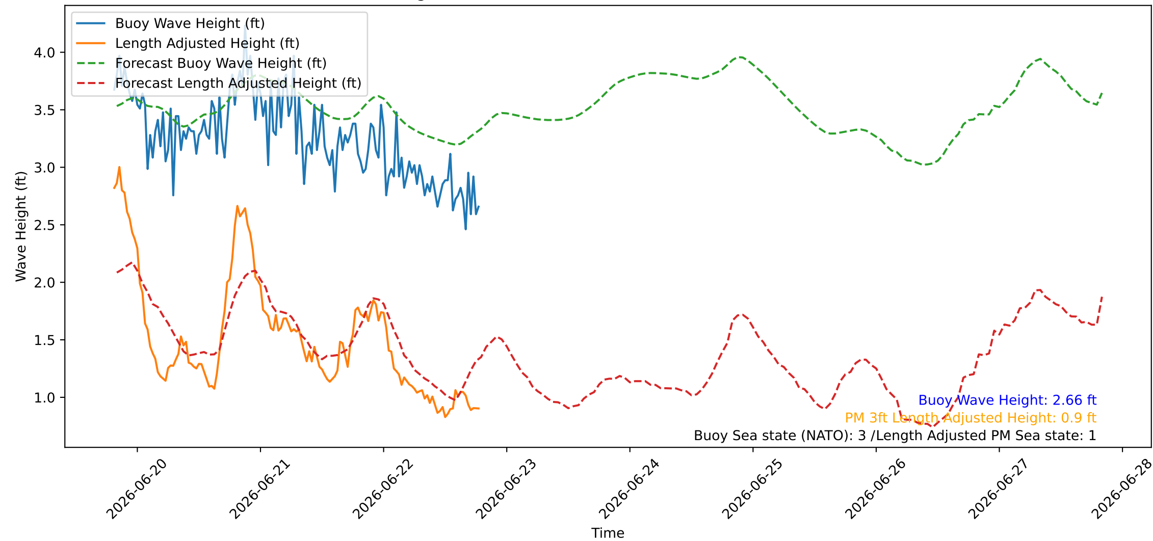
Wave Heights over Time for Green Beach at 2026-06-22 19:31:08
