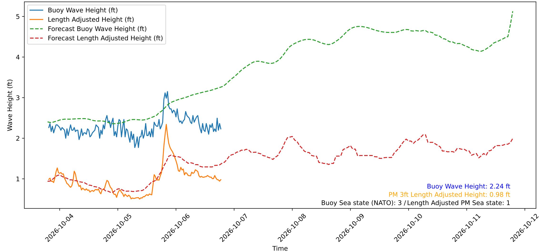
Wave Heights over Time for Green Beach at 2026-10-06 19:11:11
