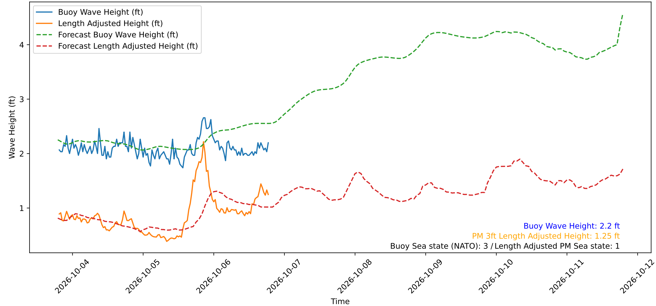
Wave Heights over Time for Red Beach at 2026-10-06 19:10:49
