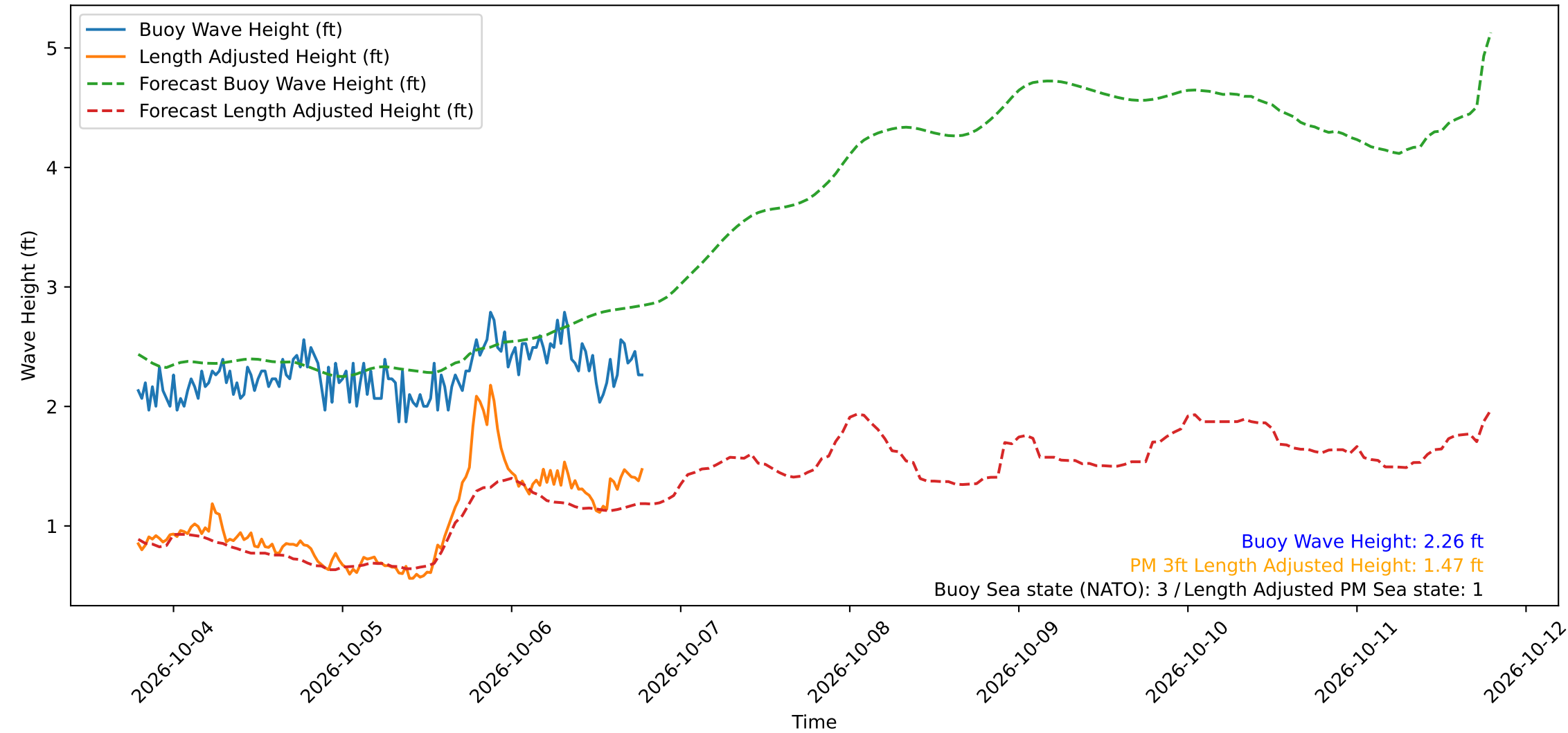
Wave Heights over Time for Oceanside Harbor at 2026-10-06 19:10:29
