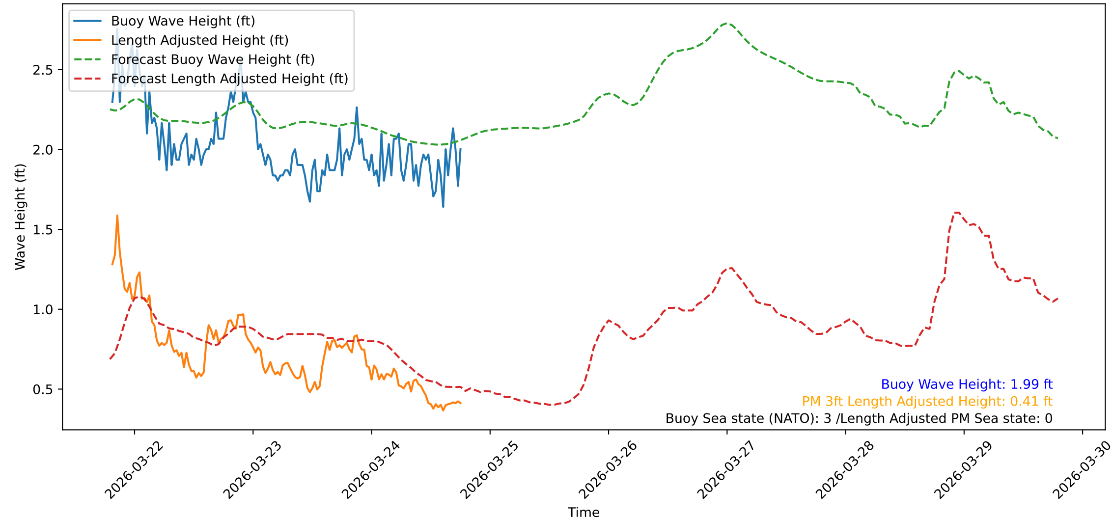
Wave Heights over Time for Red Beach at 2026-03-24 19:10:48
