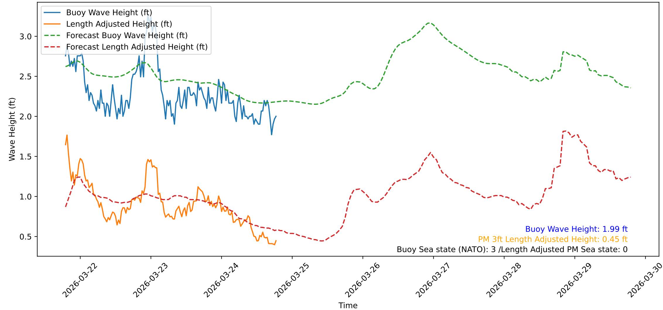
Wave Heights over Time for Green Beach at 2026-03-24 19:11:10
