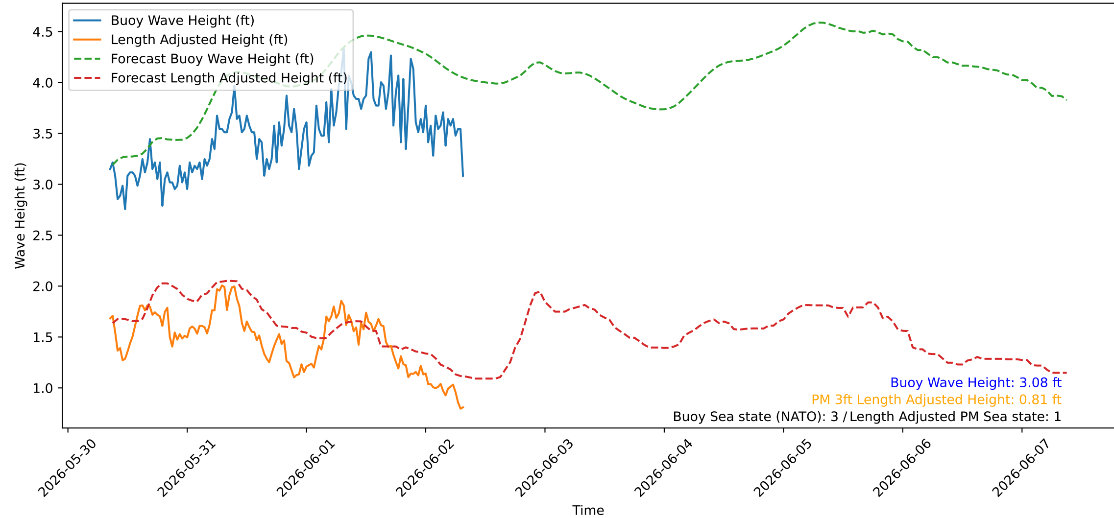
Wave Heights over Time for Green Beach at 2026-06-02 08:31:07
