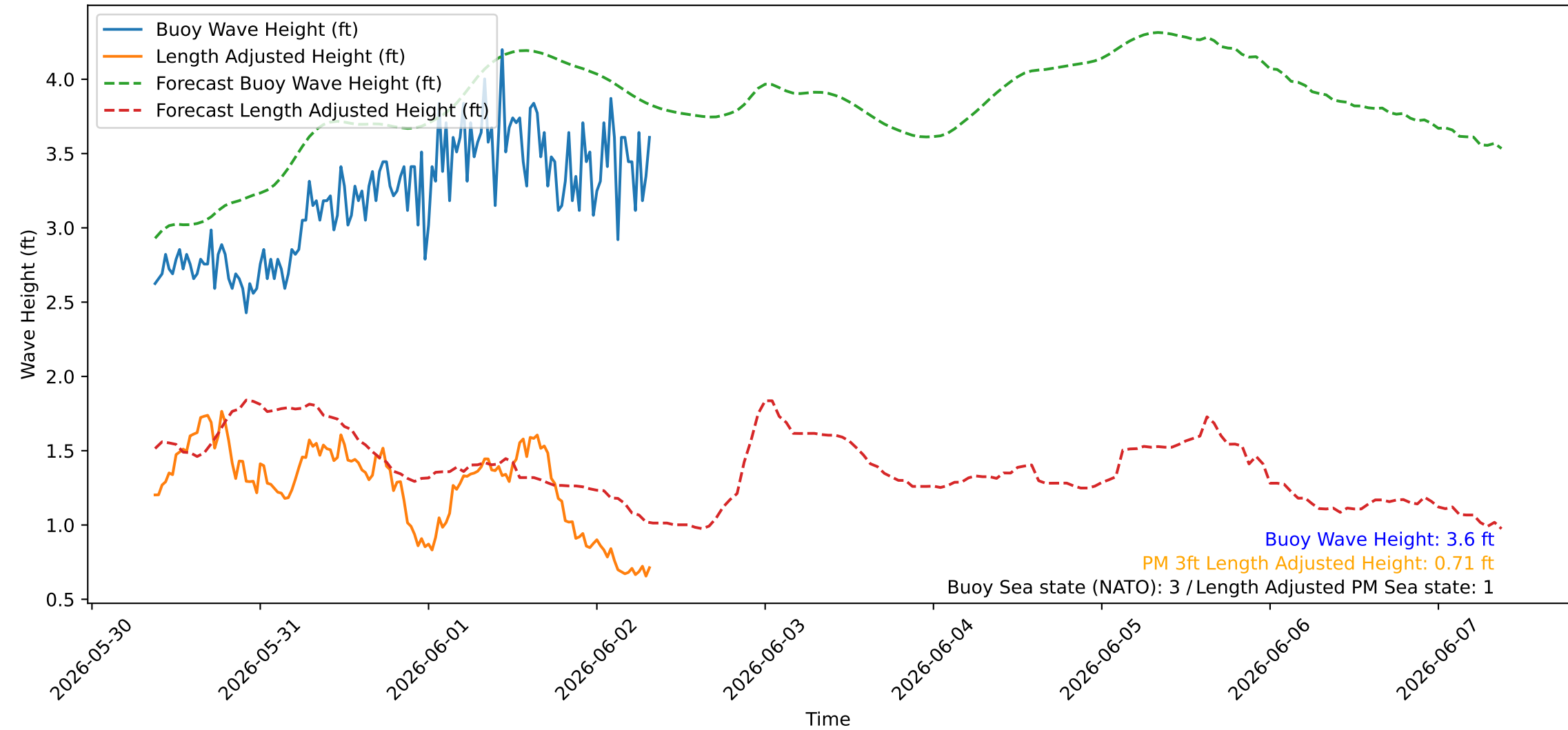
Wave Heights over Time for Red Beach at 2026-06-02 08:30:45
