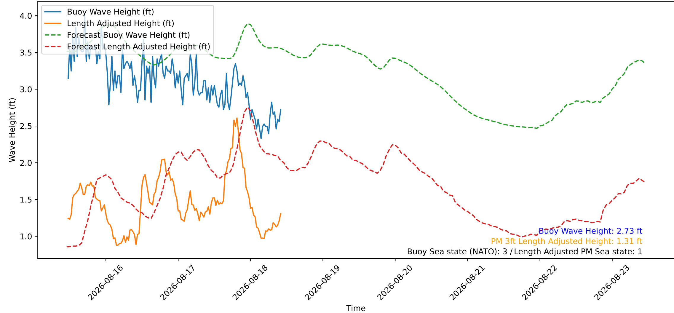
Wave Heights over Time for Red Beach at 2026-08-18 11:10:45
