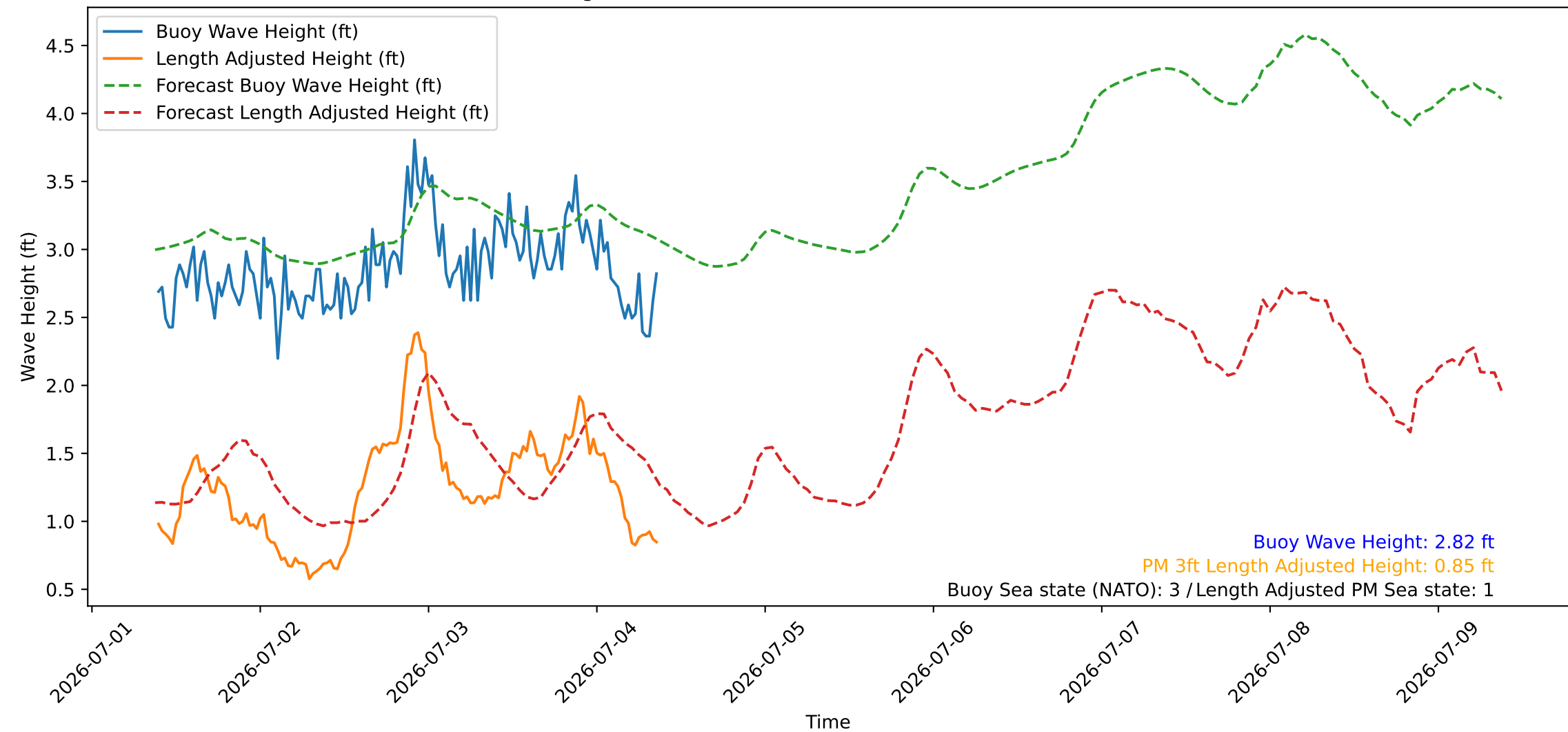
Wave Heights over Time for Red Beach at 2026-07-04 09:10:46
