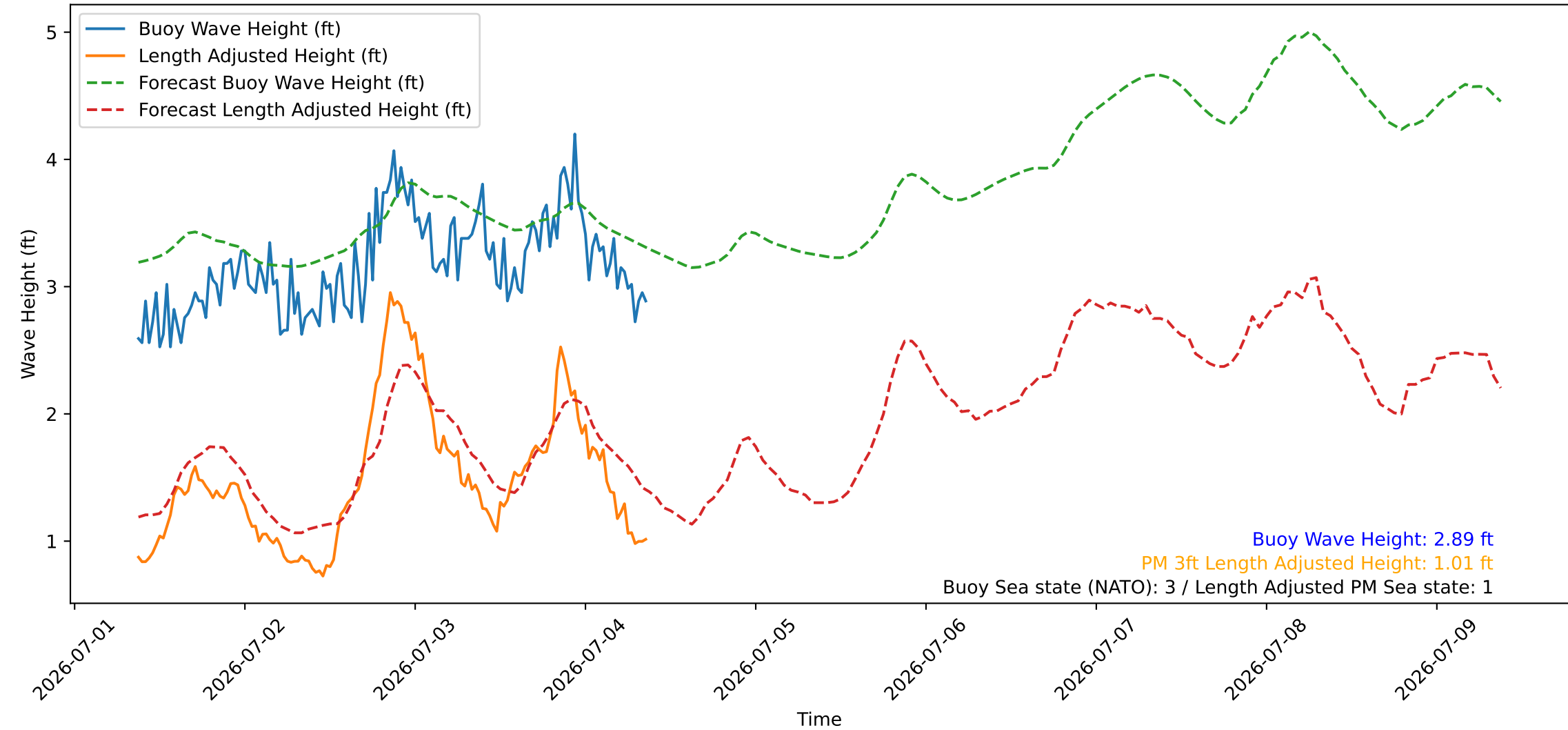
Wave Heights over Time for Green Beach at 2026-07-04 09:11:08
