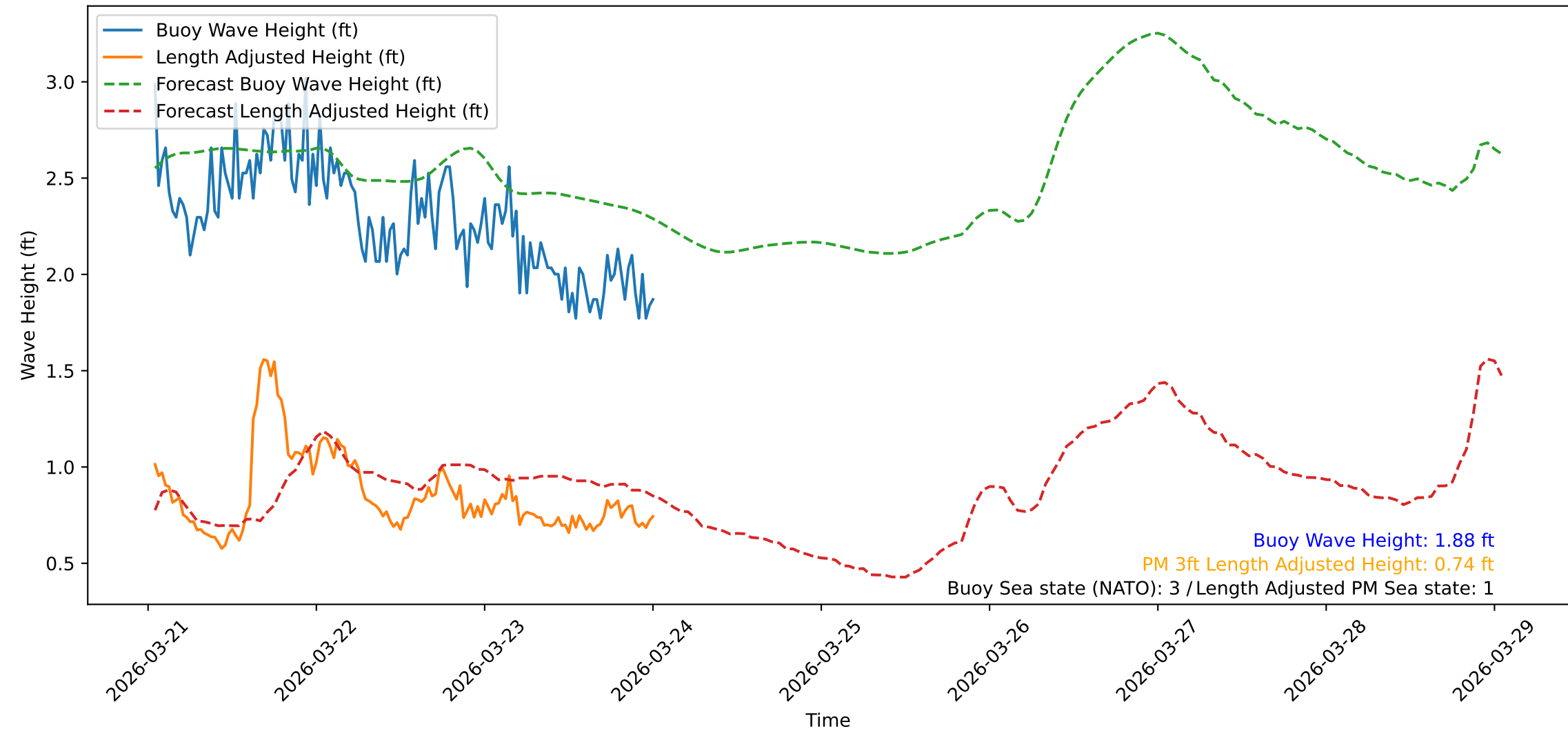
Wave Heights over Time for Oceanside Harbor at 2026-03-24 00:50:31
