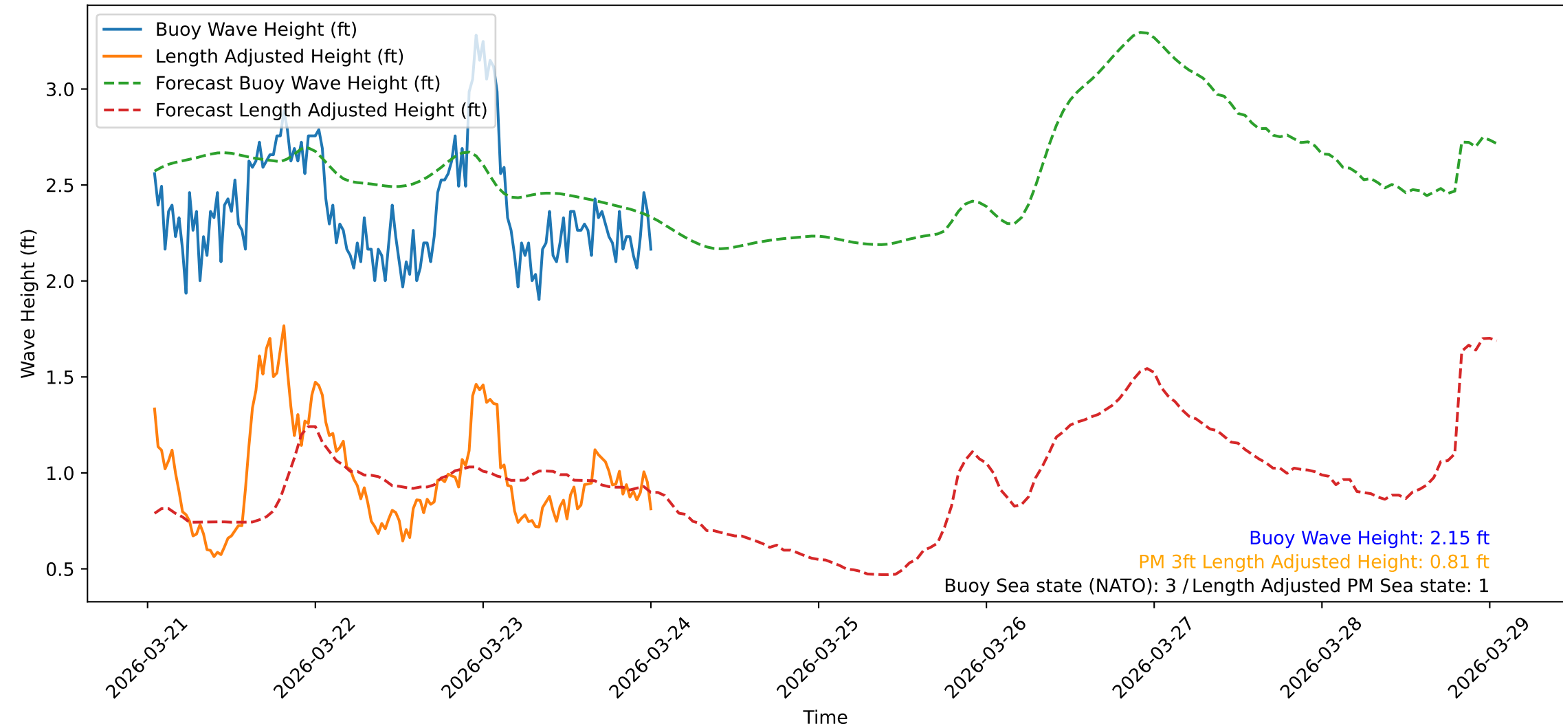
Wave Heights over Time for Green Beach at 2026-03-24 00:51:09
