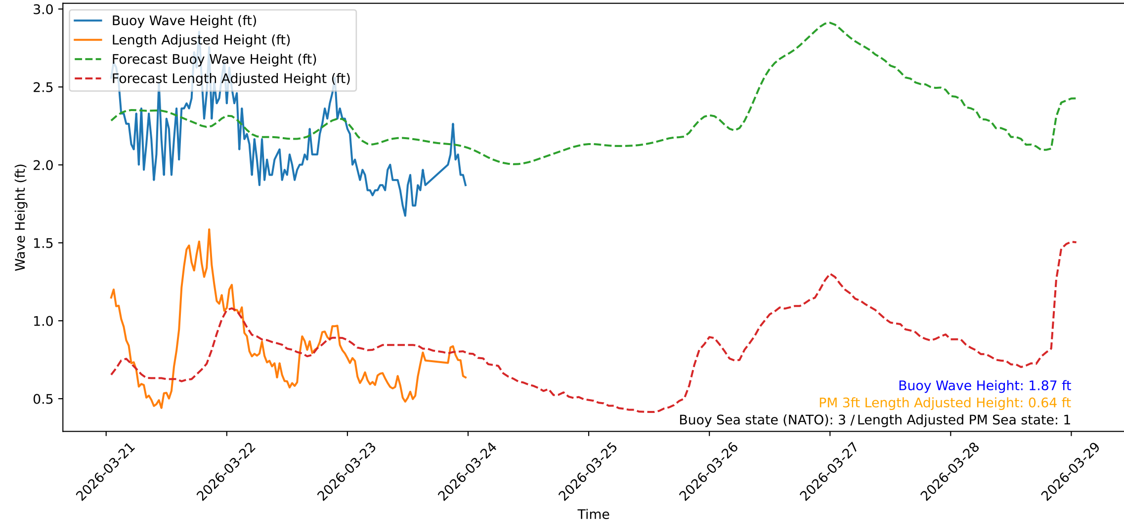
Wave Heights over Time for Red Beach at 2026-03-24 00:50:47
