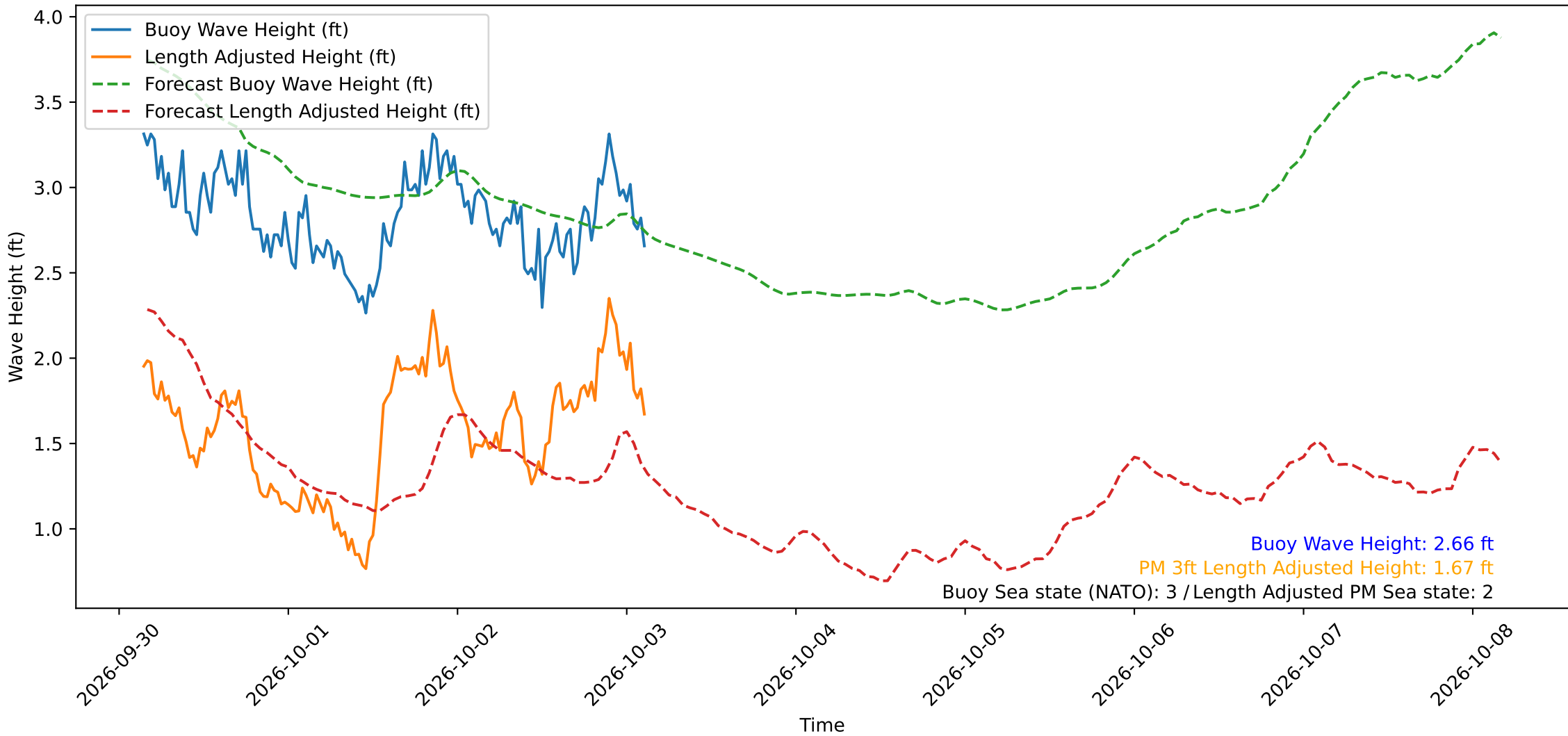
Wave Heights over Time for Oceanside Harbor at 2026-10-03 03:30:29
