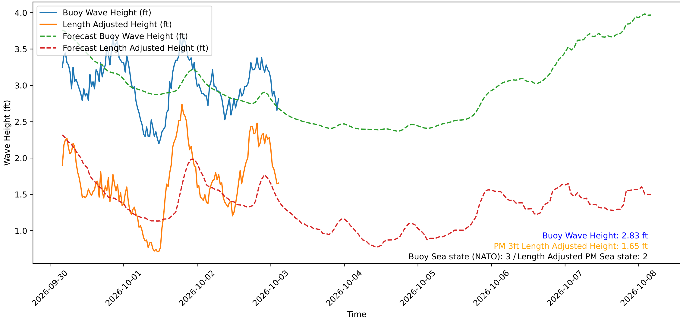
Wave Heights over Time for Green Beach at 2026-10-03 03:31:12
