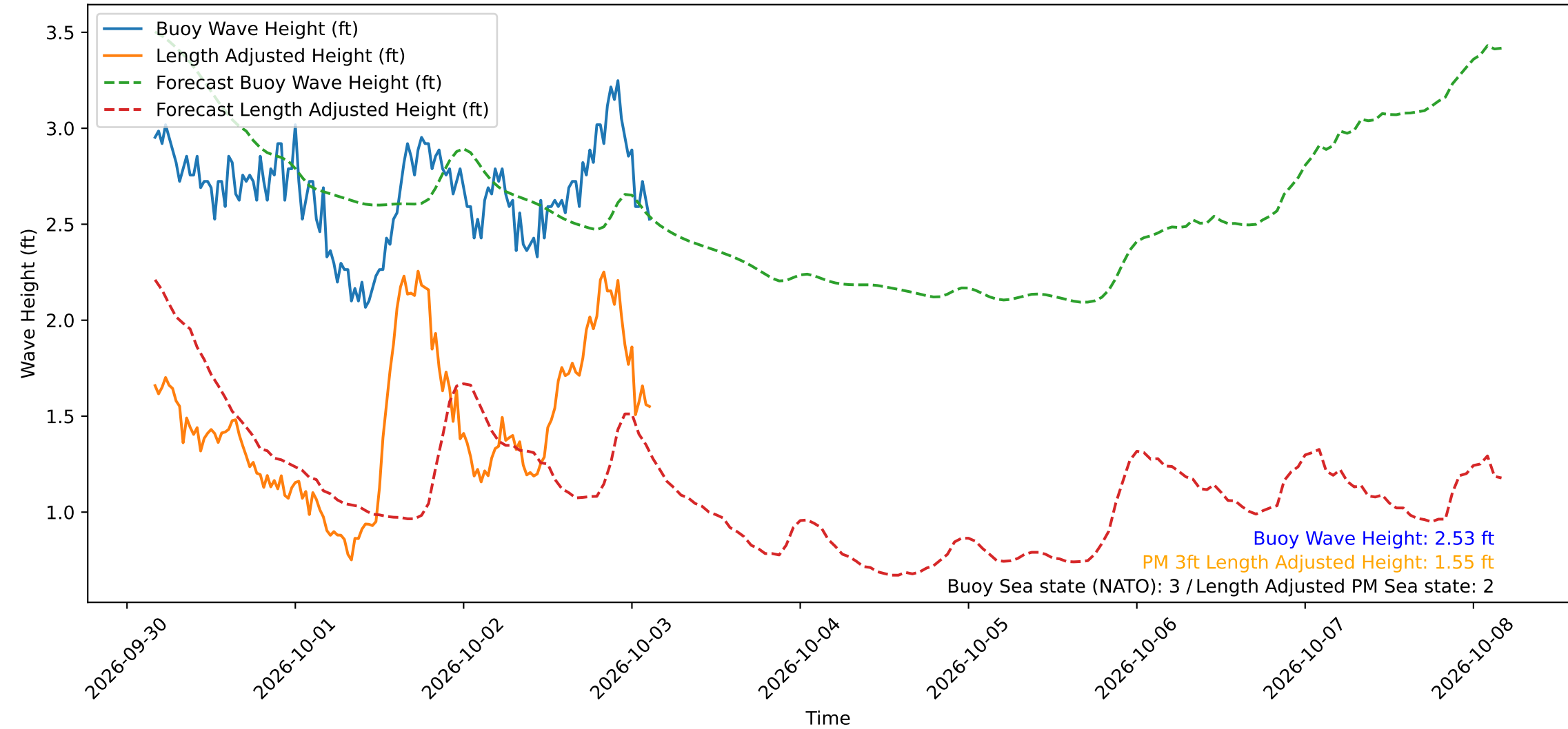
Wave Heights over Time for Red Beach at 2026-10-03 03:30:48
