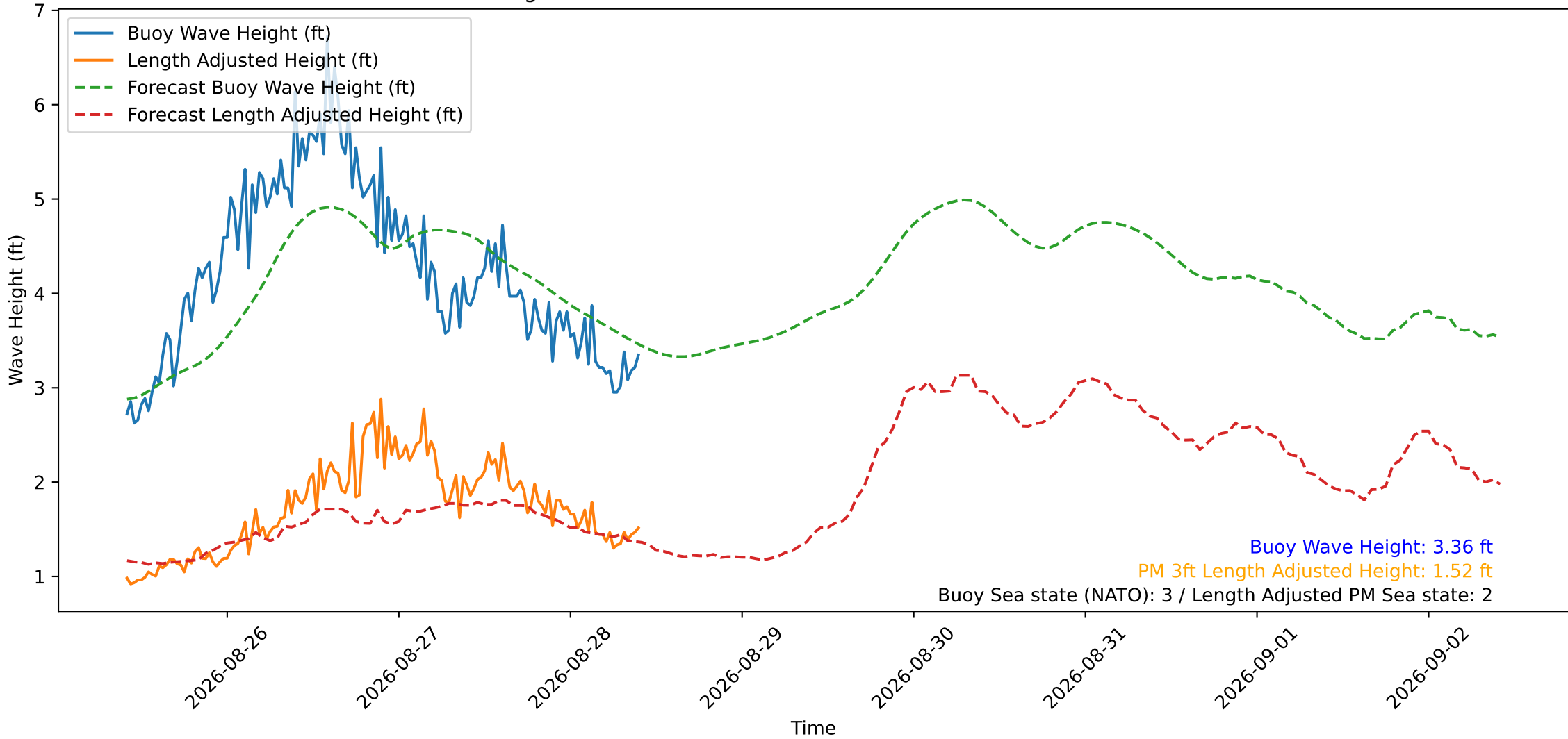
Wave Heights over Time for Oceanside Harbor at 2026-08-28 10:10:29
