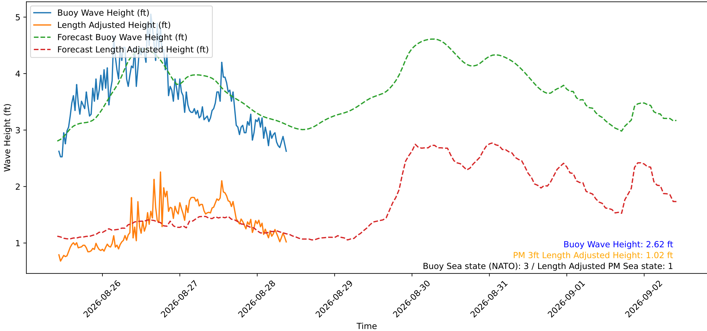
Wave Heights over Time for Red Beach at 2026-08-28 10:10:49
