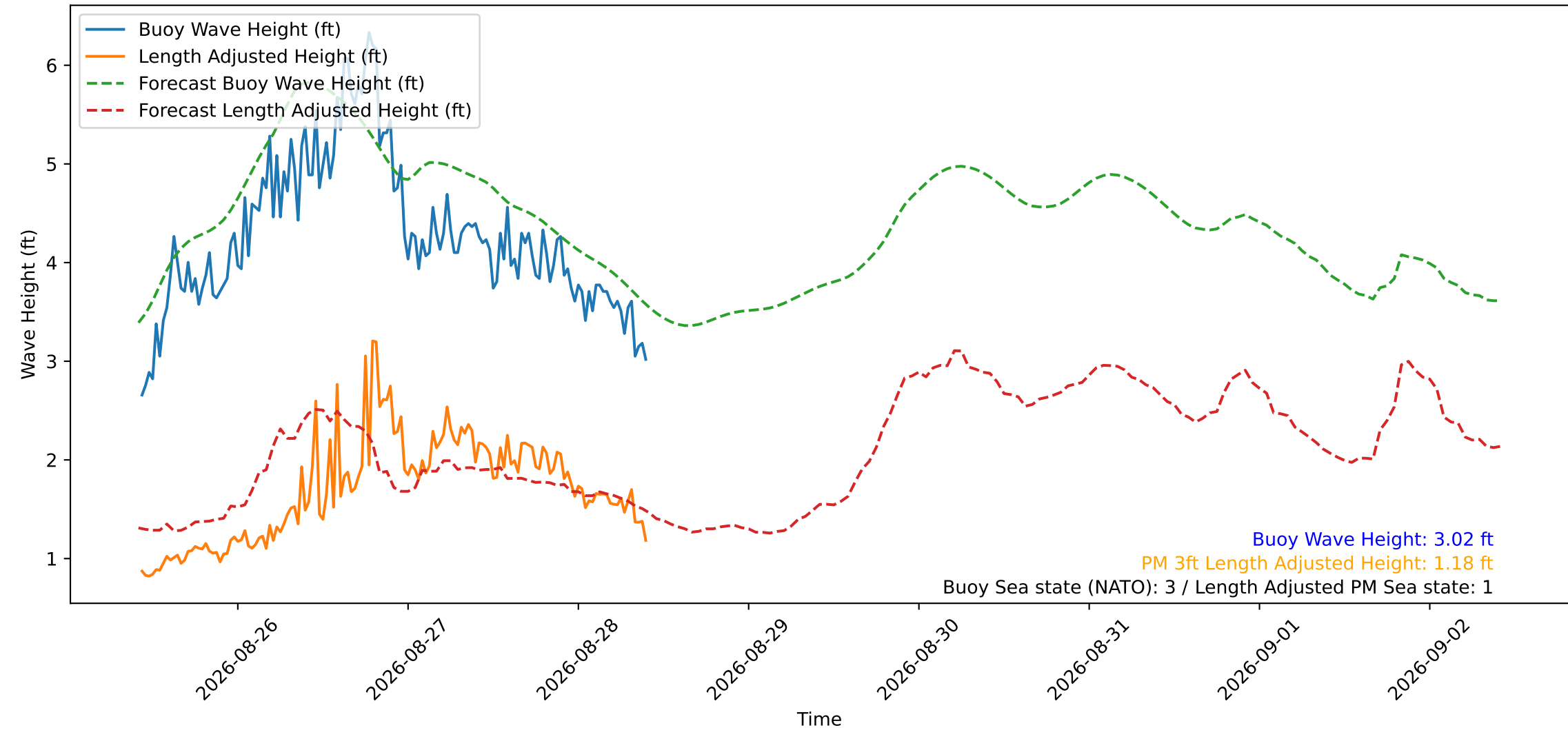
Wave Heights over Time for Green Beach at 2026-08-28 10:11:11
