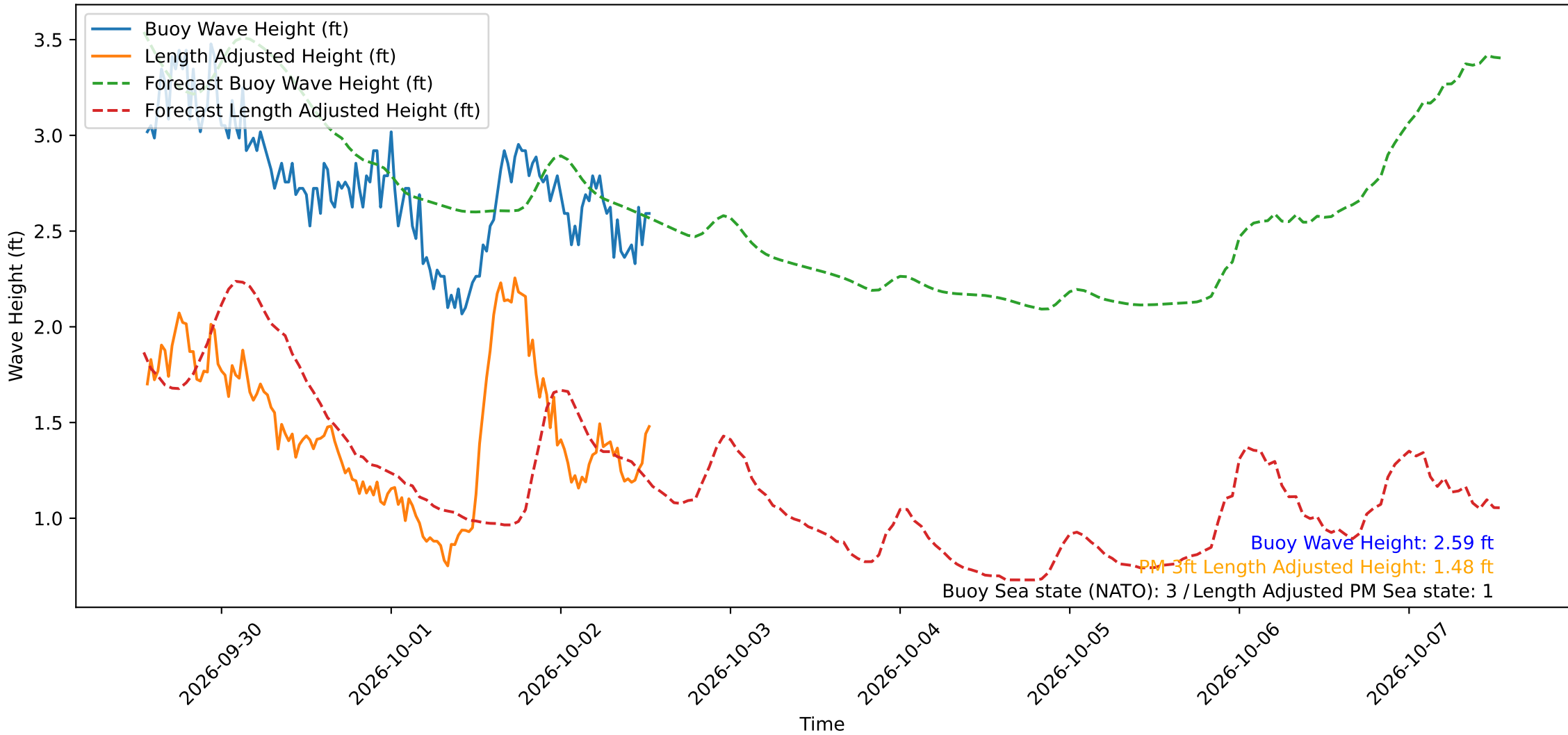
Wave Heights over Time for Red Beach at 2026-10-02 13:20:50
