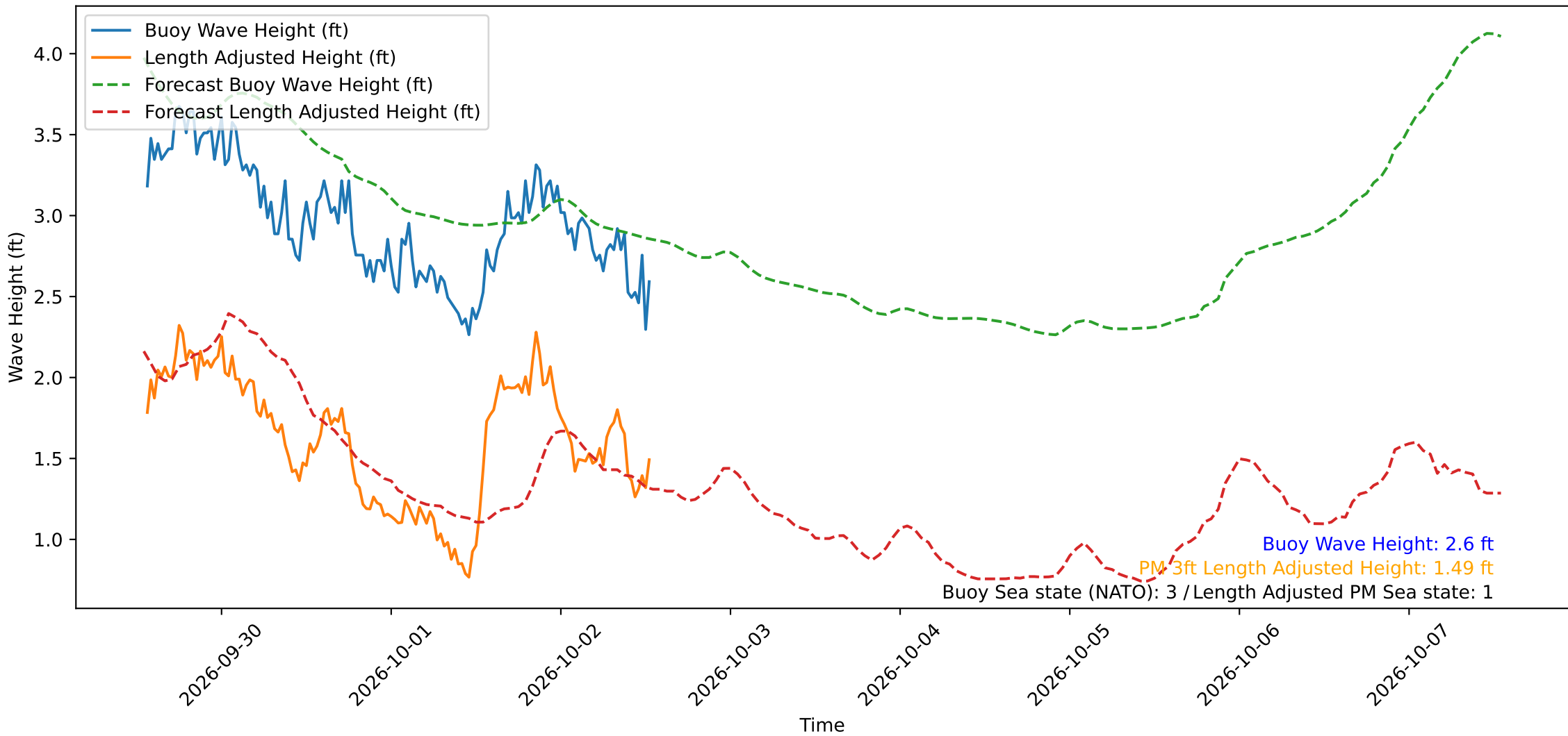
Wave Heights over Time for Oceanside Harbor at 2026-10-02 13:20:29
