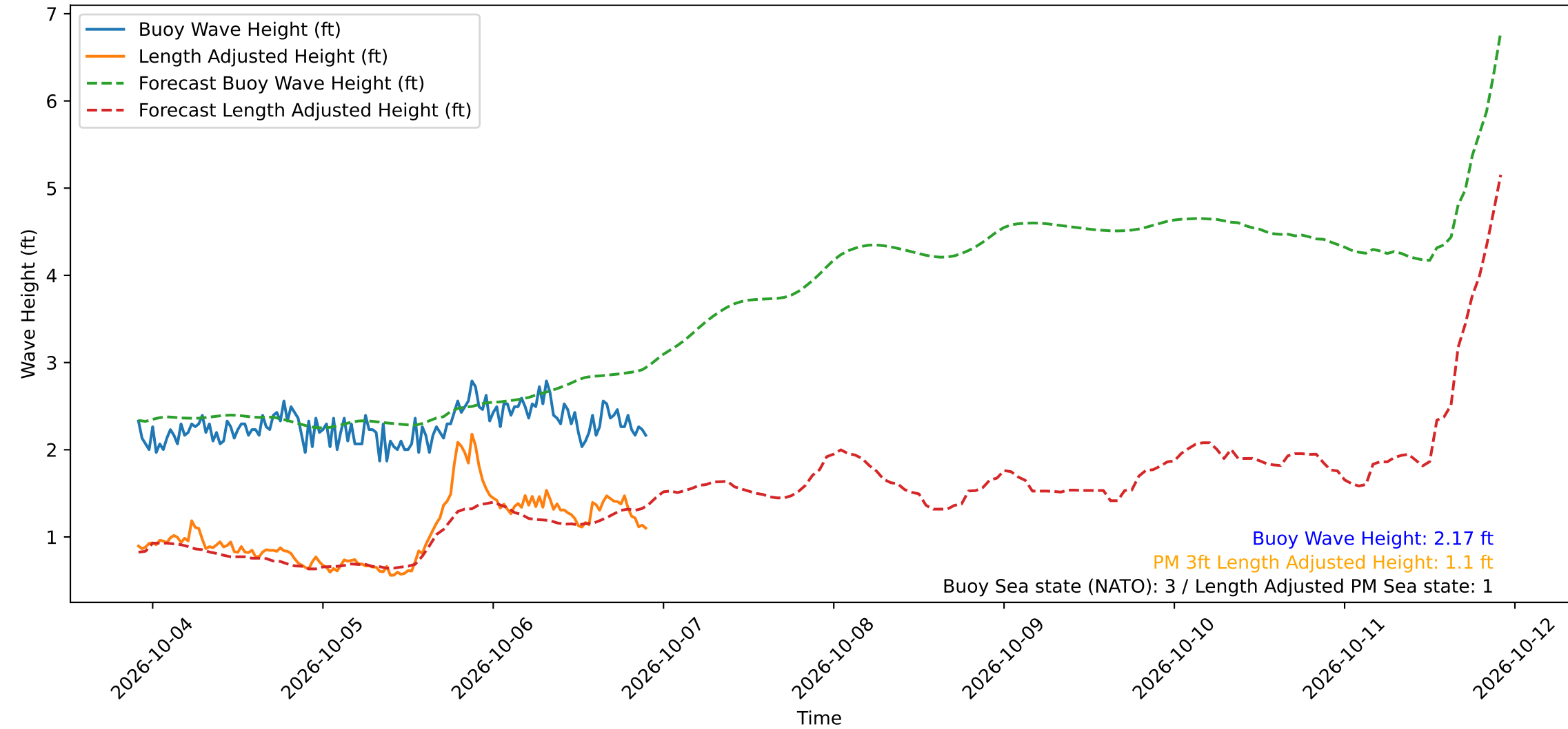
Wave Heights over Time for Oceanside Harbor at 2026-10-06 22:10:30
