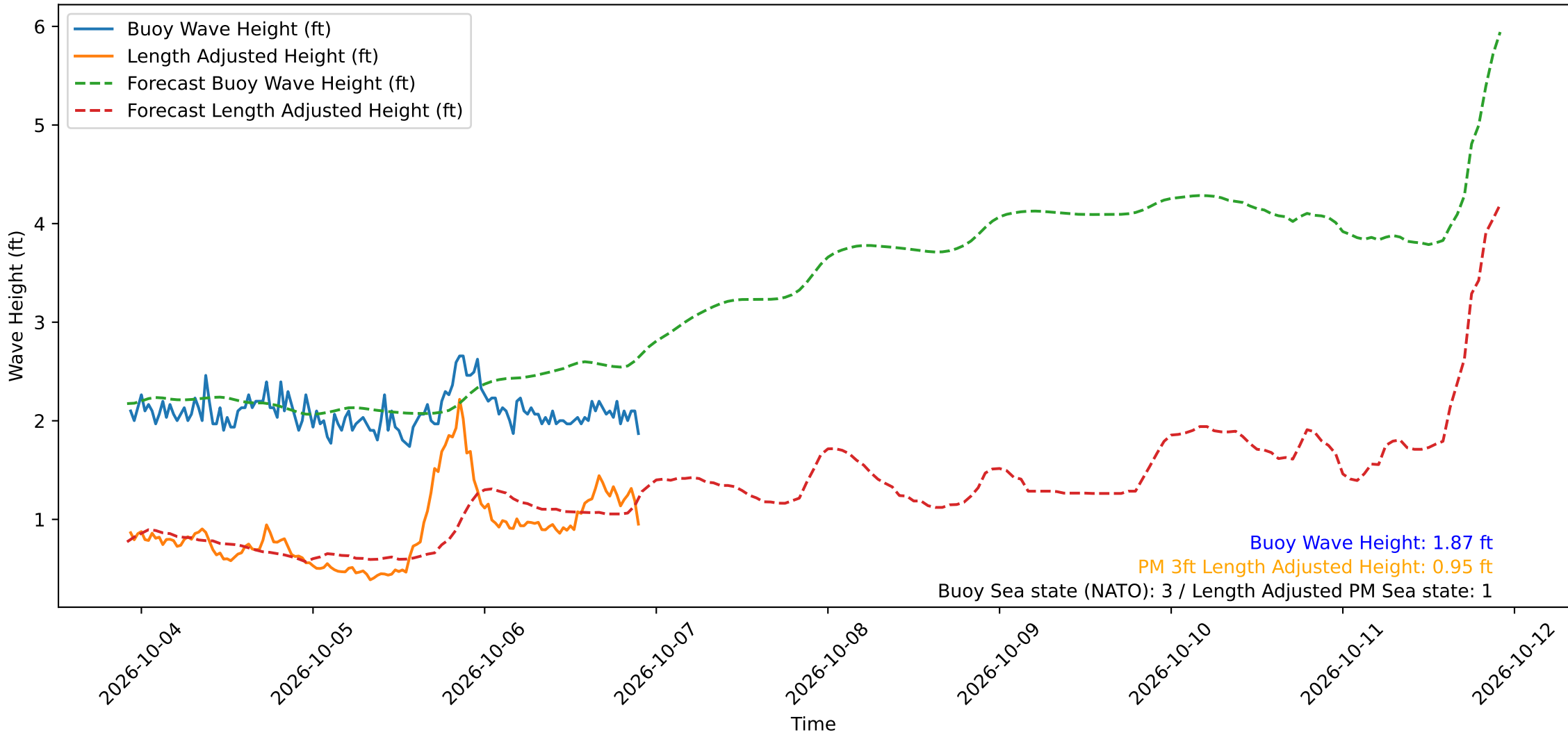
Wave Heights over Time for Red Beach at 2026-10-06 22:10:49
