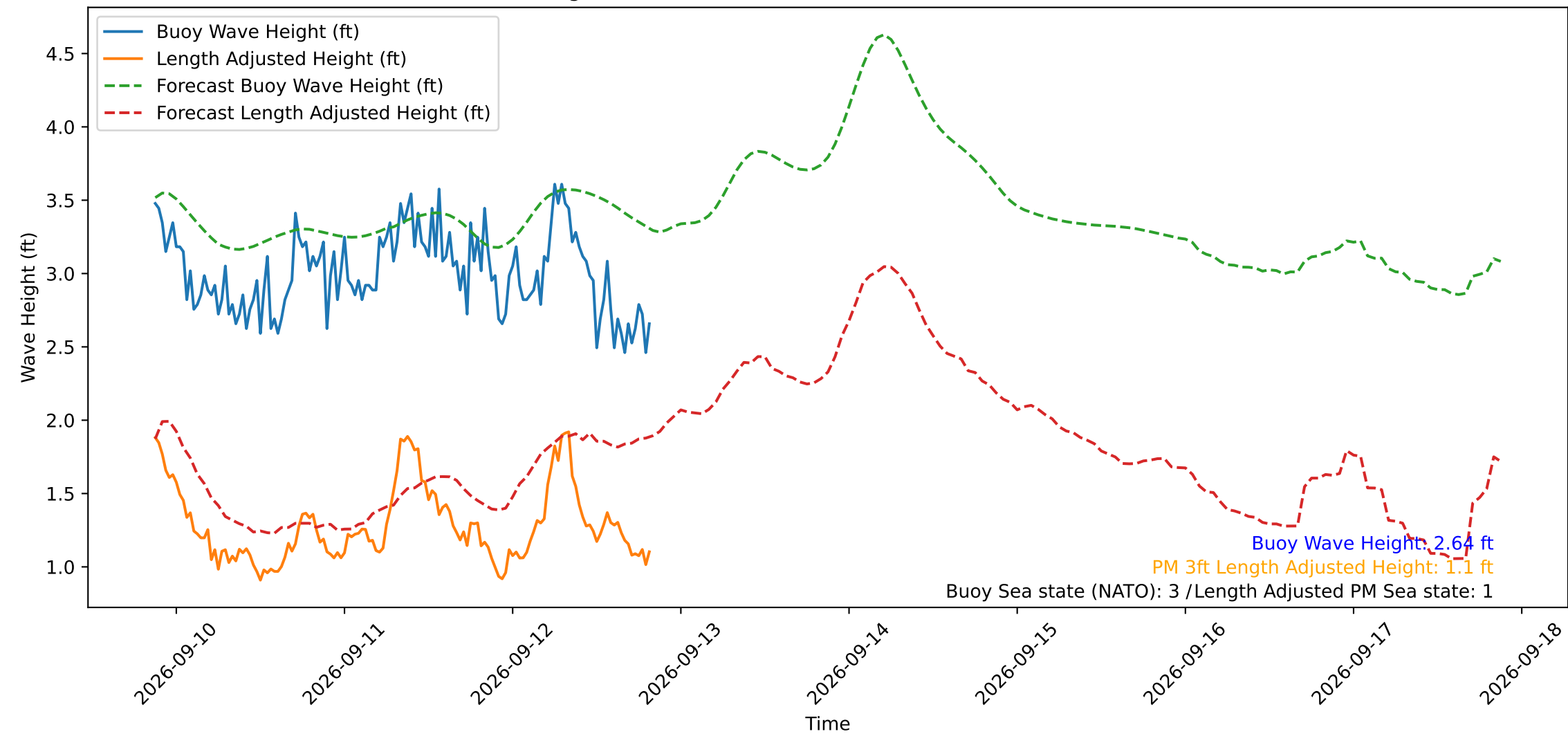
Wave Heights over Time for Green Beach at 2026-09-12 20:31:11
