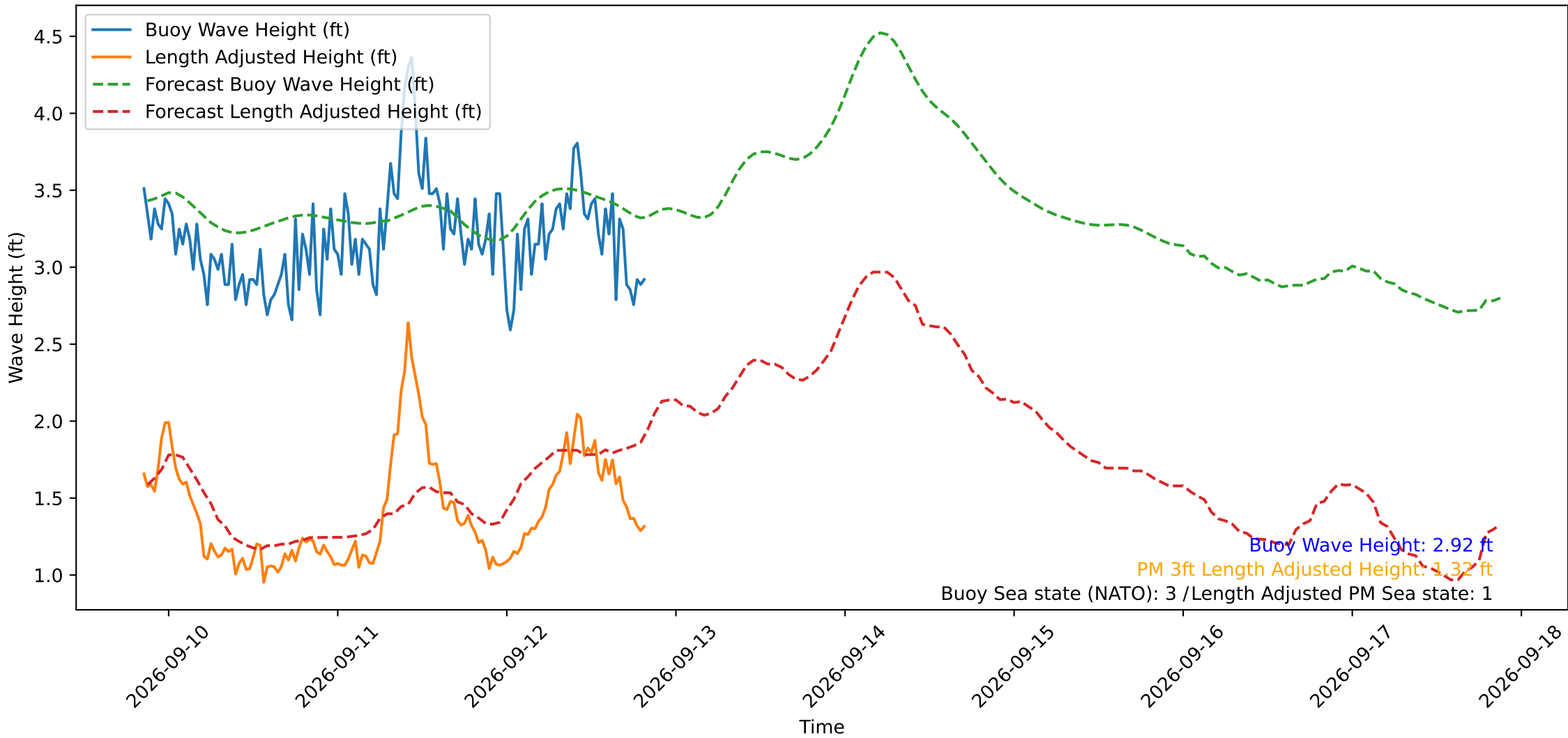
Wave Heights over Time for Oceanside Harbor at 2026-09-12 20:30:29
