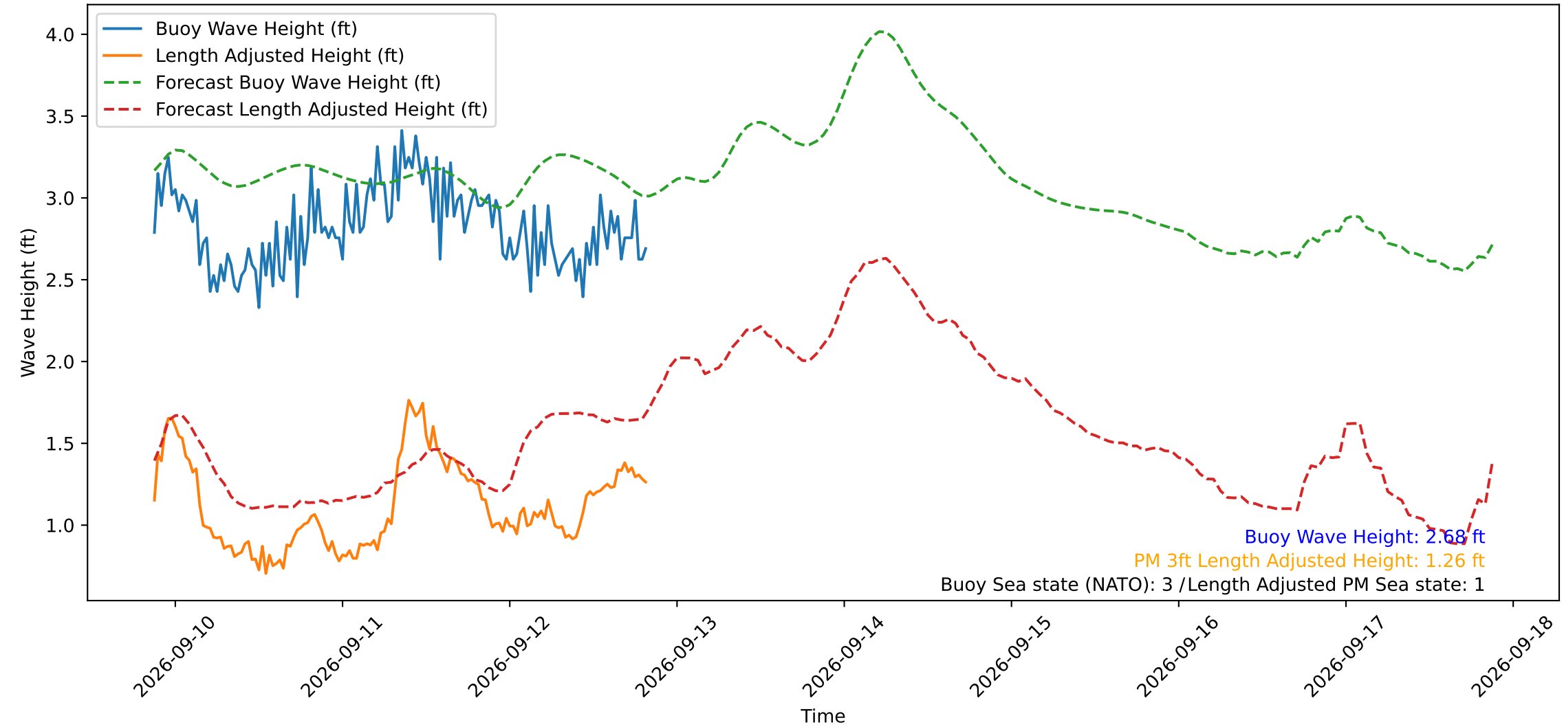
Wave Heights over Time for Red Beach at 2026-09-12 20:30:49
