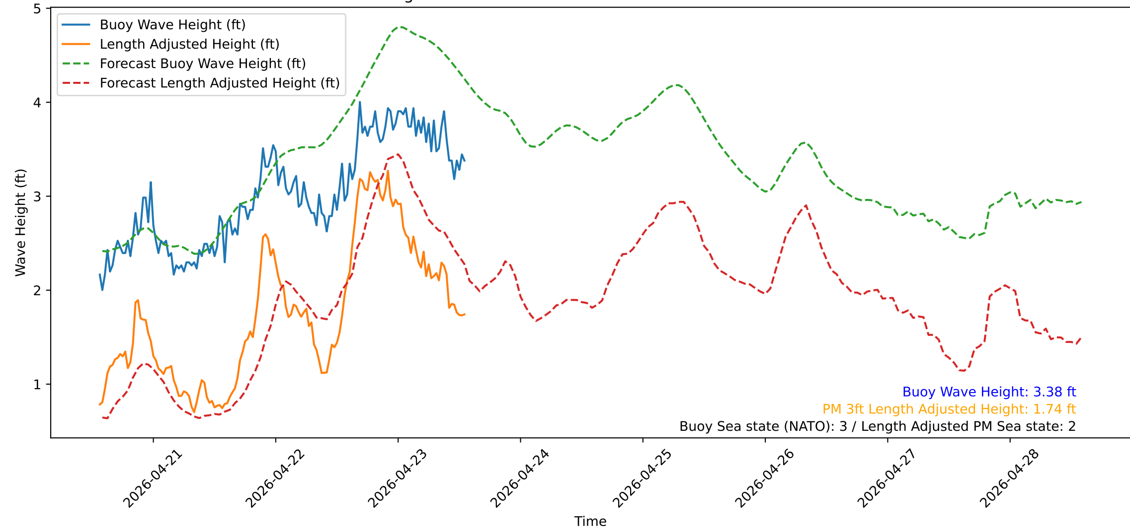
Wave Heights over Time for Green Beach at 2026-04-23 13:41:12
