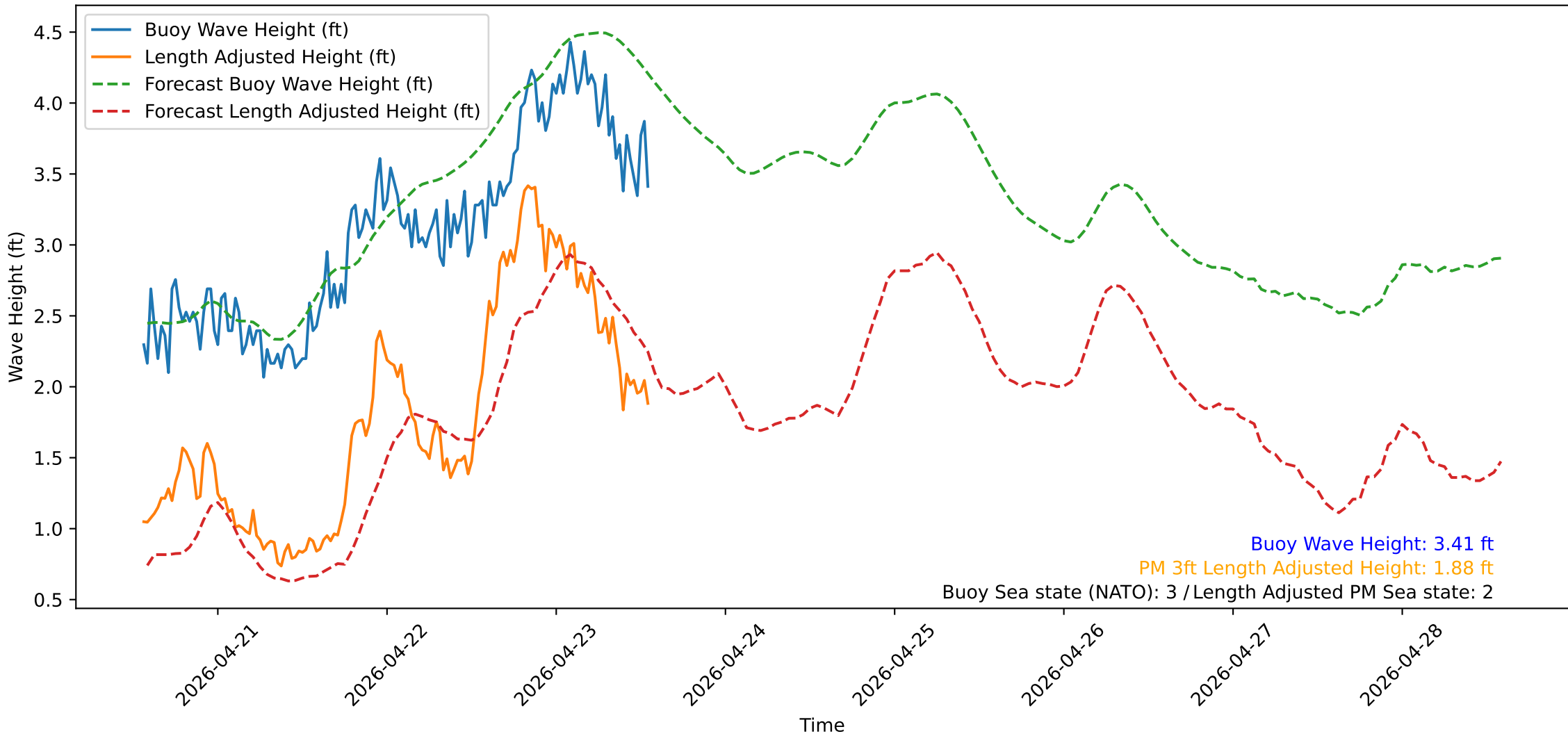
Wave Heights over Time for Oceanside Harbor at 2026-04-23 13:40:31
