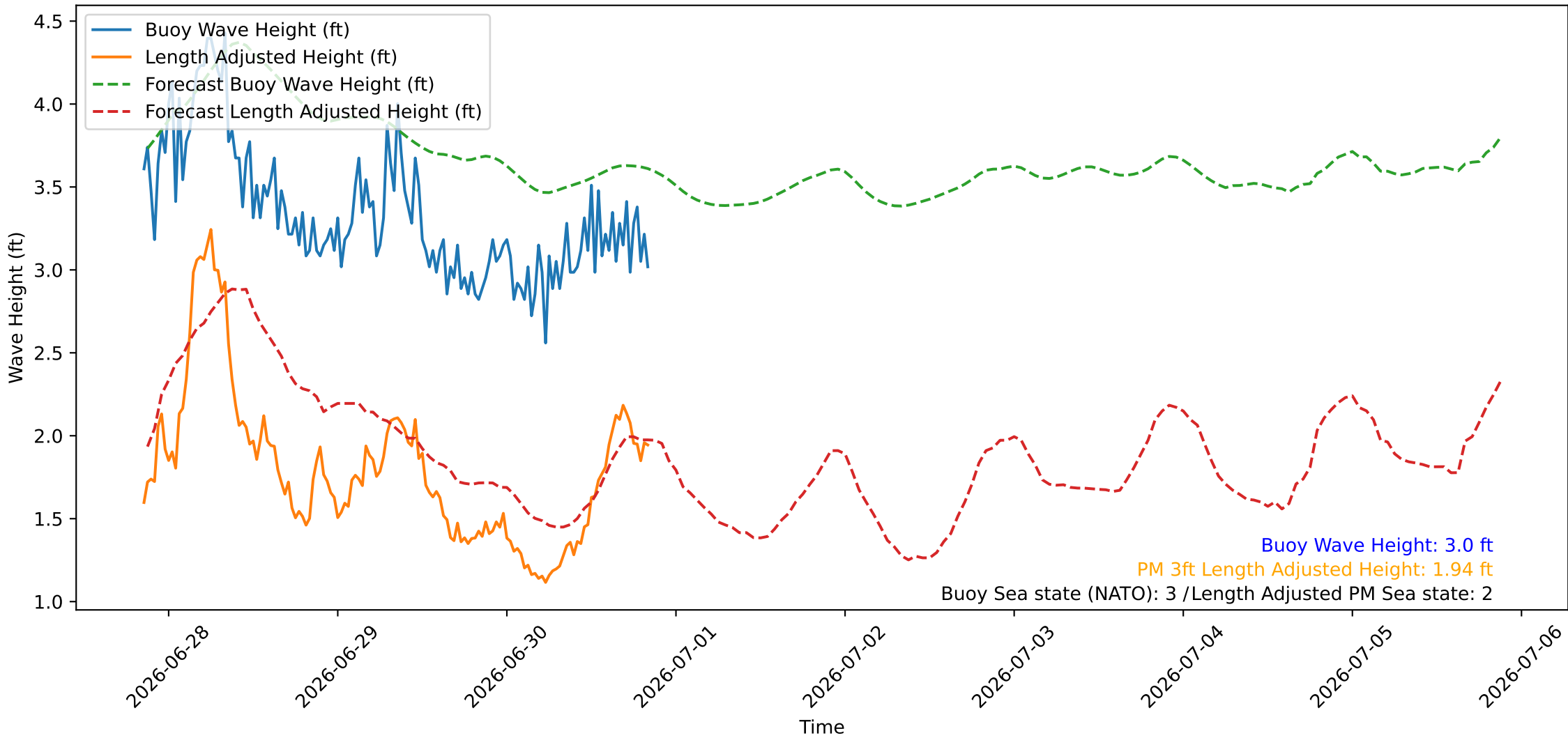
Wave Heights over Time for Oceanside Harbor at 2026-06-30 20:40:26
