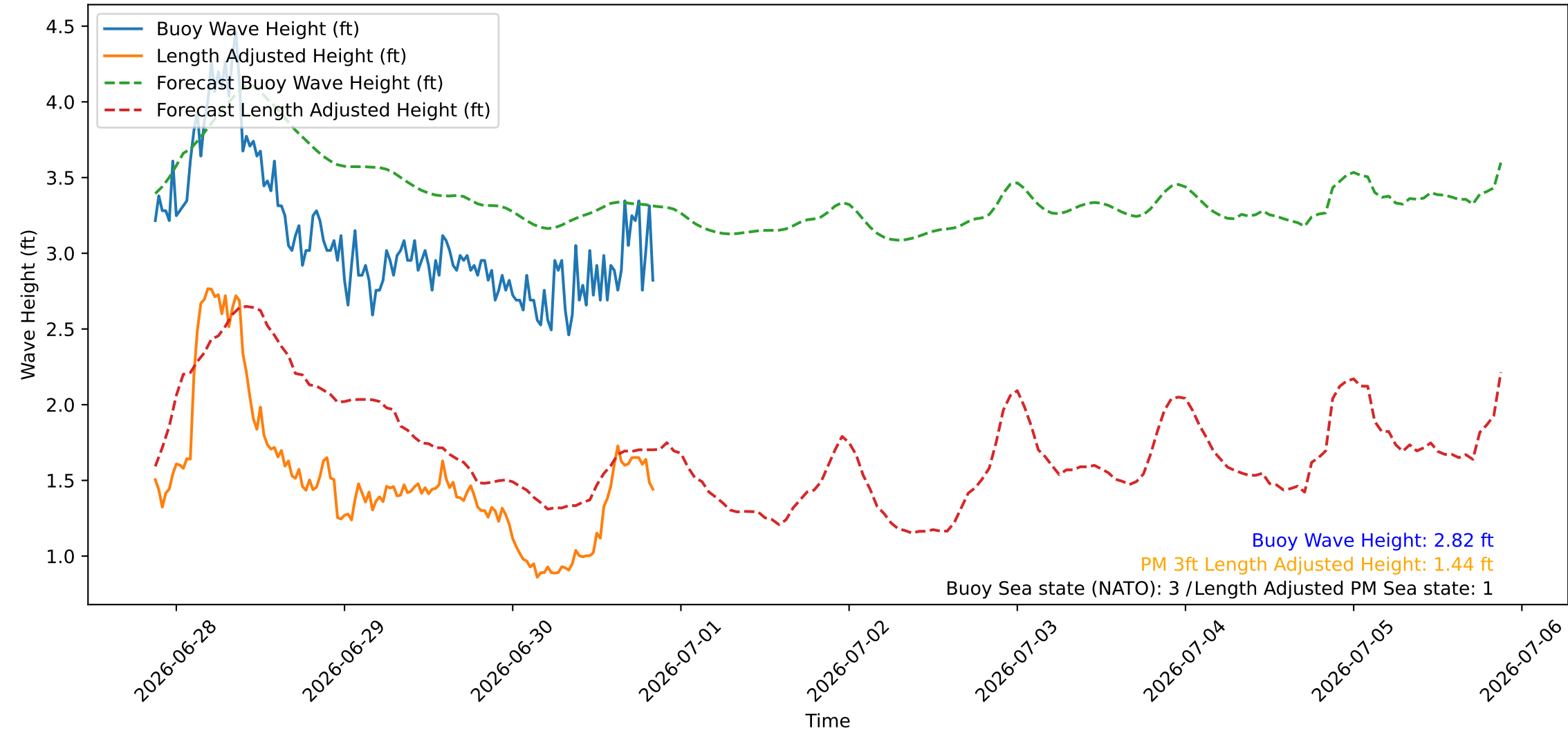
Wave Heights over Time for Red Beach at 2026-06-30 20:40:46
