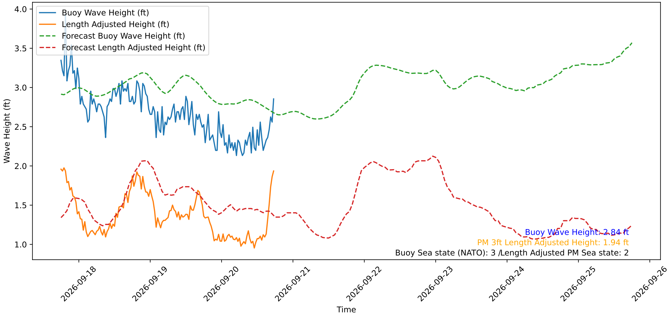
Wave Heights over Time for Oceanside Harbor at 2026-09-20 18:10:29
