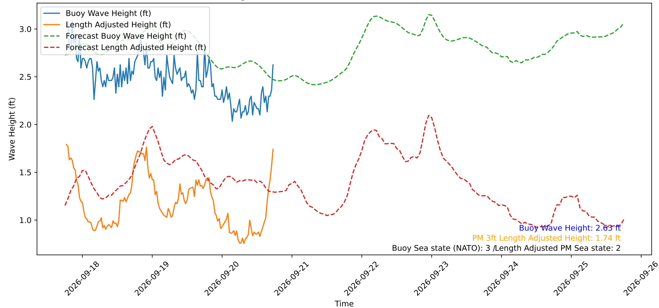
Wave Heights over Time for Red Beach at 2026-09-20 18:10:49
