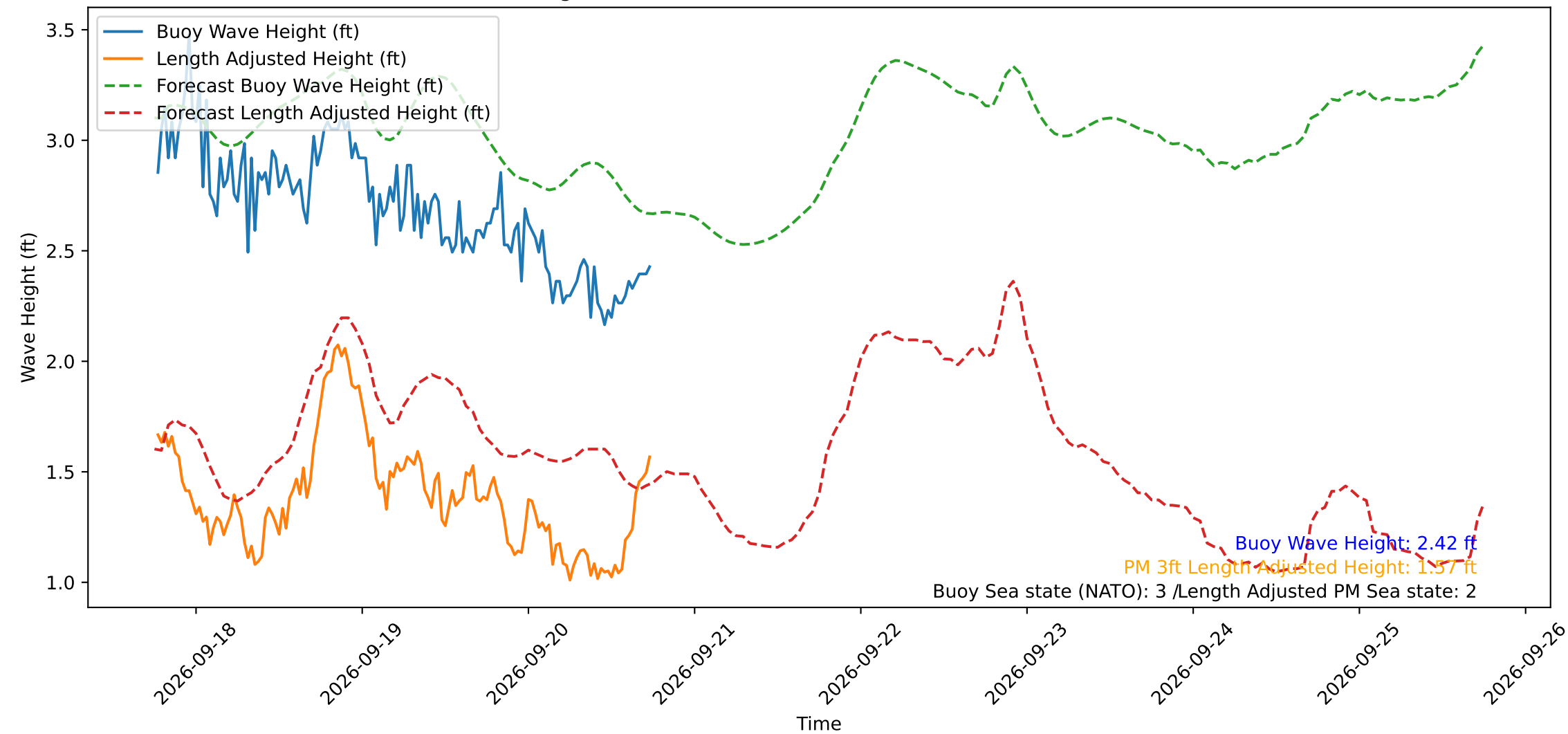
Wave Heights over Time for Green Beach at 2026-09-20 18:11:12
