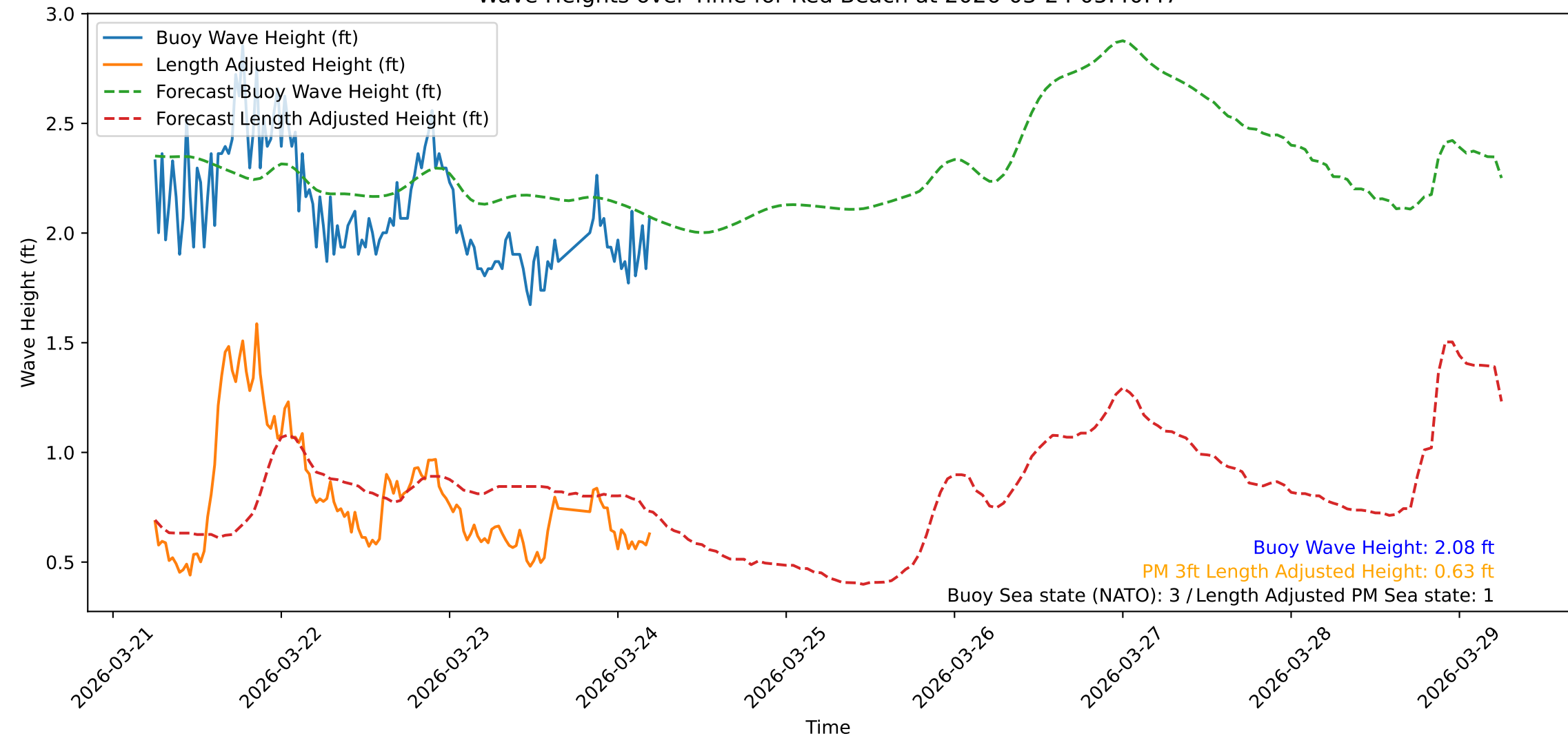
Wave Heights over Time for Red Beach at 2026-03-24 05:40:47
