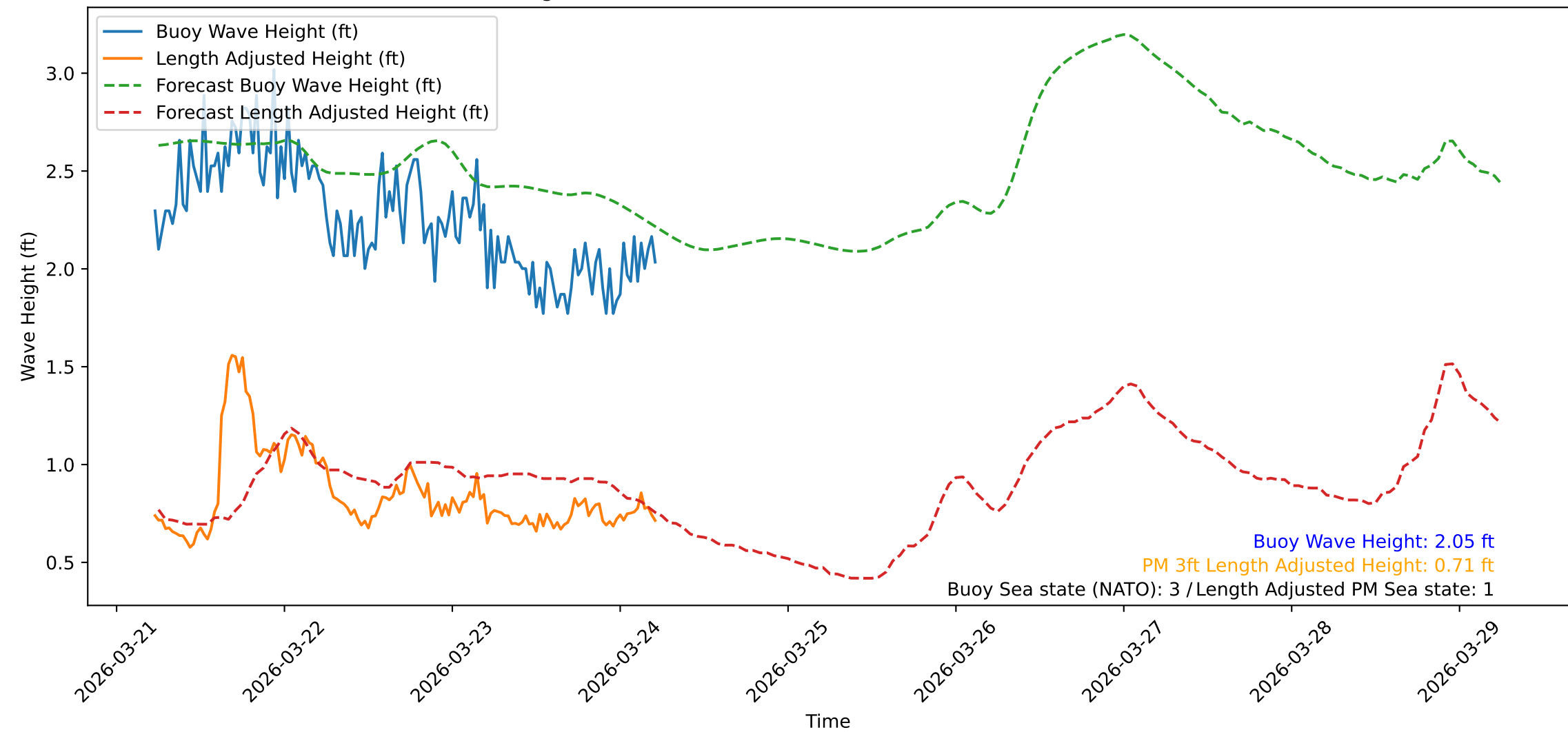
Wave Heights over Time for Oceanside Harbor at 2026-03-24 05:40:31
