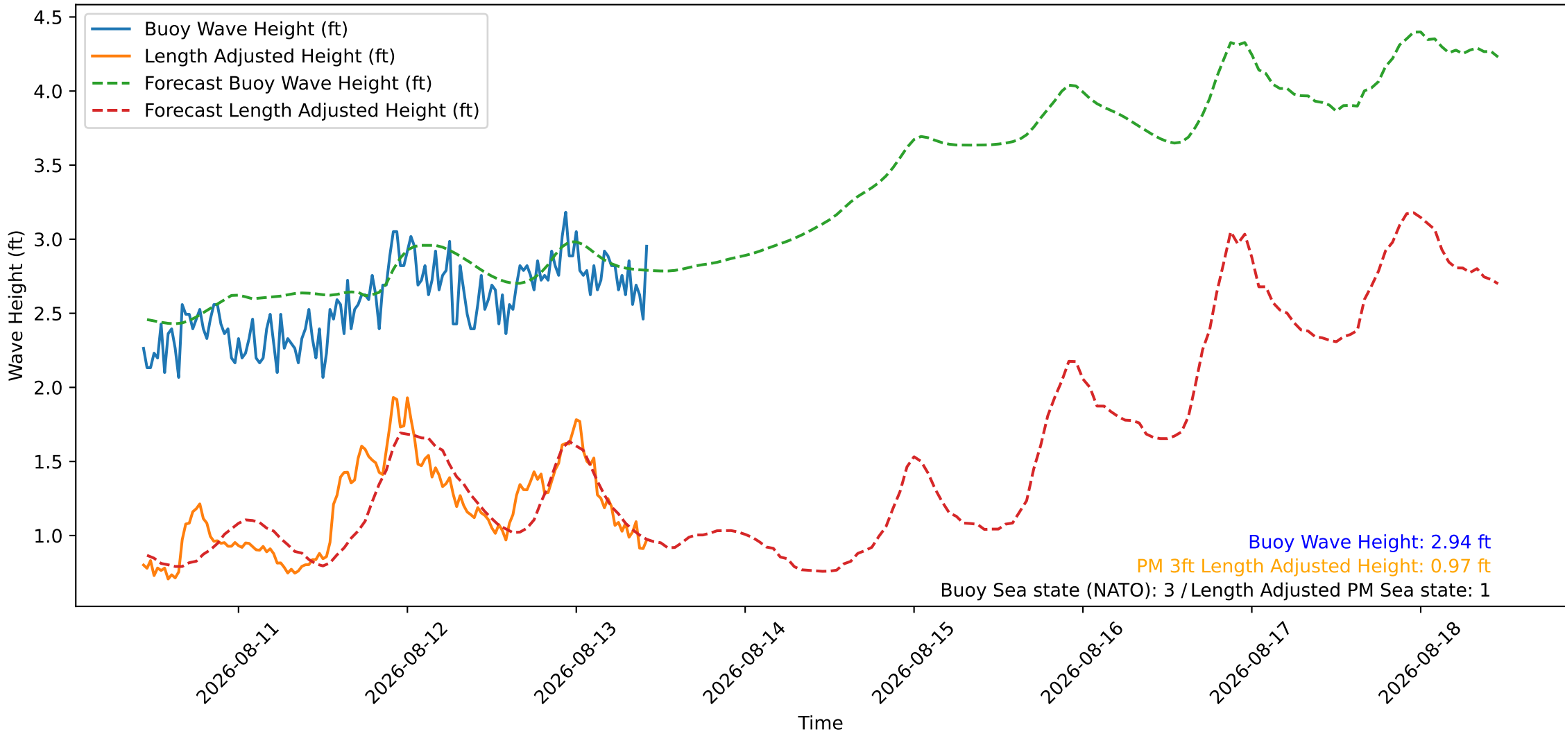
Wave Heights over Time for Oceanside Harbor at 2026-08-13 10:40:26
