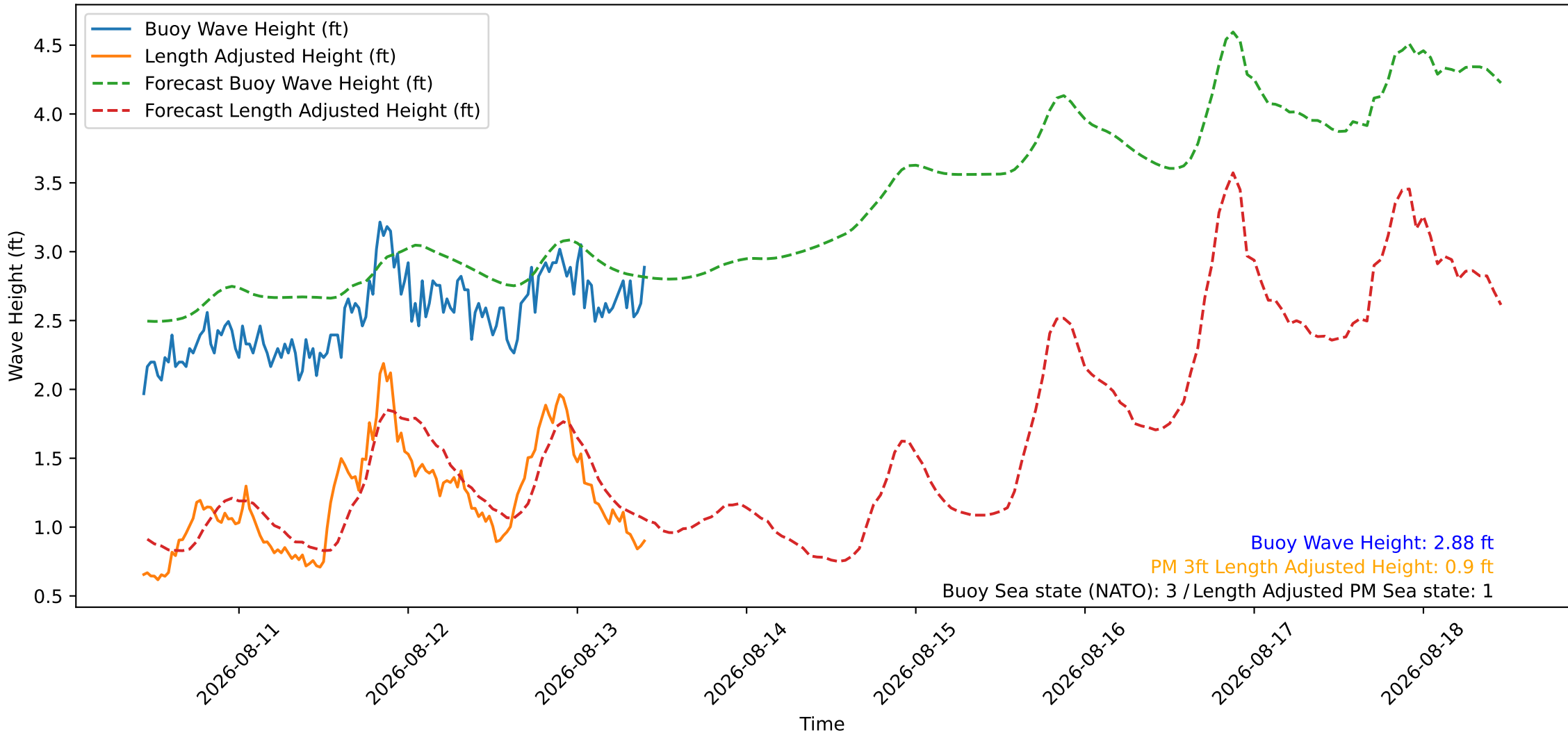
Wave Heights over Time for Green Beach at 2026-08-13 10:41:09
