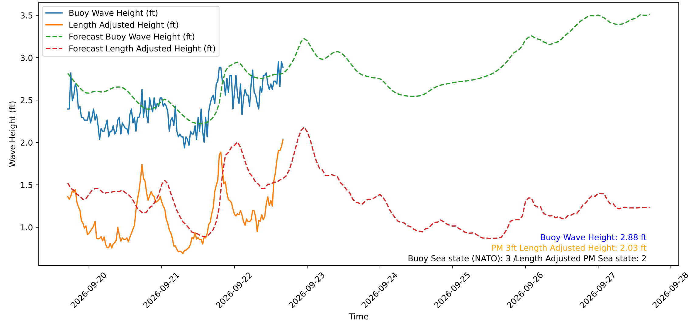
Wave Heights over Time for Red Beach at 2026-09-22 16:40:50
