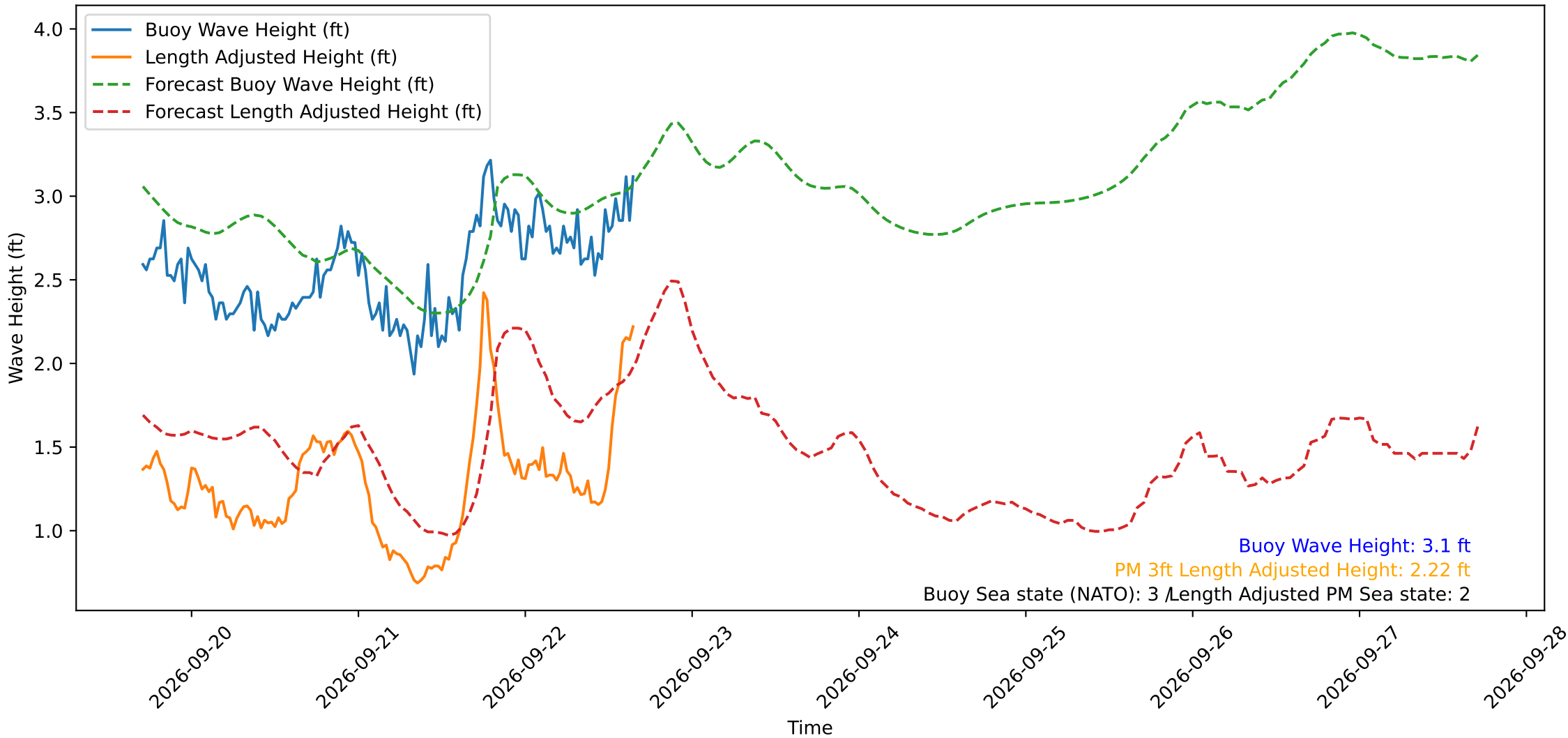
Wave Heights over Time for Green Beach at 2026-09-22 16:41:12
