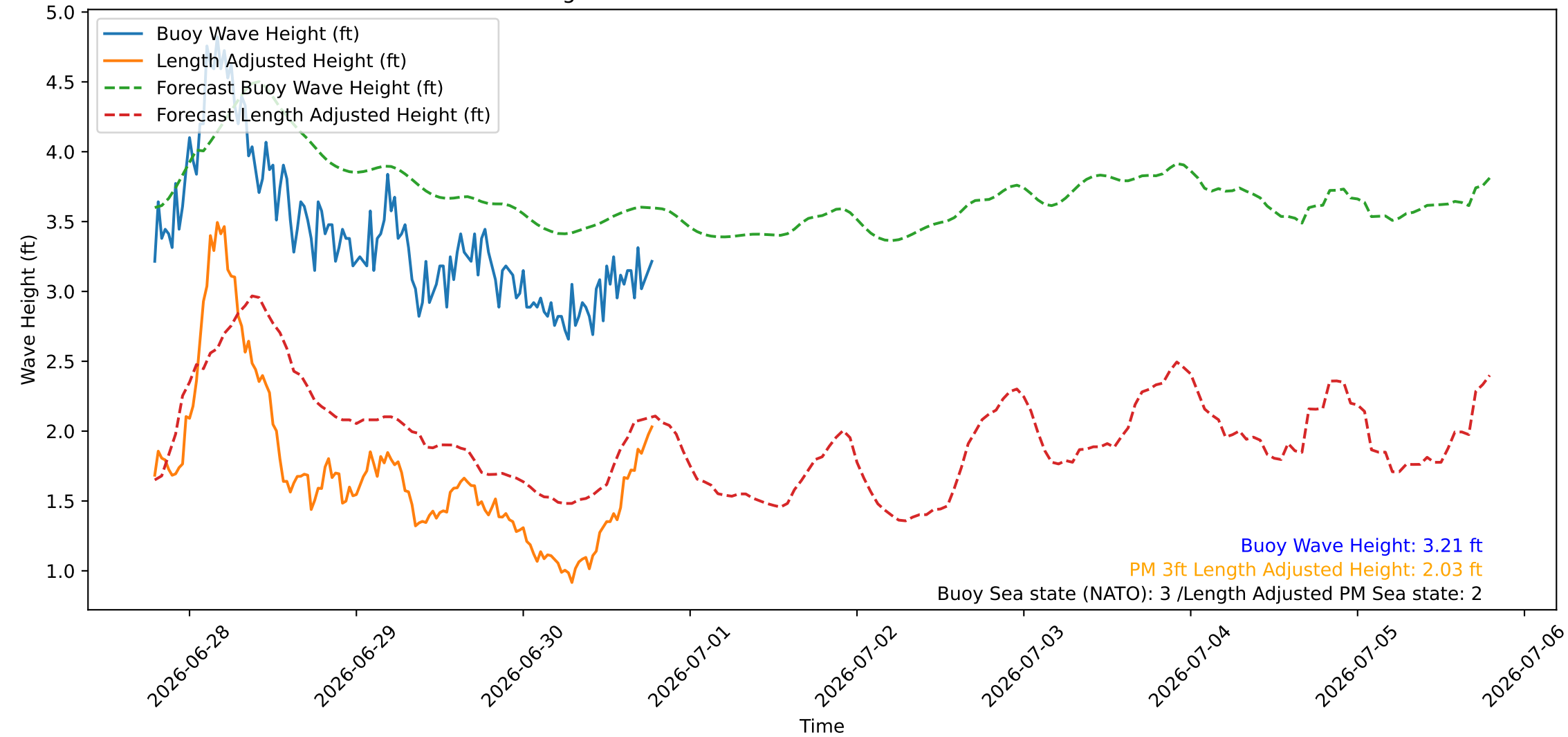
Wave Heights over Time for Green Beach at 2026-06-30 19:11:08
