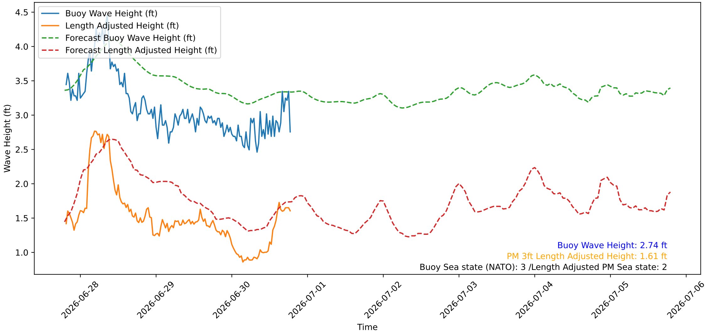
Wave Heights over Time for Red Beach at 2026-06-30 19:10:46
