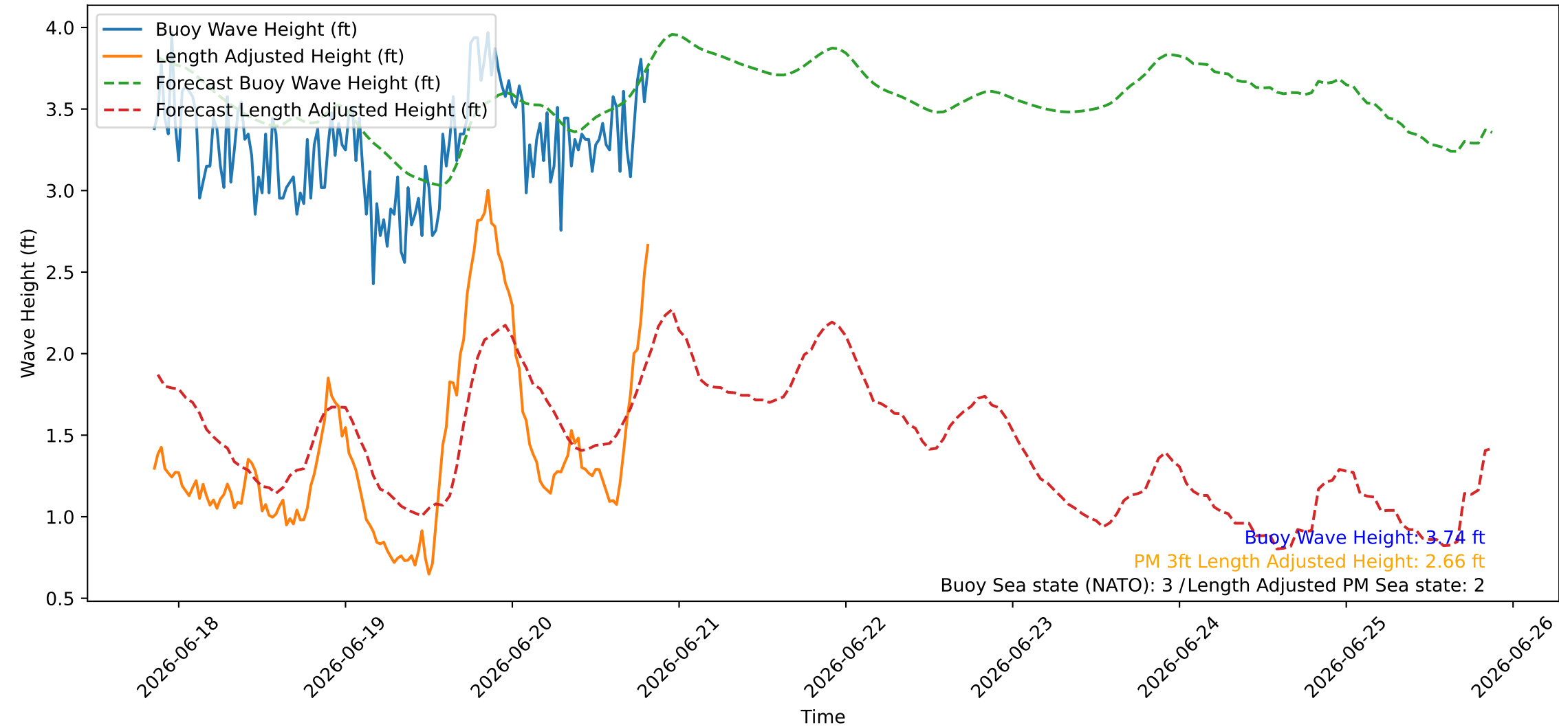
Wave Heights over Time for Green Beach at 2026-06-20 20:31:07
