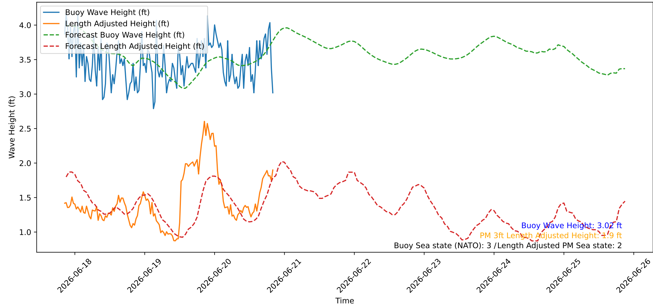
Wave Heights over Time for Oceanside Harbor at 2026-06-20 20:30:25
