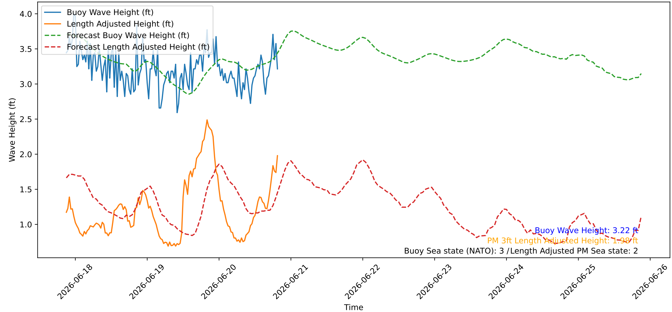
Wave Heights over Time for Red Beach at 2026-06-20 20:30:45
