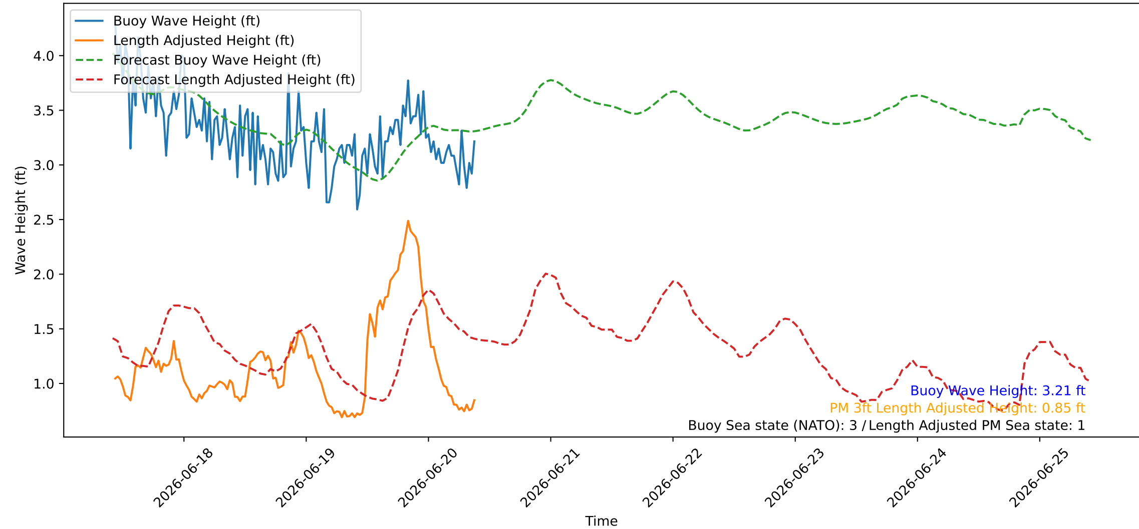
Wave Heights over Time for Red Beach at 2026-06-20 10:00:45
