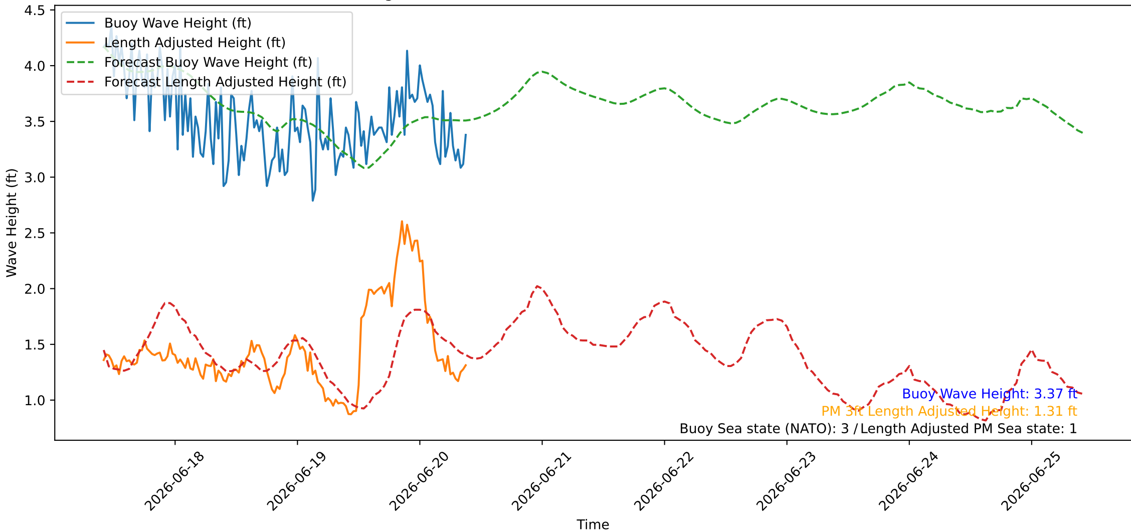
Wave Heights over Time for Oceanside Harbor at 2026-06-20 10:00:26
