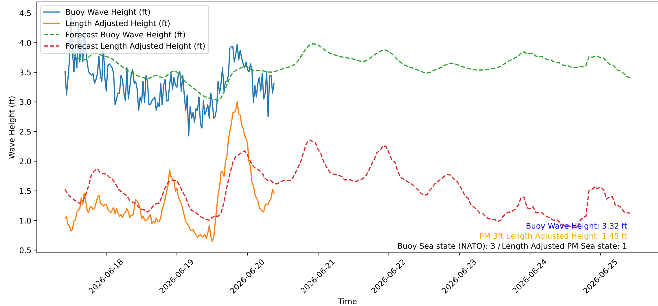
Wave Heights over Time for Green Beach at 2026-06-20 10:01:07
