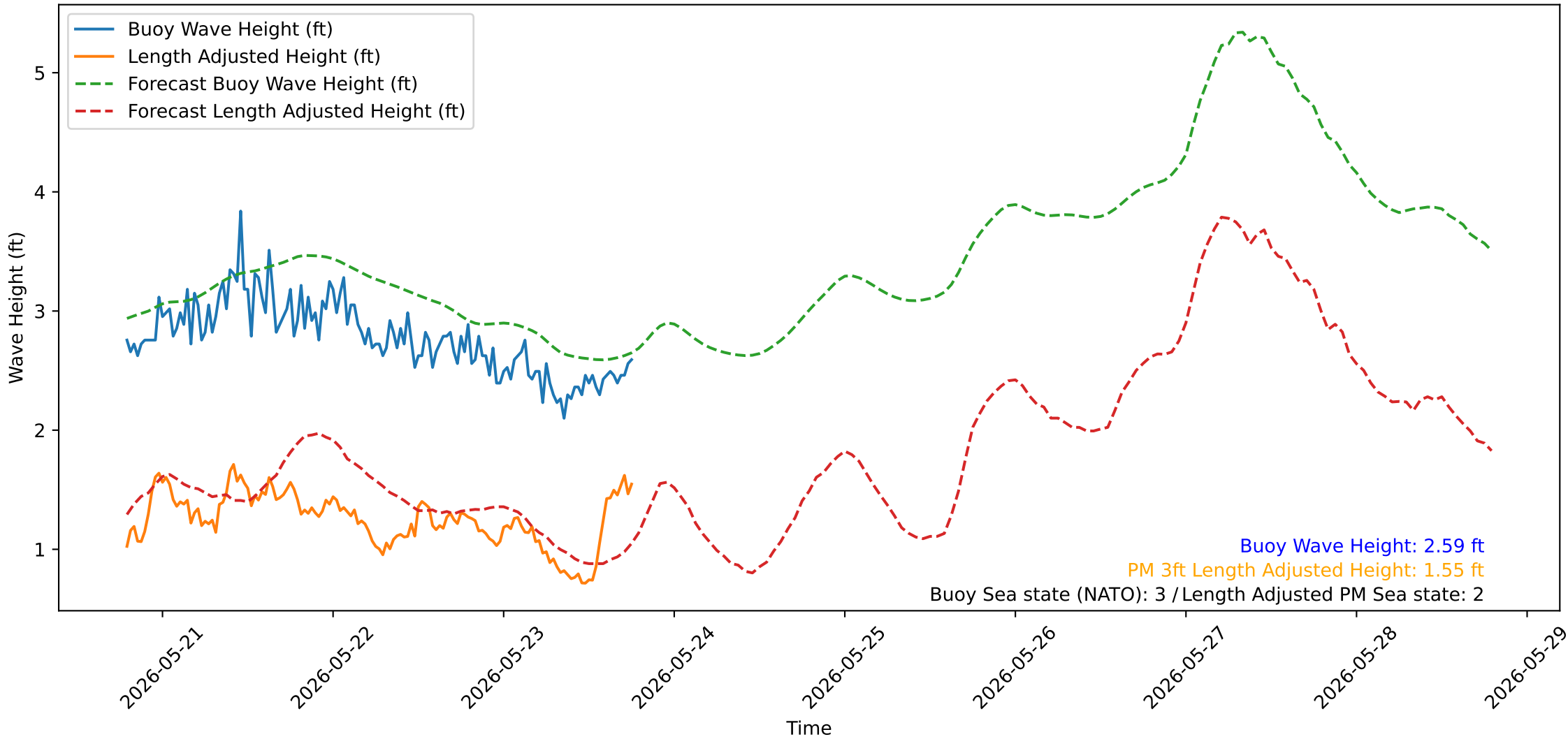
Wave Heights over Time for Oceanside Harbor at 2026-05-23 18:50:32
