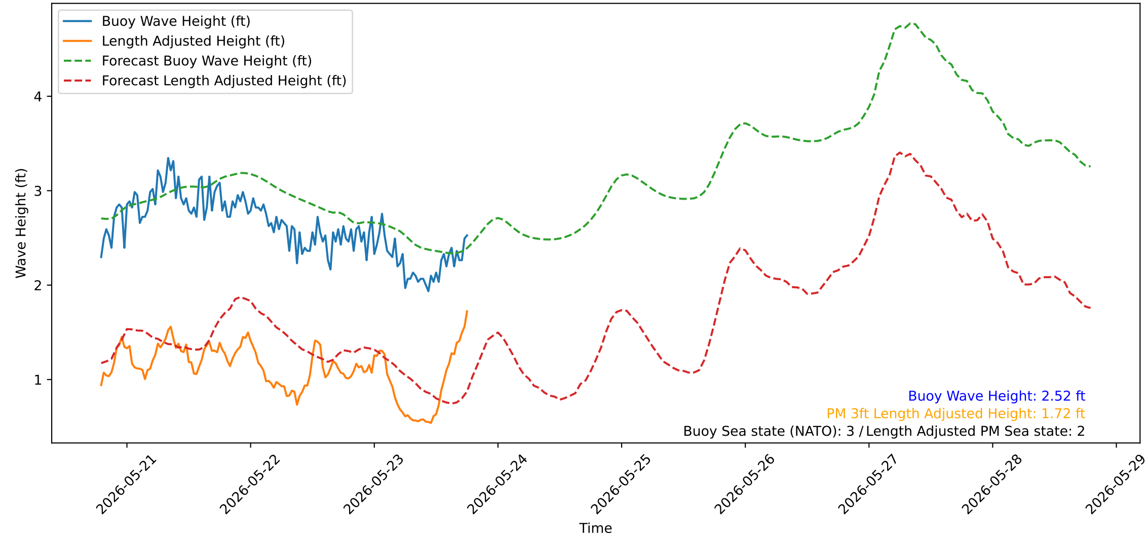
Wave Heights over Time for Red Beach at 2026-05-23 18:50:53
