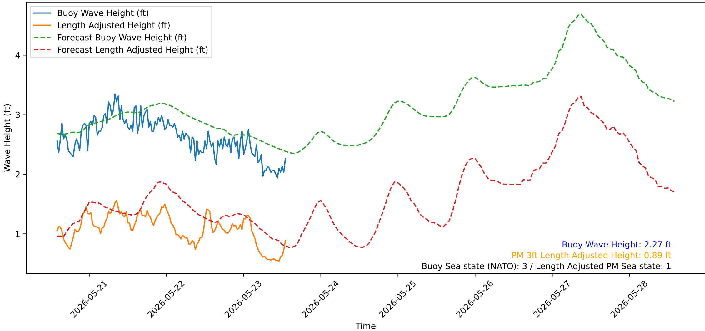
Wave Heights over Time for Red Beach at 2026-05-23 13:40:51
