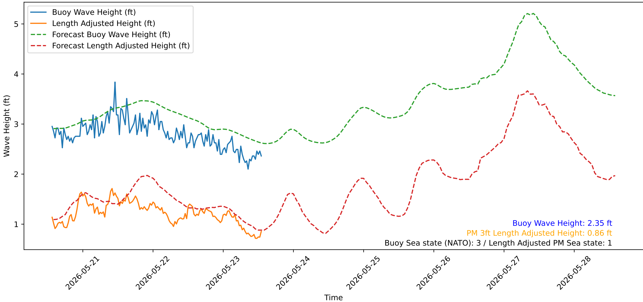
Wave Heights over Time for Oceanside Harbor at 2026-05-23 13:40:32
