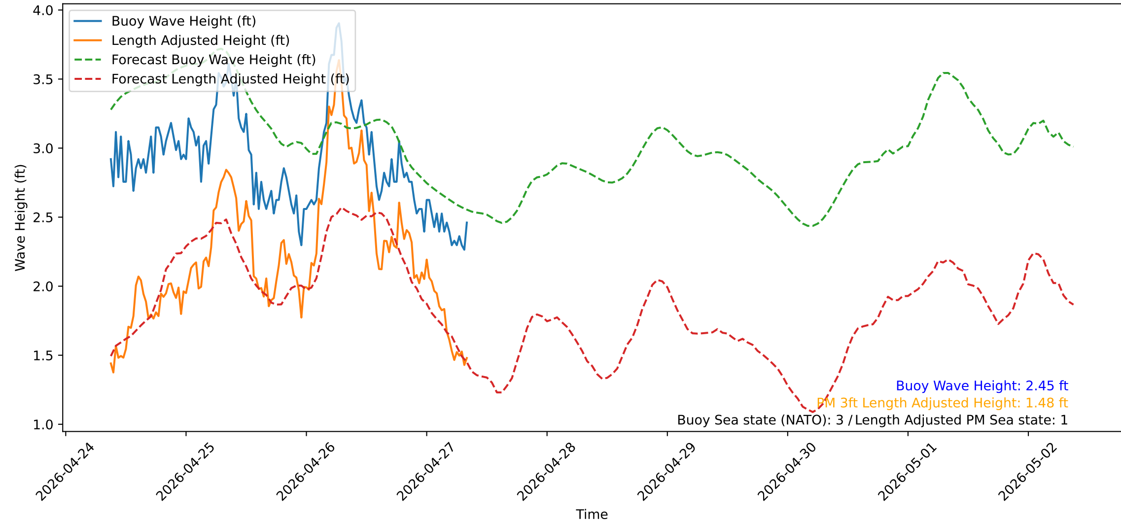
Wave Heights over Time for Oceanside Harbor at 2026-04-27 09:00:31
