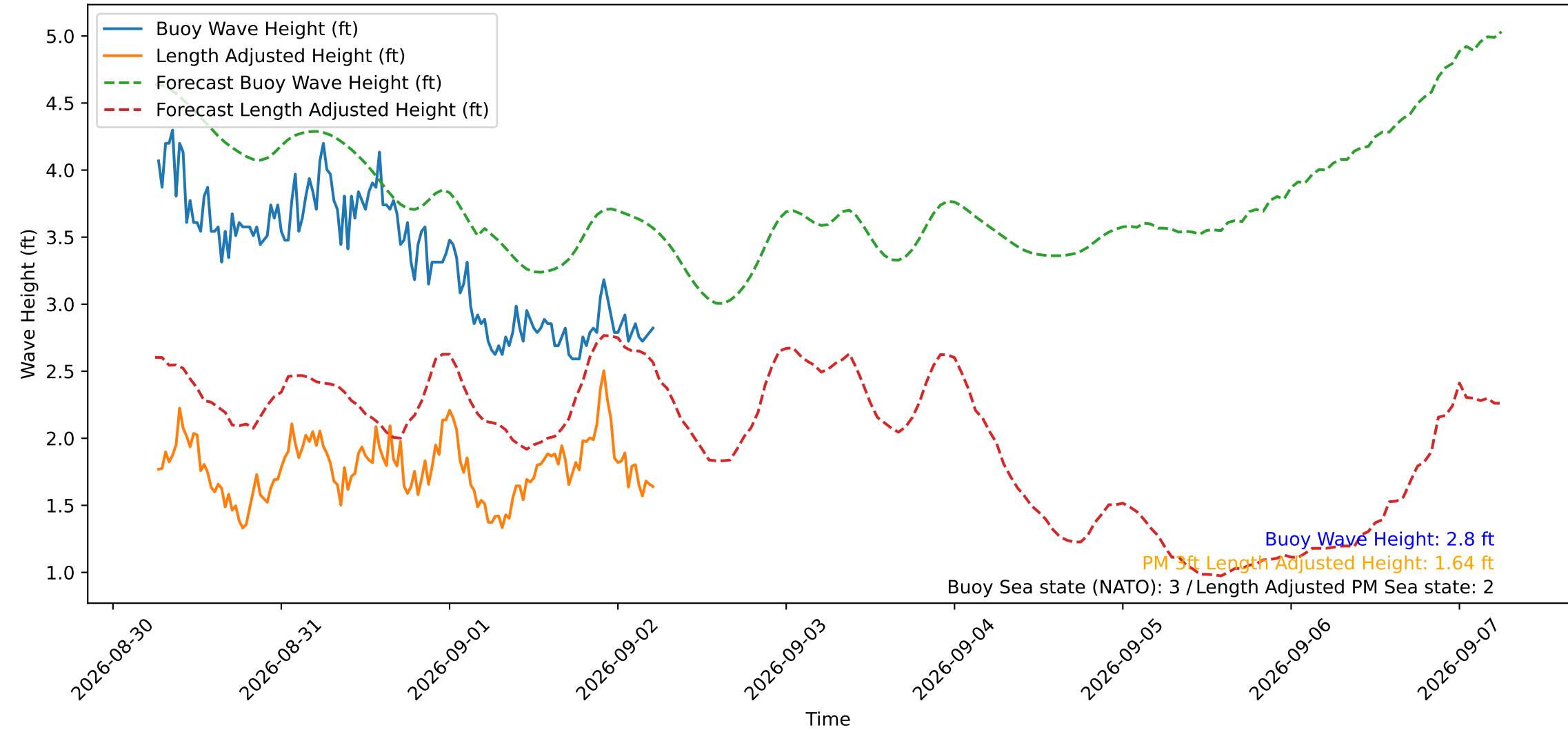
Wave Heights over Time for Red Beach at 2026-09-02 06:00:49
