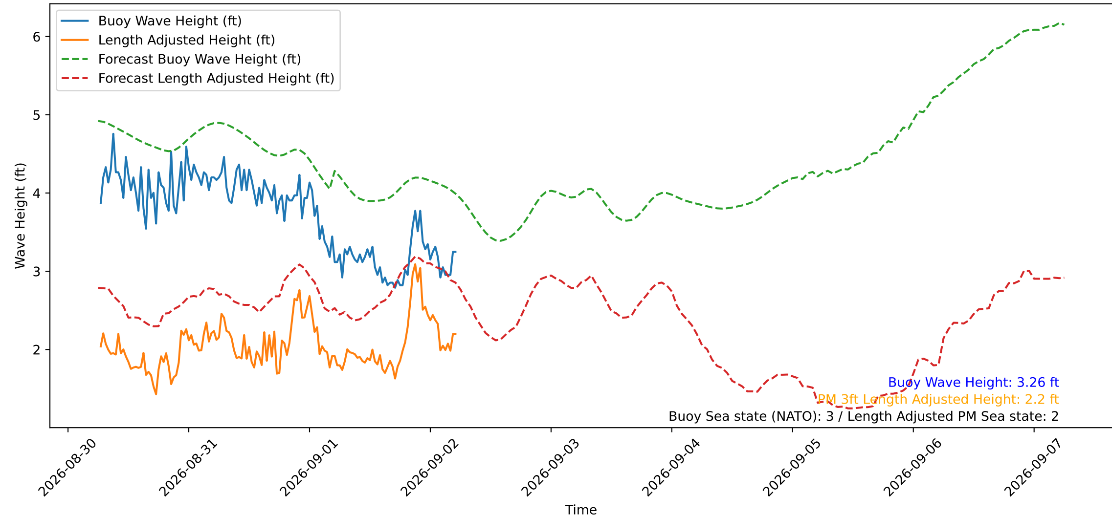
Wave Heights over Time for Green Beach at 2026-09-02 06:01:12
