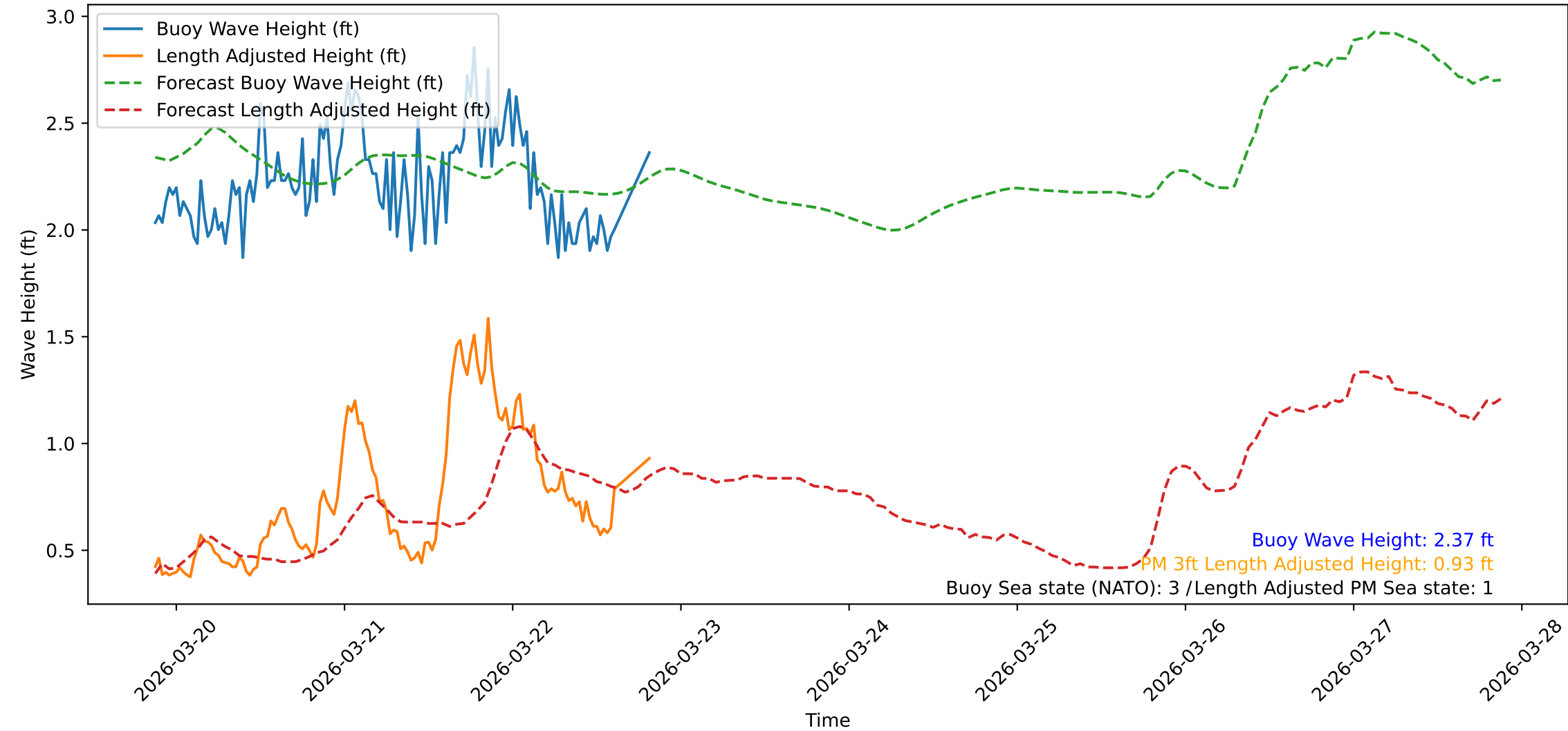
Wave Heights over Time for Red Beach at 2026-03-22 20:30:49
