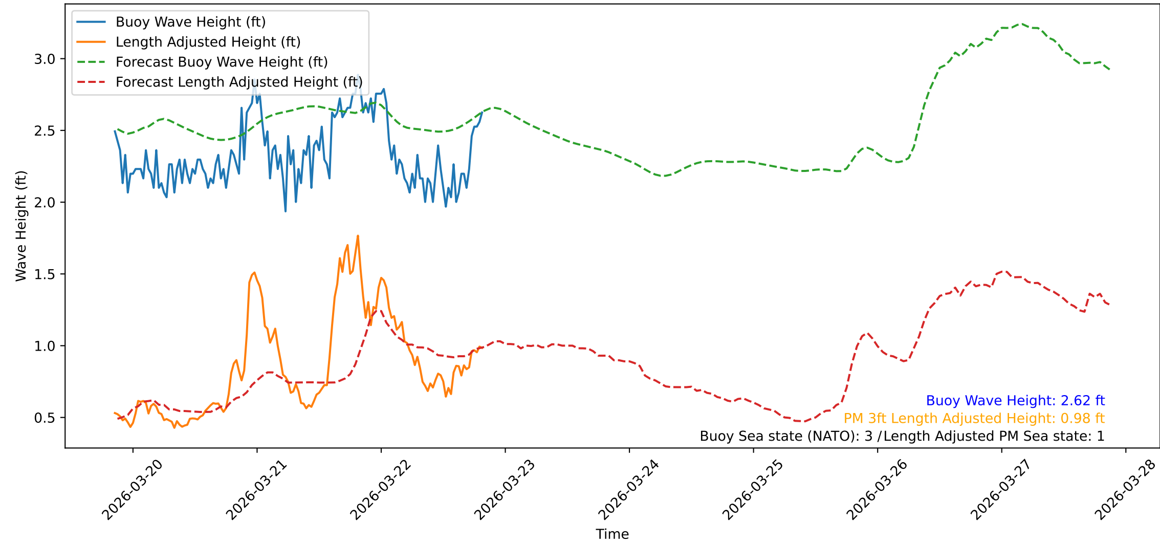
Wave Heights over Time for Green Beach at 2026-03-22 20:31:11
