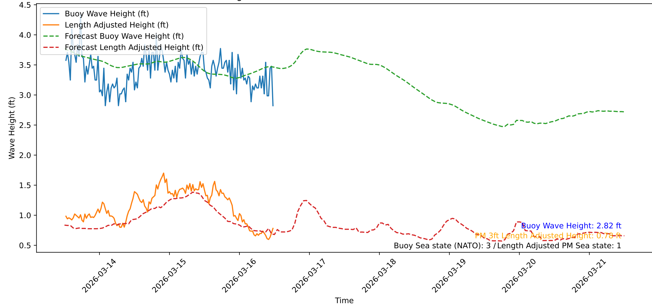
Wave Heights over Time for Green Beach at 2026-03-16 12:21:43
