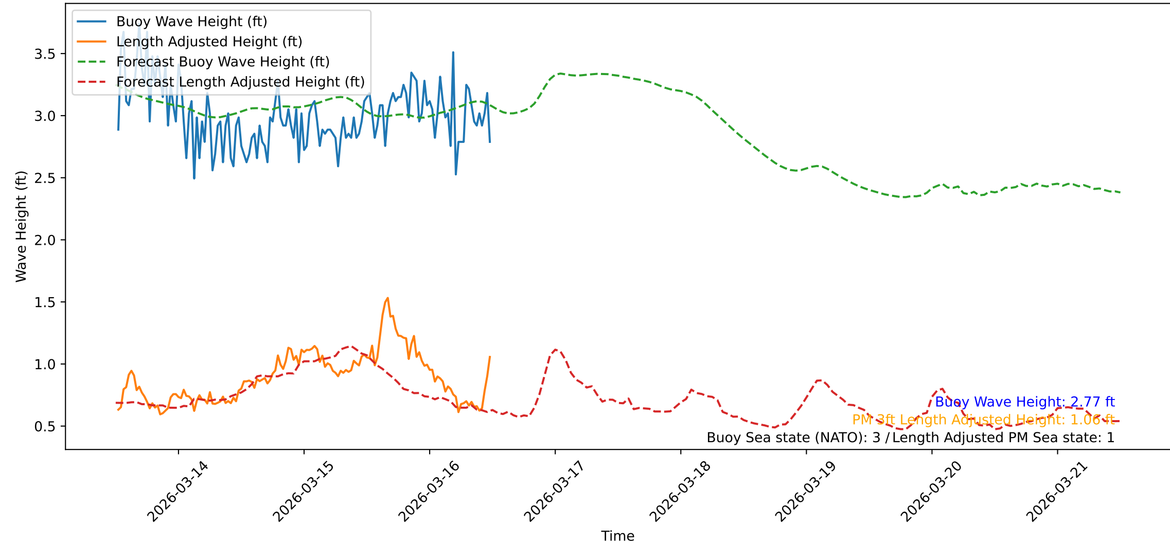
Wave Heights over Time for Red Beach at 2026-03-16 12:21:06
