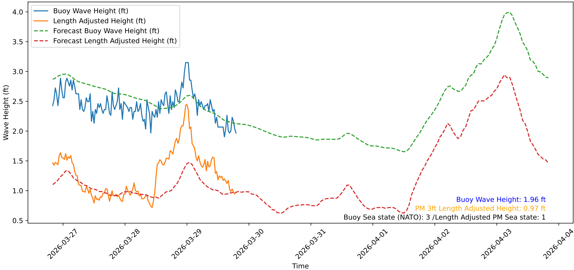
Wave Heights over Time for Oceanside Harbor at 2026-03-29 19:50:31
