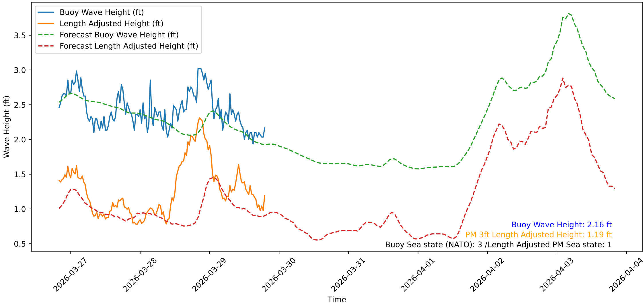
Wave Heights over Time for Red Beach at 2026-03-29 19:50:47
