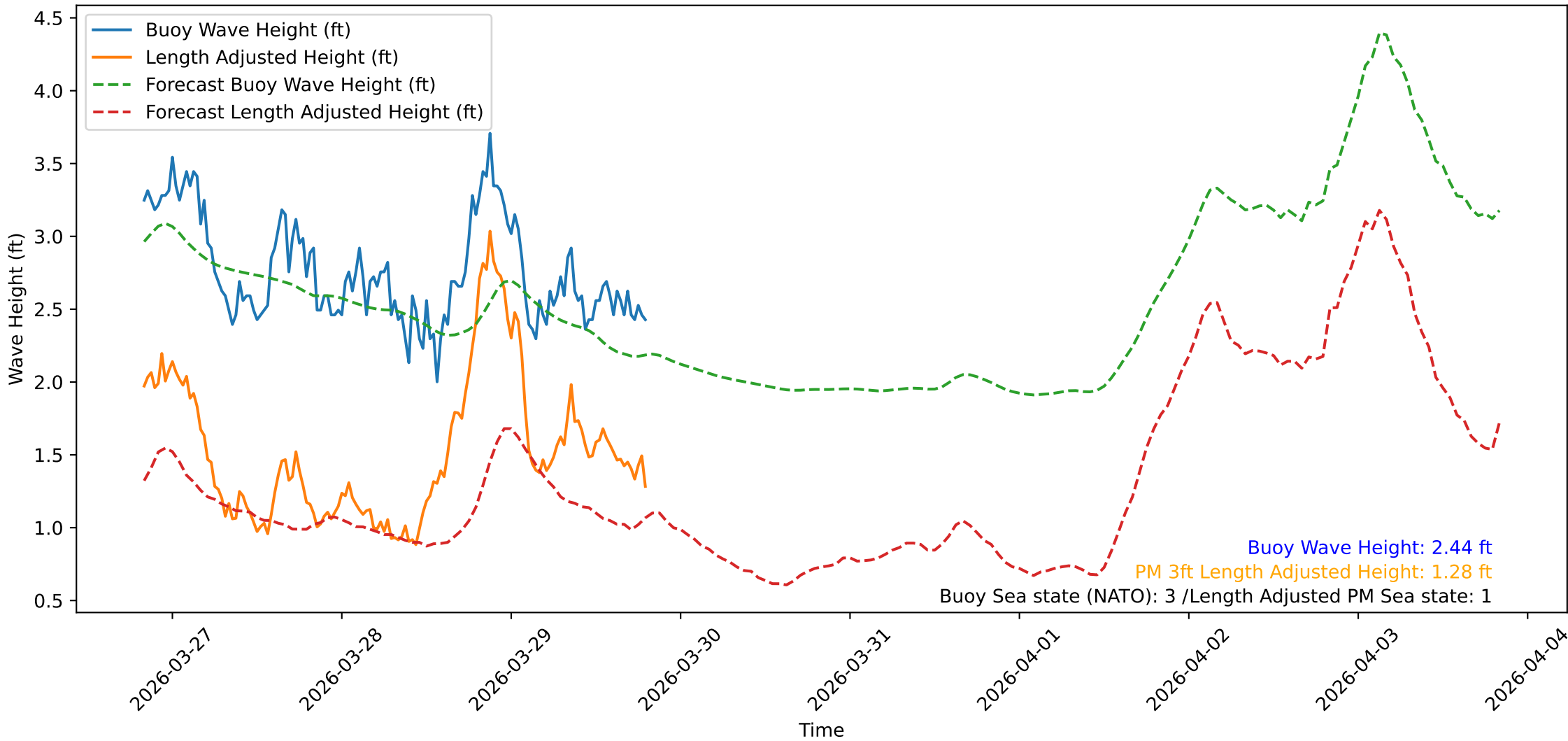
Wave Heights over Time for Green Beach at 2026-03-29 19:51:09
