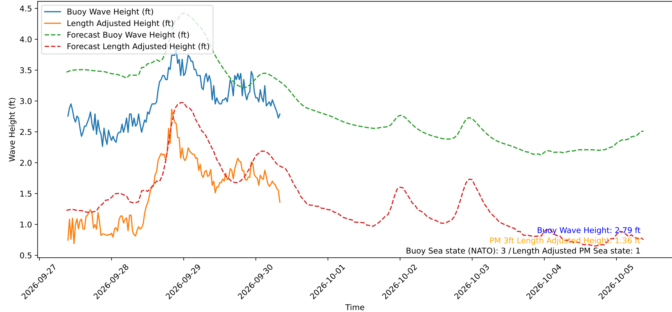
Wave Heights over Time for Red Beach at 2026-09-30 09:00:50
