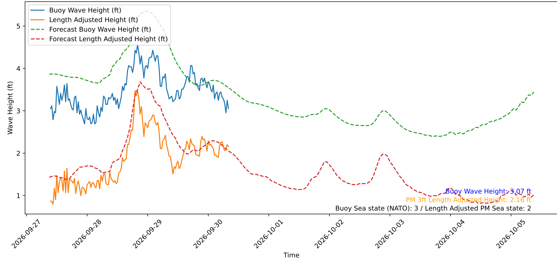
Wave Heights over Time for Green Beach at 2026-09-30 09:01:12
