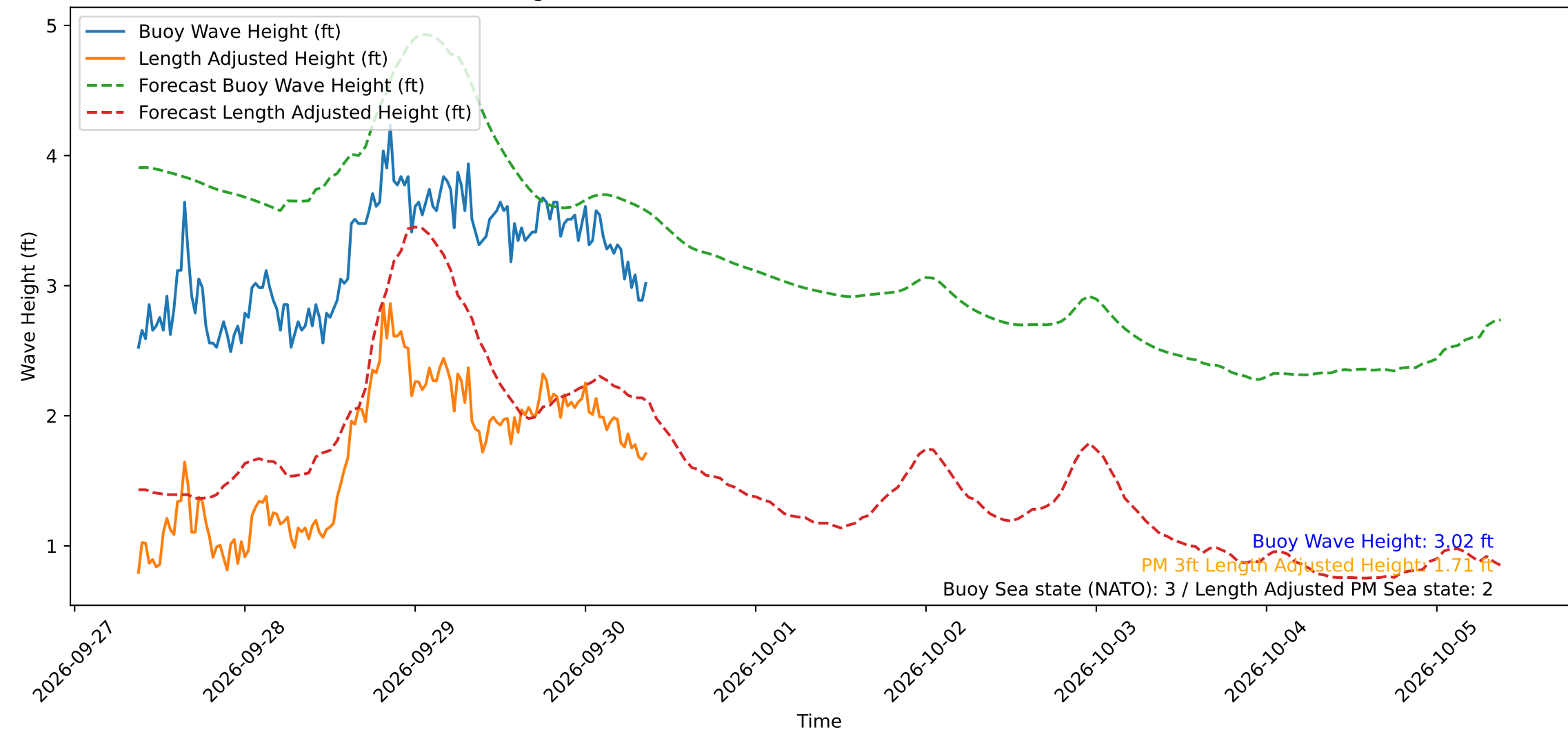
Wave Heights over Time for Oceanside Harbor at 2026-09-30 09:00:30
