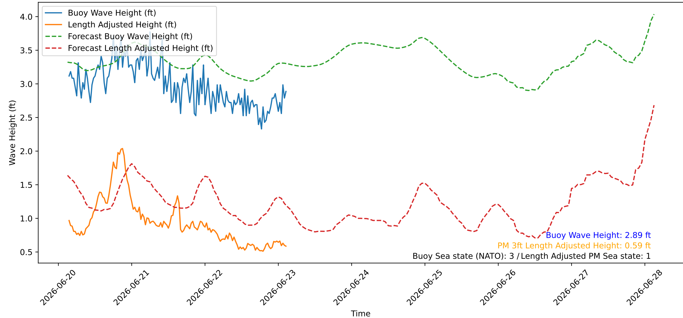
Wave Heights over Time for Red Beach at 2026-06-23 03:10:45
