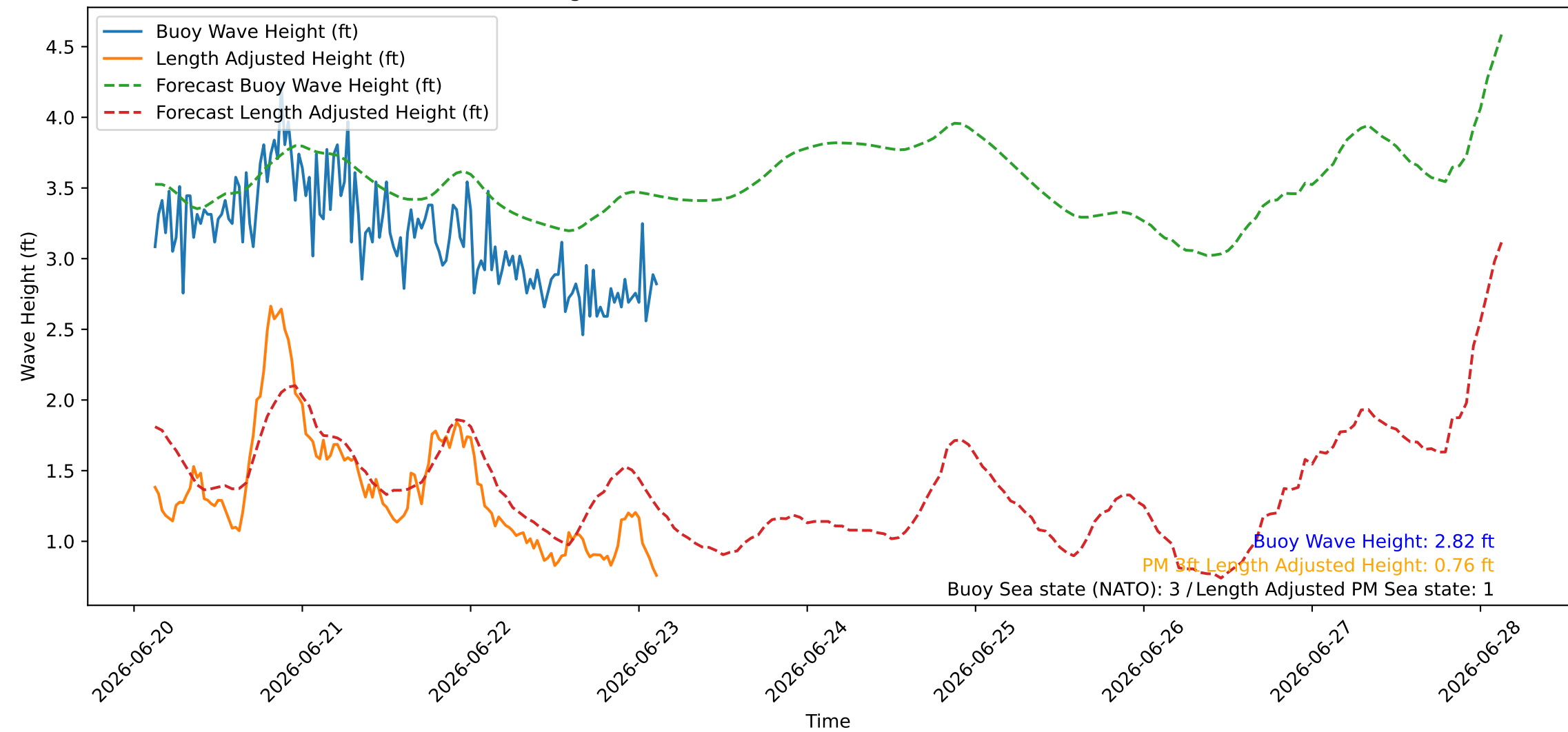
Wave Heights over Time for Green Beach at 2026-06-23 03:11:08
