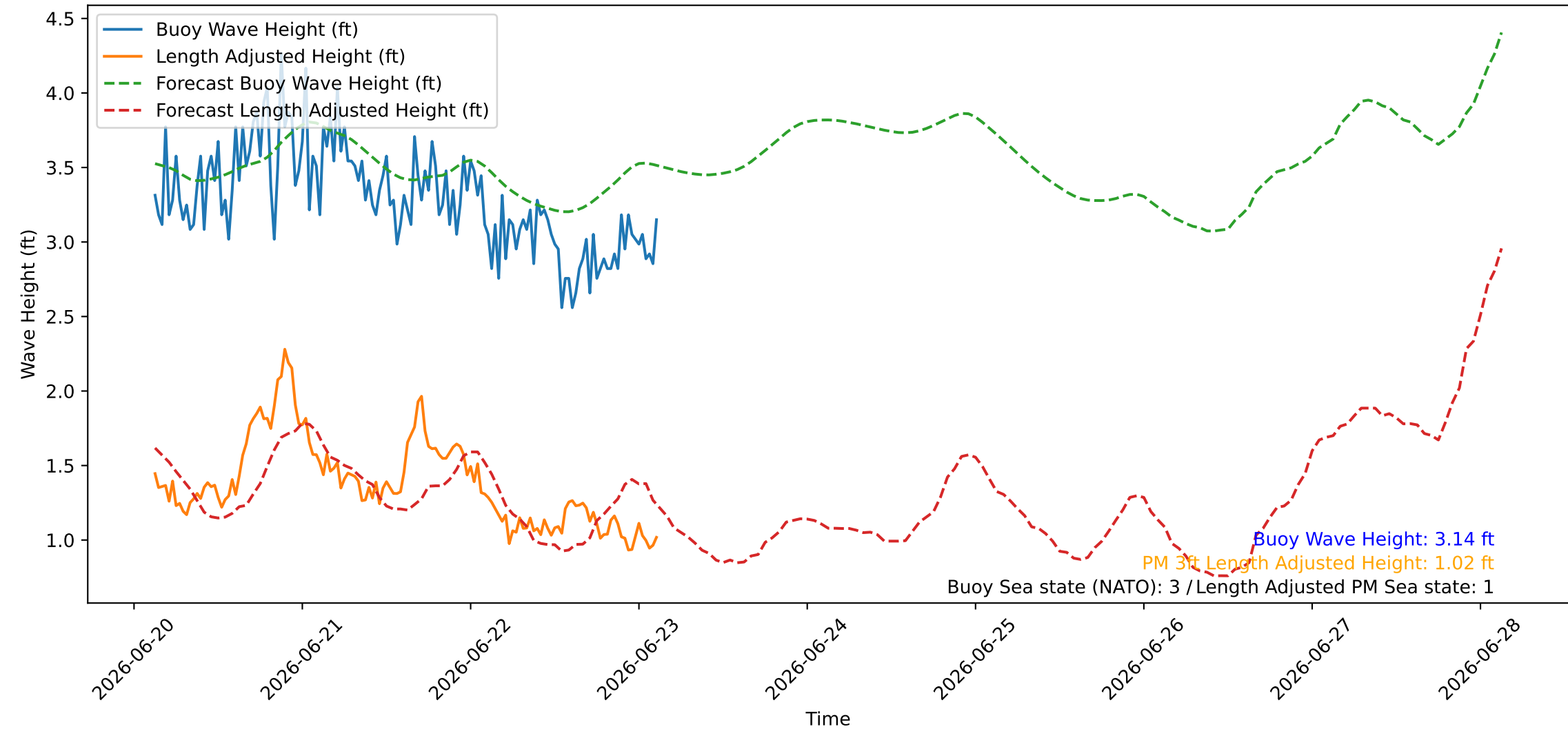
Wave Heights over Time for Oceanside Harbor at 2026-06-23 03:10:26
