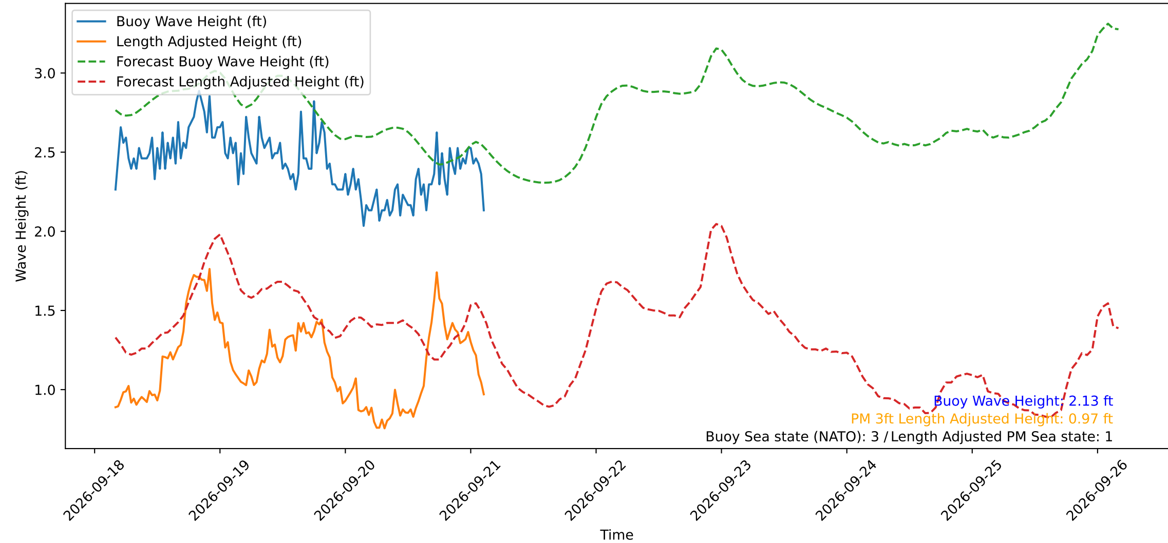
Wave Heights over Time for Red Beach at 2026-09-21 03:30:50
