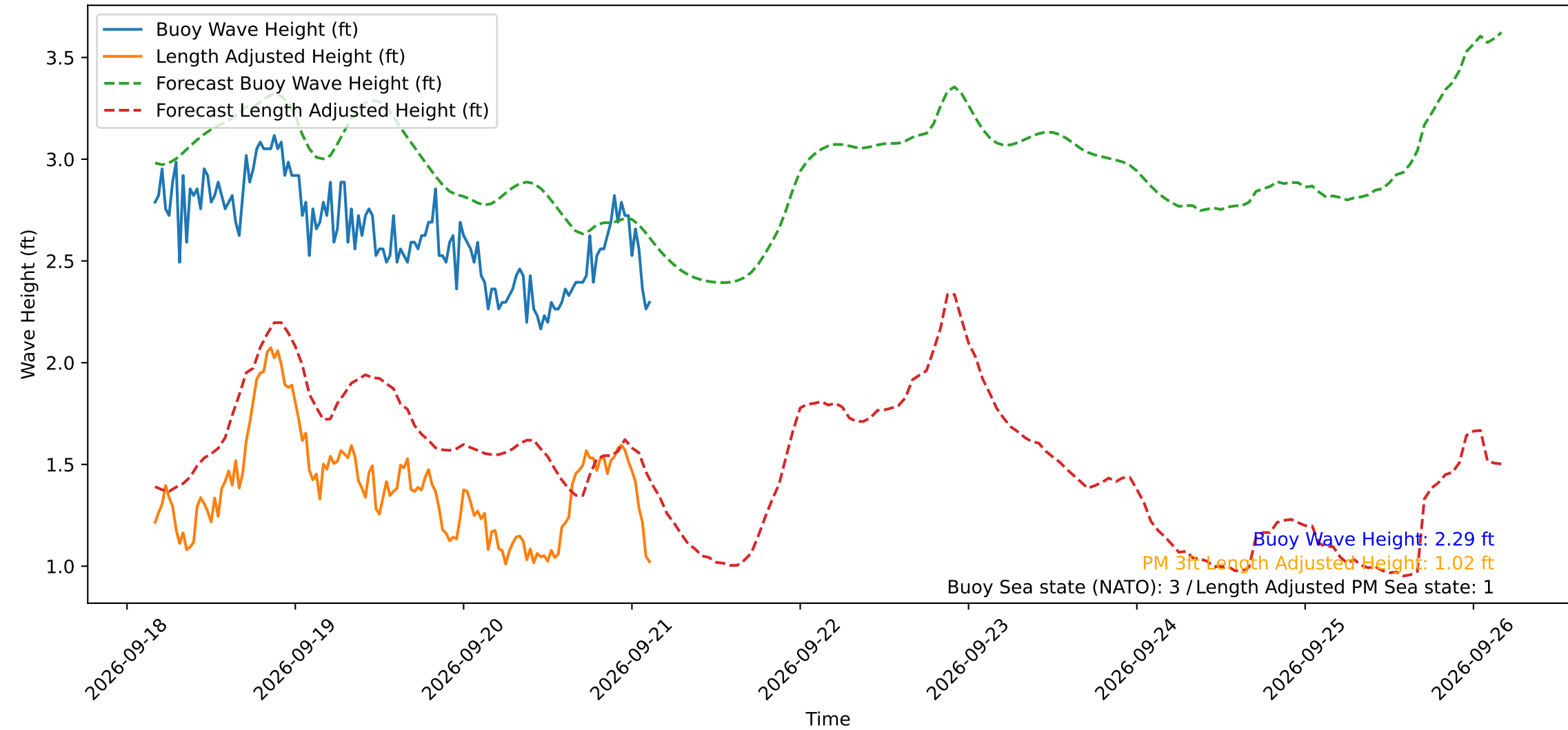
Wave Heights over Time for Green Beach at 2026-09-21 03:31:12
