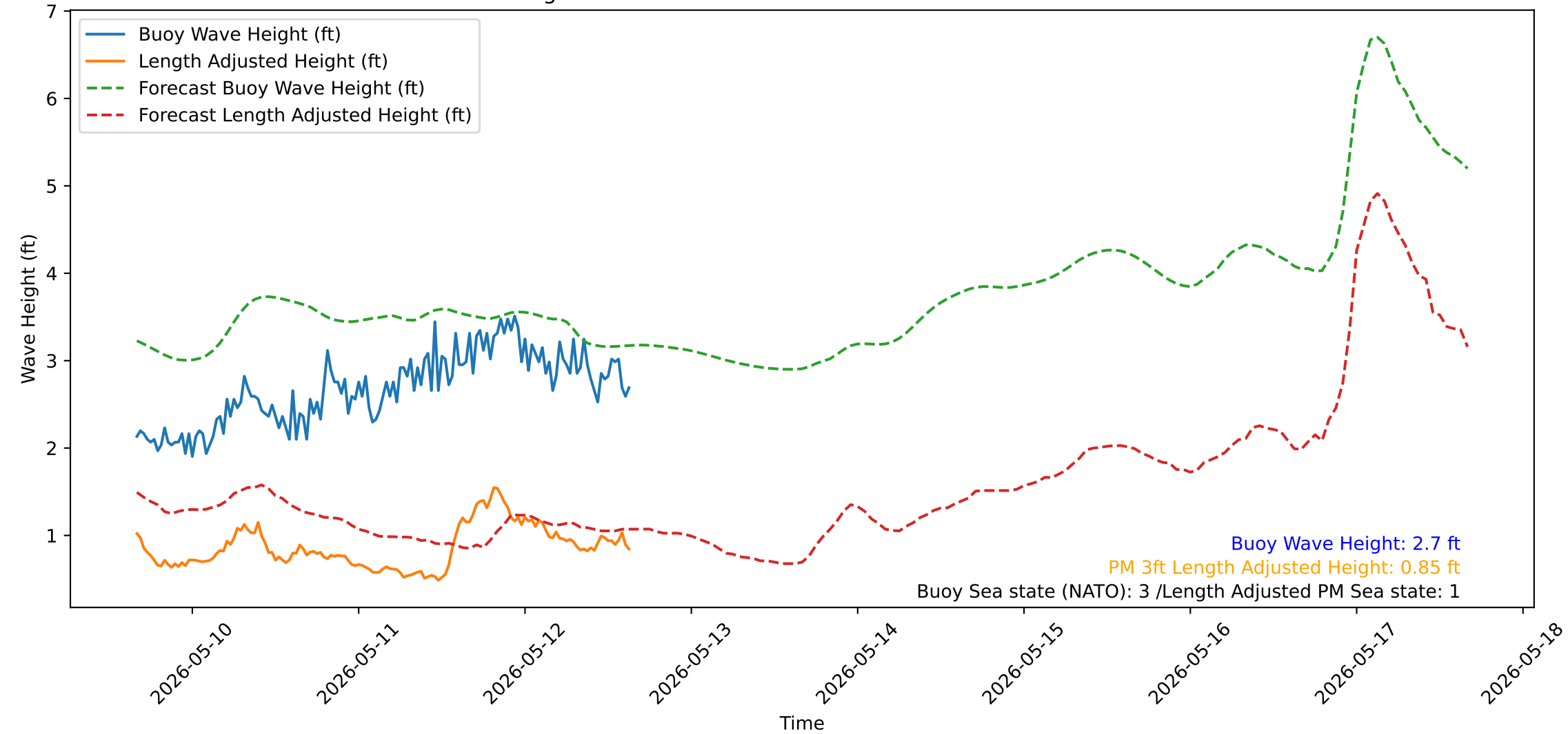
Wave Heights over Time for Green Beach at 2026-05-12 15:51:15
