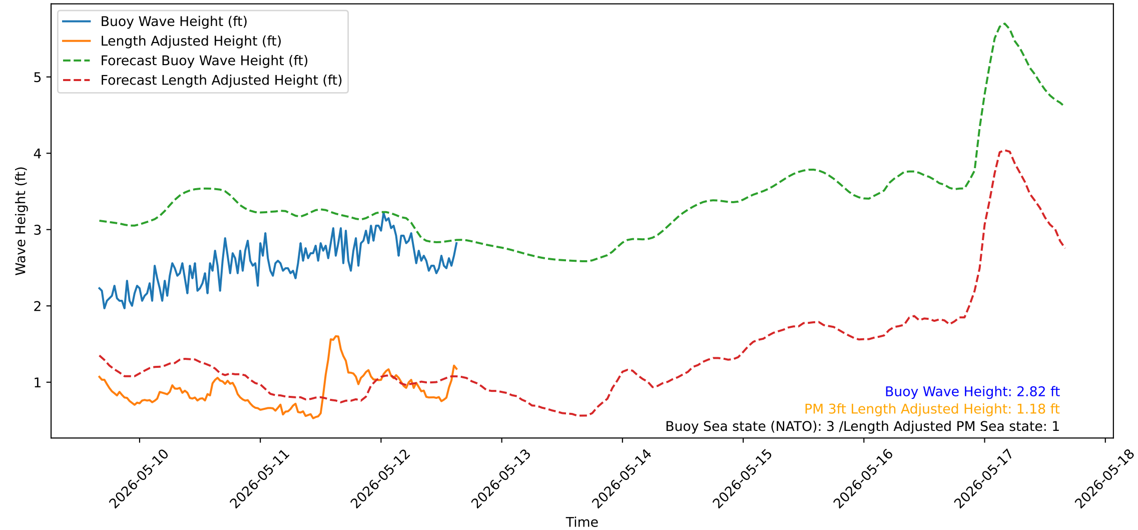
Wave Heights over Time for Red Beach at 2026-05-12 15:50:53
