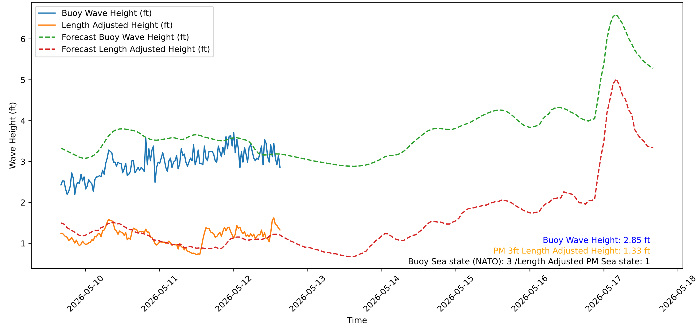
Wave Heights over Time for Oceanside Harbor at 2026-05-12 15:50:33
