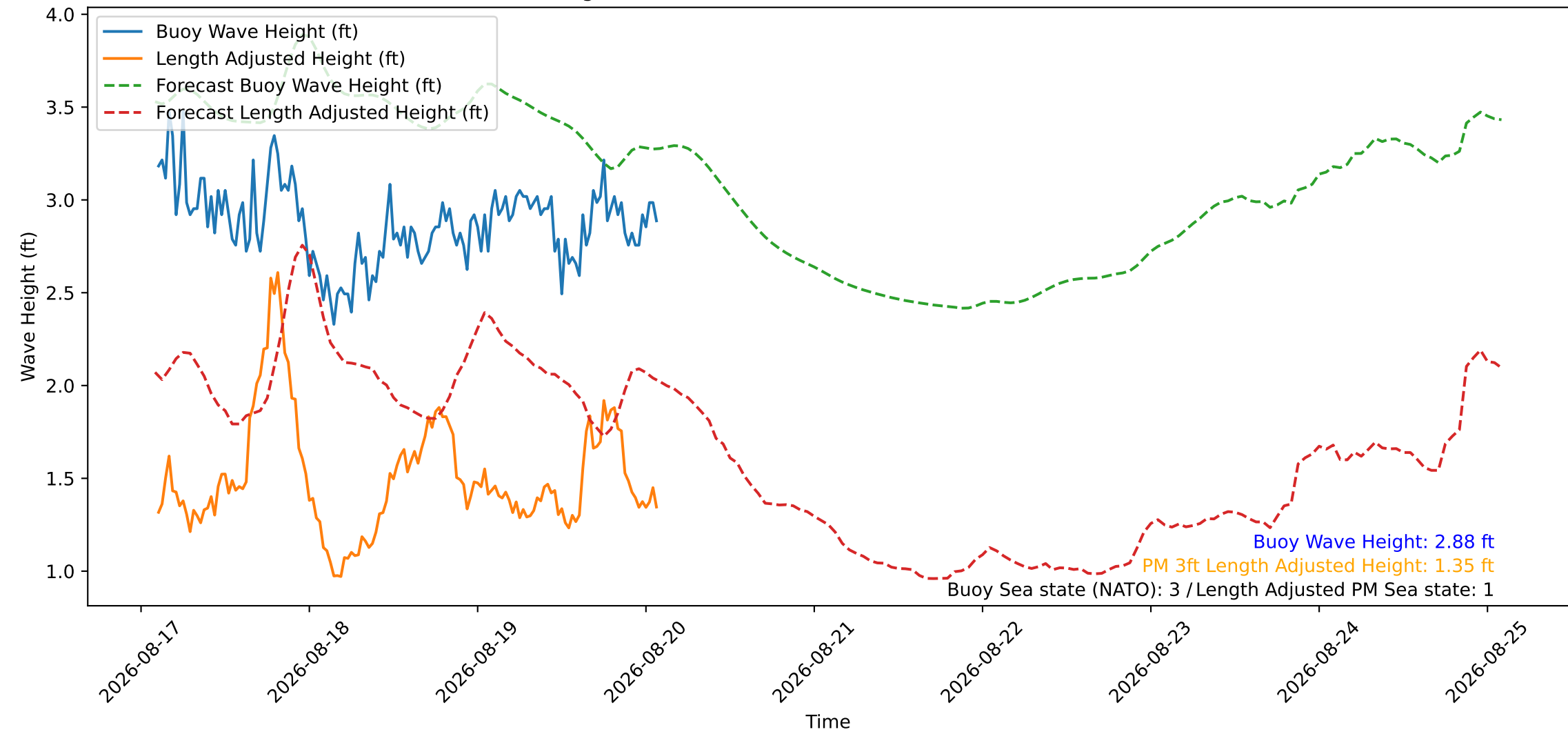
Wave Heights over Time for Red Beach at 2026-08-20 02:10:46
