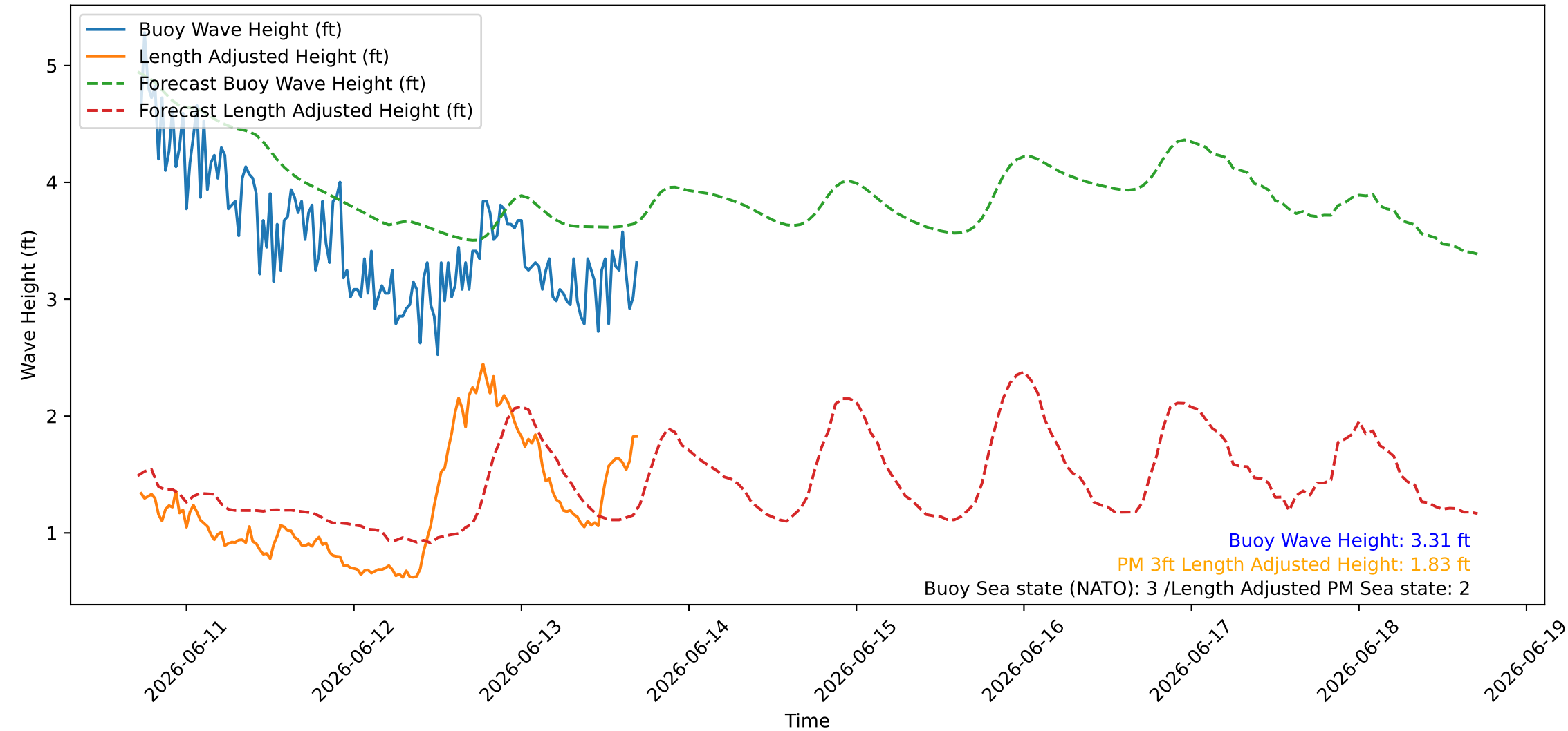
Wave Heights over Time for Red Beach at 2026-06-13 17:10:46
