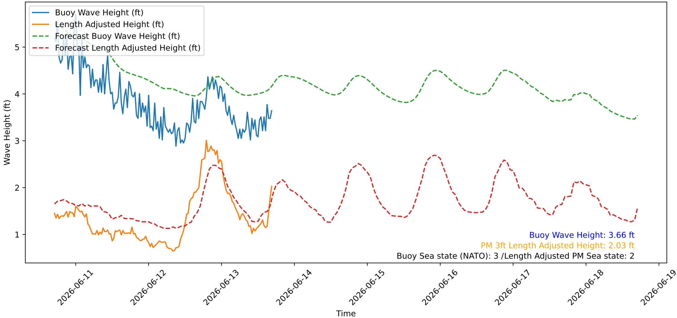
Wave Heights over Time for Green Beach at 2026-06-13 17:11:08
