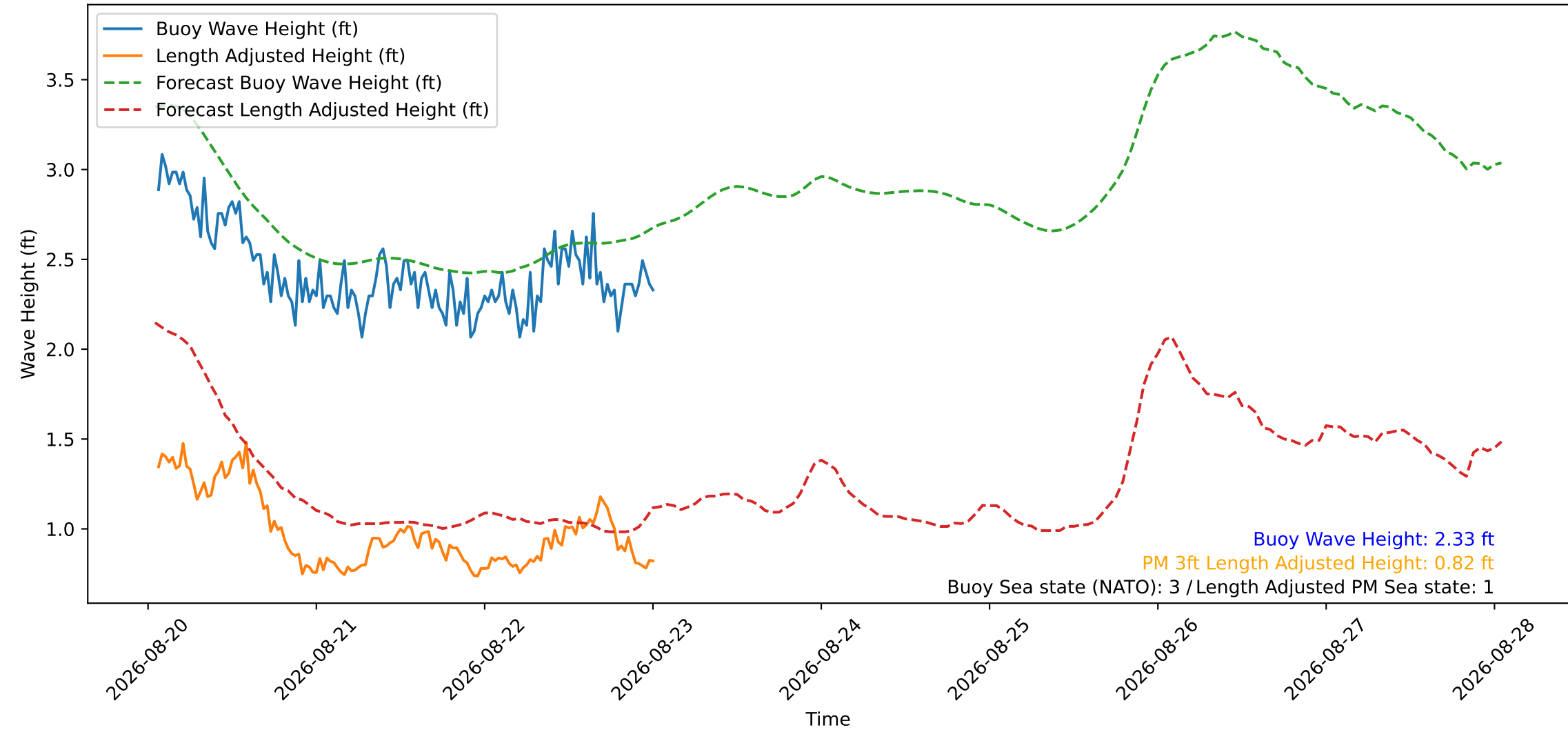
Wave Heights over Time for Red Beach at 2026-08-23 01:00:50
