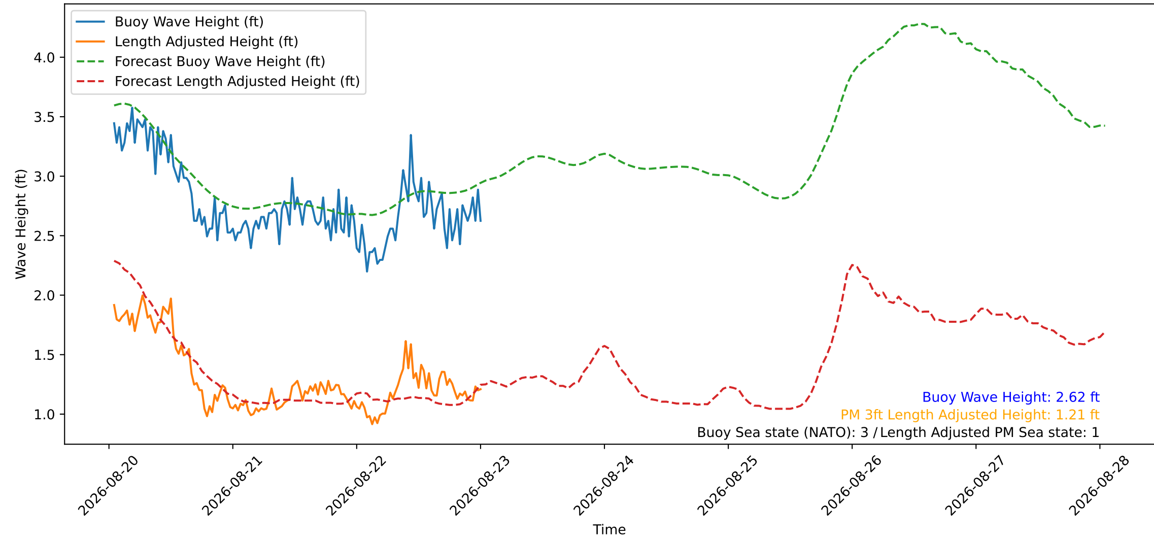
Wave Heights over Time for Oceanside Harbor at 2026-08-23 01:00:30
