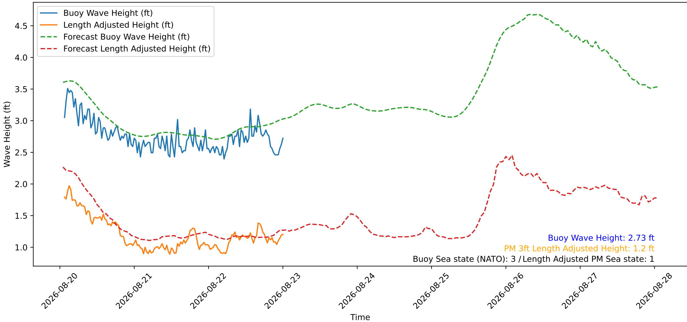
Wave Heights over Time for Green Beach at 2026-08-23 01:01:12
